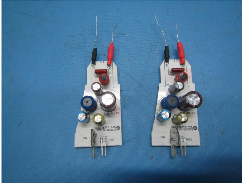
Driver PCB view (Left: for model WFD7102; Right: for models WFD7105 and WFD7107)
