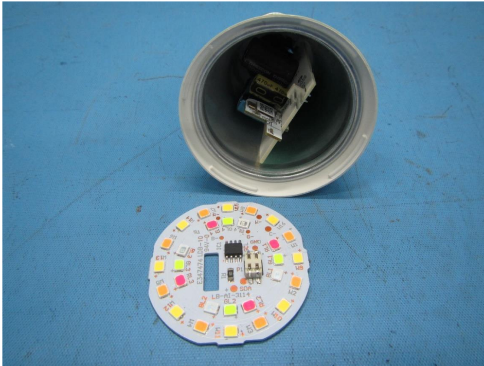
Internal view of model WFD7101 for representative
