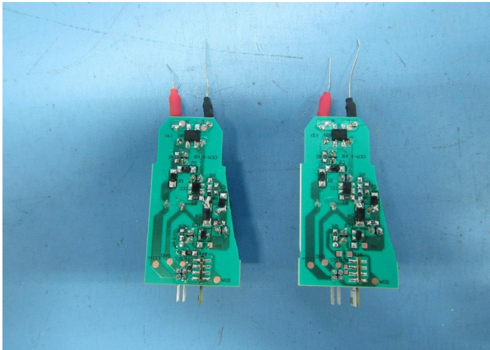
Driver PCB view (Left: for model WFD7102; Right: for models WFD7105 and WFD7107)
