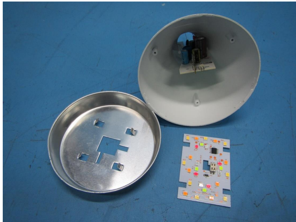
Internal view of model WFD7102 for representative
