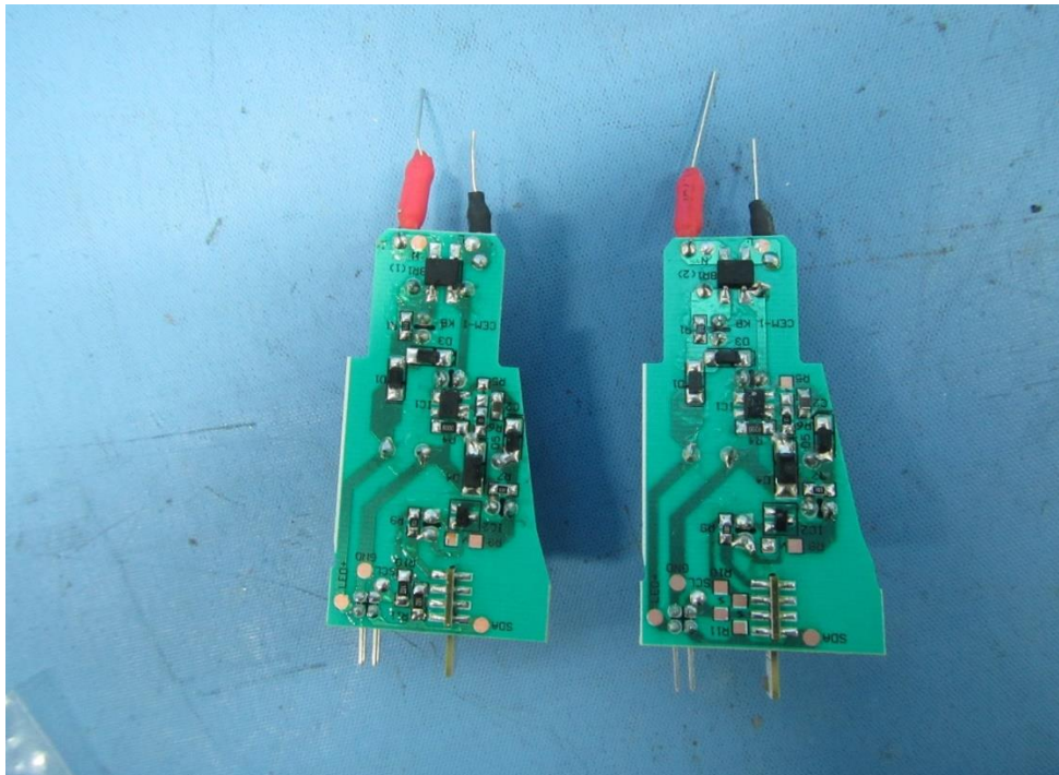
Driver PCB view (Left: for model WFD7101; Right: for models WFD7104 and WFD7106)
