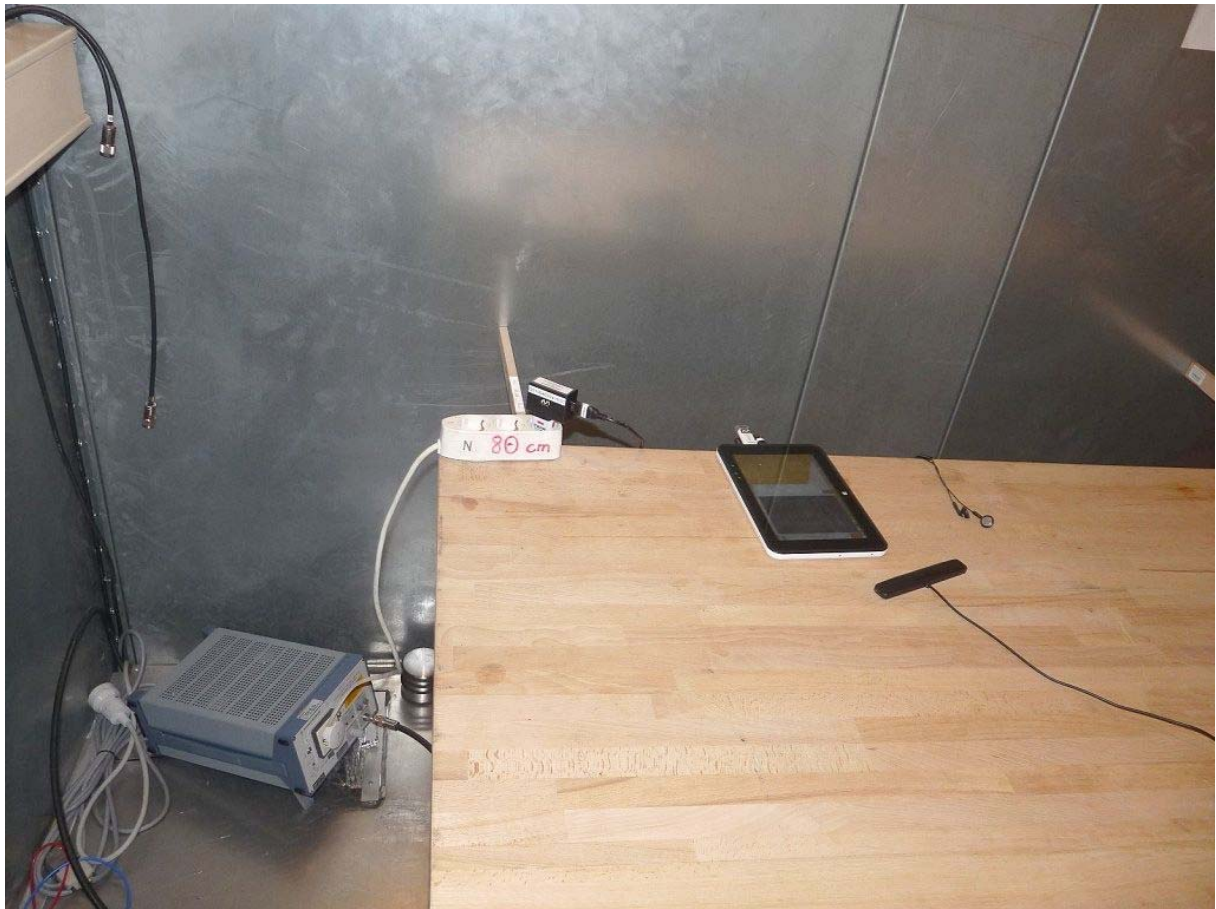
Photo 6: Test setup for conducted measurements (intentional radiator §15, AC Mains conducted emissions)
