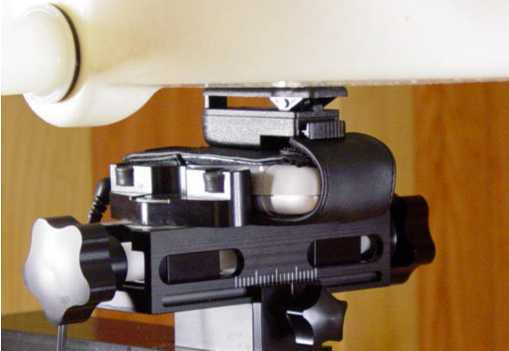
Figure 12.4 Body SAR Set-up (with standard case)
