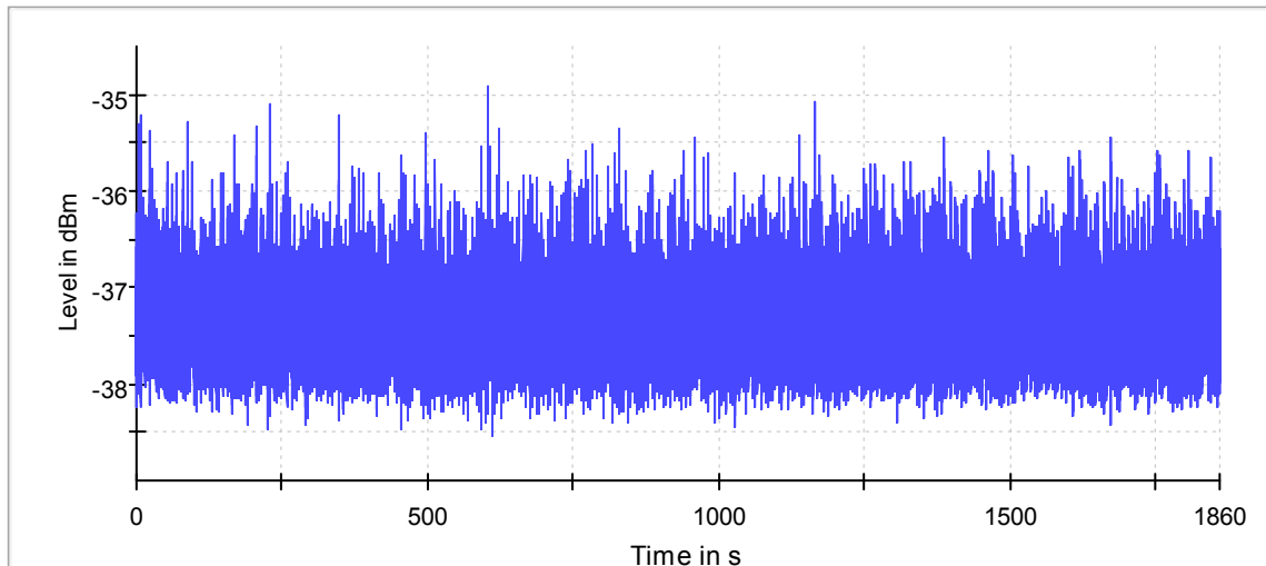
802.11ac (80 MHz) Channel 58
