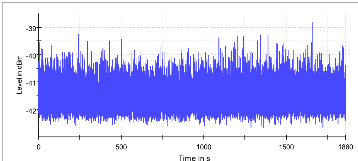
802.11ac (160 MHz) Channel 114
