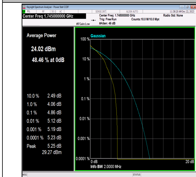
Band66-1.4MHz-QPSK-132322-1RB#0-PASS
