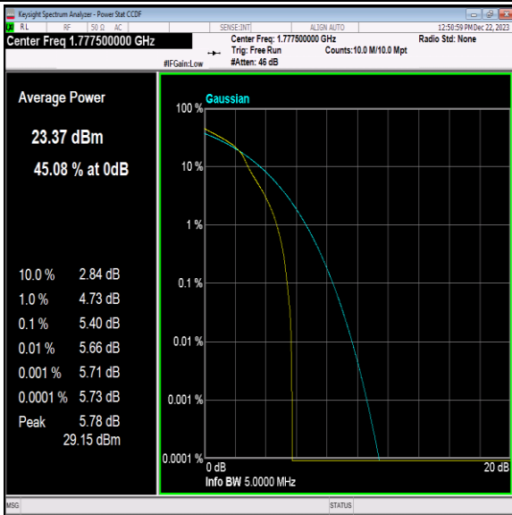
Band66-5MHz-16QAM-132647-1RB#0-PASS
