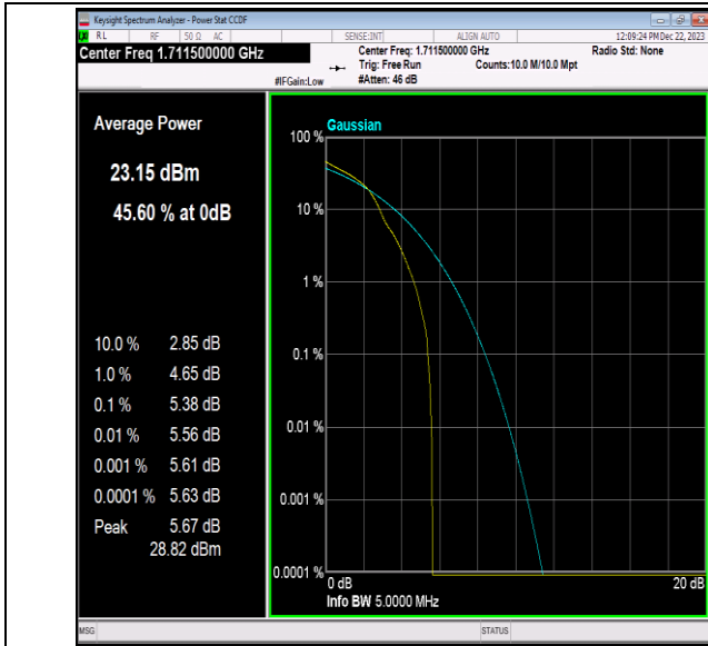
Band66-3MHz-16QAM-131987-1RB#0-PASS
