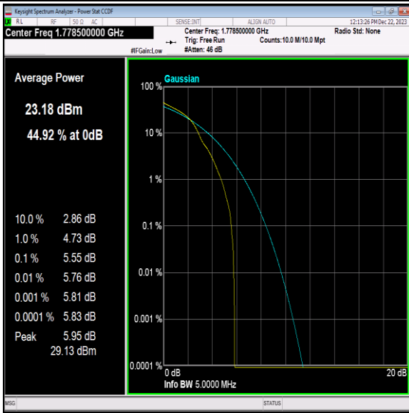
Band66-3MHz-16QAM-132657-1RB#0-PASS
