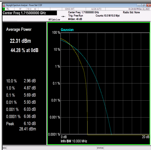
Band66-10MHz-64QAM-132022-1RB#0-PASS
