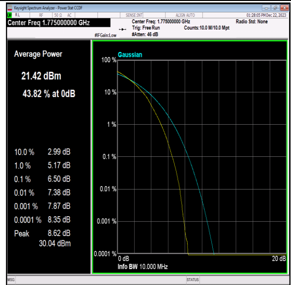
Band66-10MHz-64QAM-132622-50RB#0-PASS
