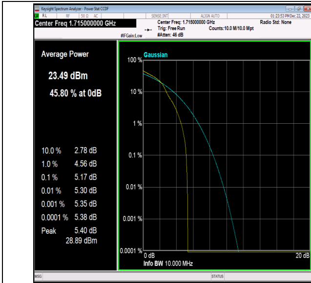
Band66-10MHz-16QAM-132022-1RB#0-PASS
