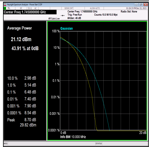
Band66-10MHz-64QAM-132322-50RB#0-PASS
