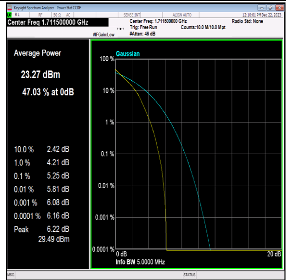
Band66-3MHz-QPSK-131987-15RB#0-PASS
