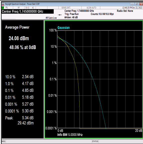
Band66-5MHz-QPSK-132322-1RB#0-PASS
