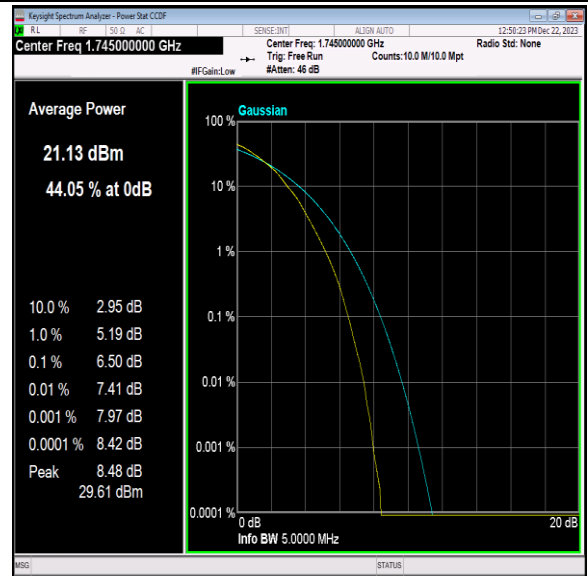
Band66-5MHz-64QAM-132322-25RB#0-PASS
