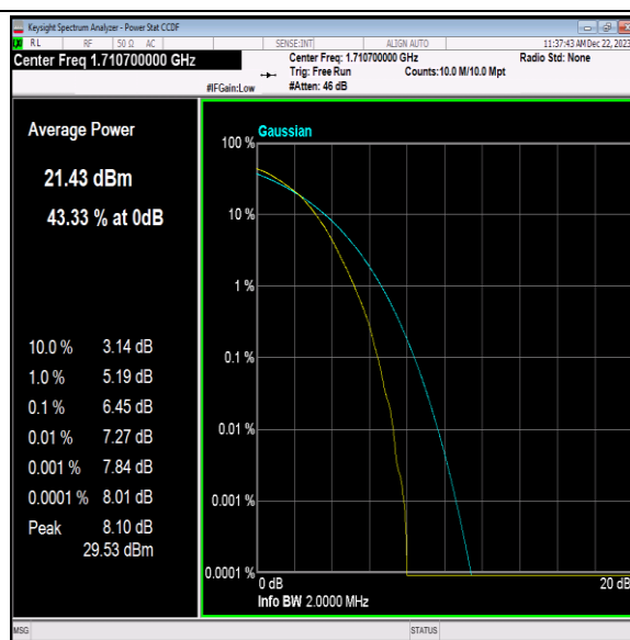
Band66-1.4MHz-64QAM-131979-6RB#0-PASS
