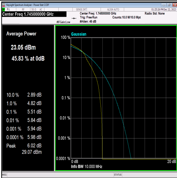
Band66-10MHz-16QAM-132322-1RB#0-PASS
