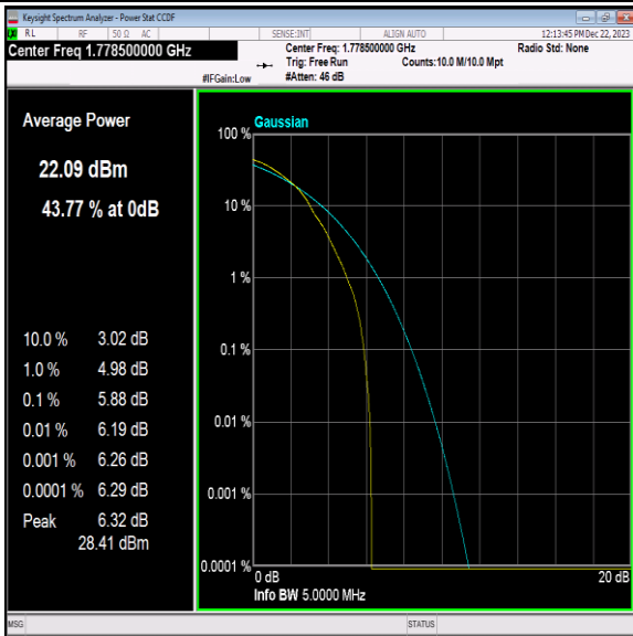
Band66-3MHz-64QAM-132657-1RB#0-PASS
