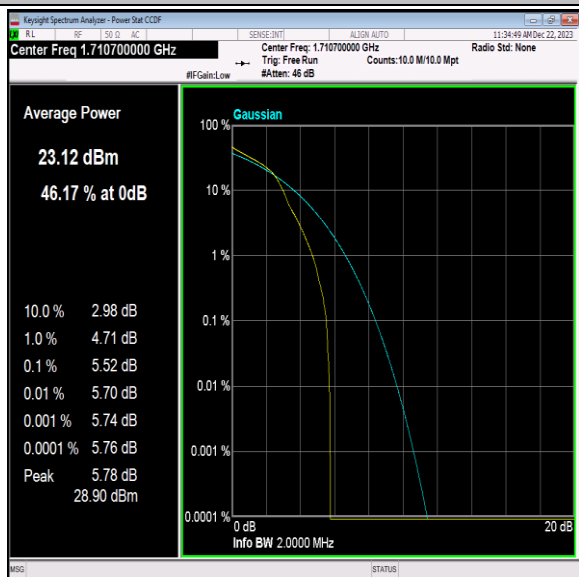
Band66-1.4MHz-16QAM-131979-1RB#0-PASS
