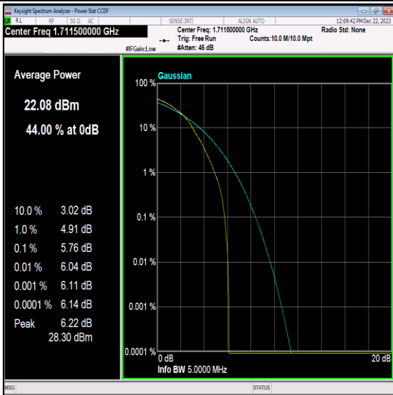
Band66-3MHz-64QAM-131987-1RB#0-PASS
