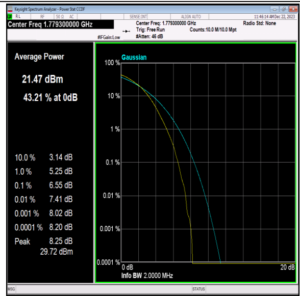
Band66-1.4MHz-64QAM-132665-6RB#0-PASS
