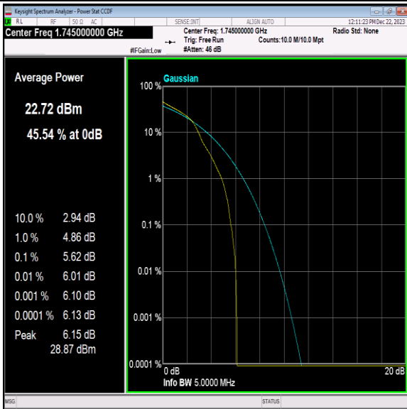
Band66-3MHz-16QAM-132322-1RB#0-PASS
