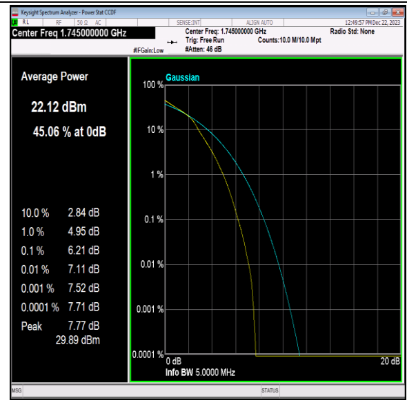
Band66-5MHz-16QAM-132322-25RB#0-PASS
