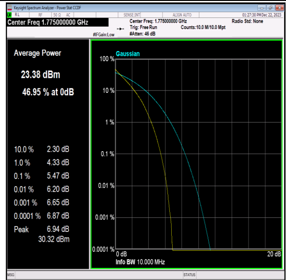
Band66-10MHz-QPSK-132622-50RB#0-PASS
