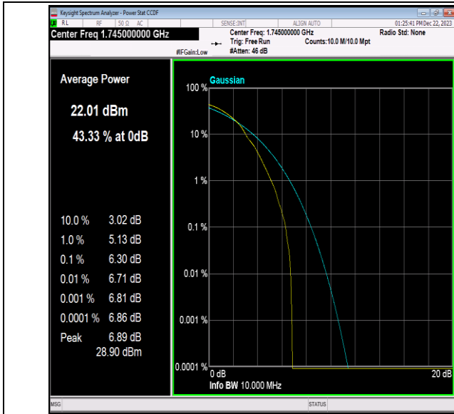
Band66-10MHz-64QAM-132322-1RB#0-PASS
