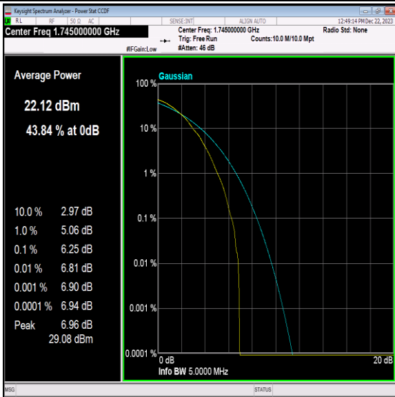
Band66-5MHz-64QAM-132322-1RB#0-PASS
