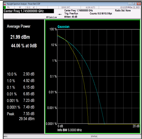
Band66-3MHz-16QAM-132322-15RB#0-PASS
