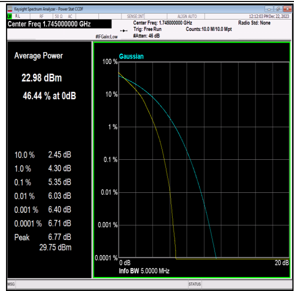
Band66-3MHz-QPSK-132322-15RB#0-PASS
