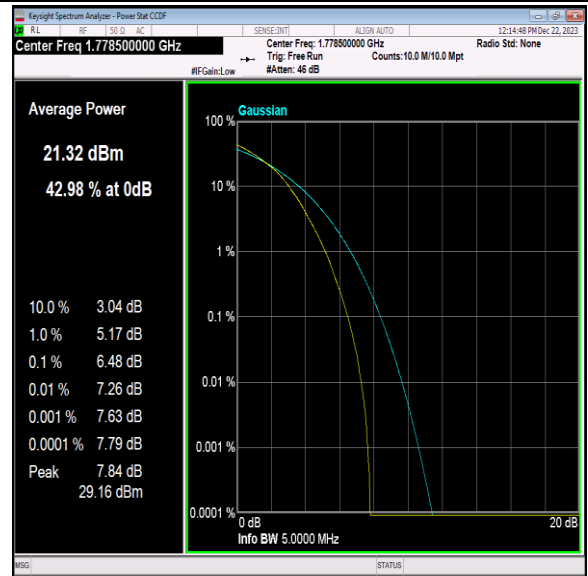
Band66-3MHz-64QAM-132657-15RB#0-PASS
