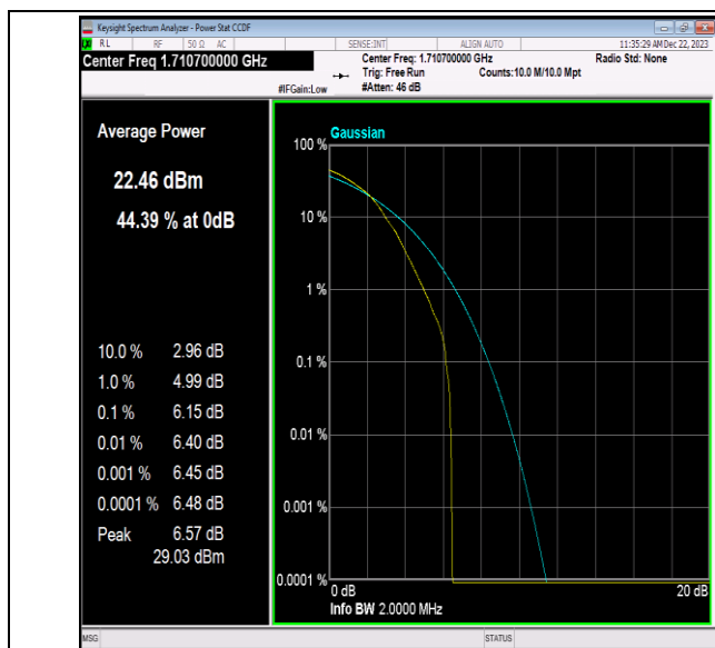
Band66-1.4MHz-64QAM-131979-1RB#0-PASS
