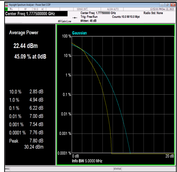
Band66-5MHz-16QAM-132647-25RB#0-PASS
