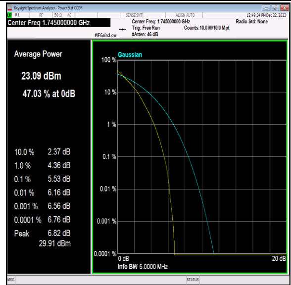
Band66-5MHz-QPSK-132322-25RB#0-PASS
