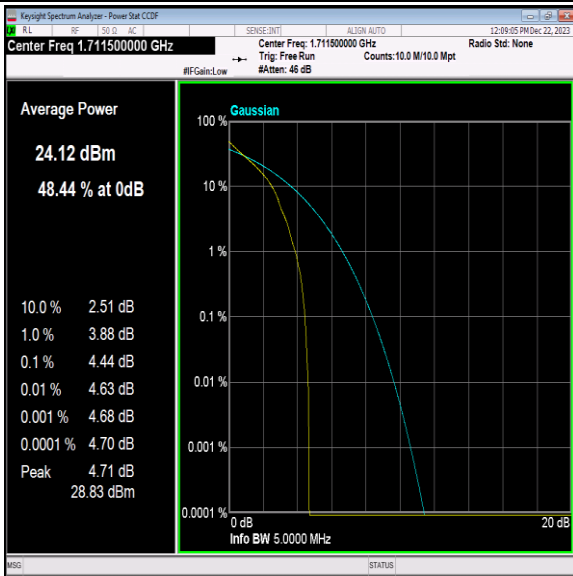
Band66-3MHz-QPSK-131987-1RB#0-PASS
