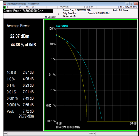
Band66-10MHz-16QAM-132322-50RB#0-PASS
