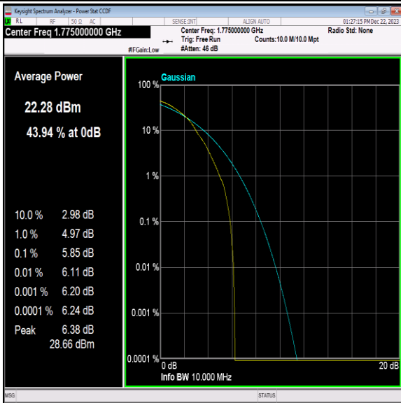
Band66-10MHz-64QAM-132622-1RB#0-PASS
