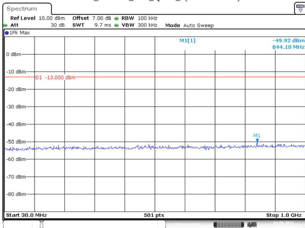
Band 2_1.4 MHz_Low_QPSK_1(30MHz-1GHz)
