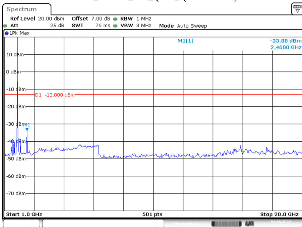
Band 2_1.4 MHz_Low_QPSK_2(1GHz-20GHz)
