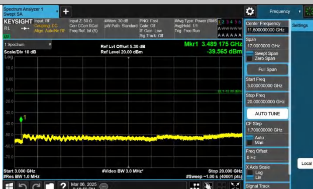
Band66-1.4MHz-QPSK-132322-1RB#0-3000~20000-PASS
