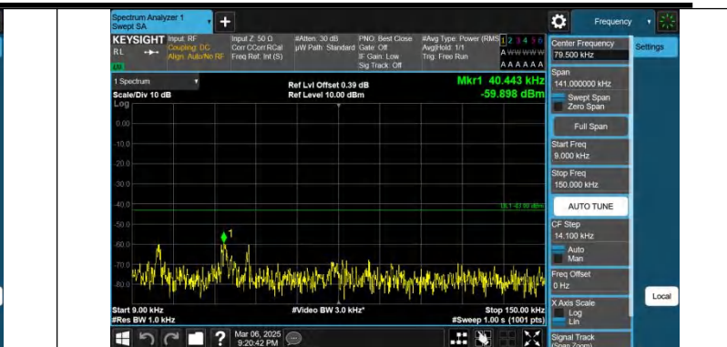
Band66-1.4MHz-QPSK-132665-1RB#5-0.009~0.15-PASS
