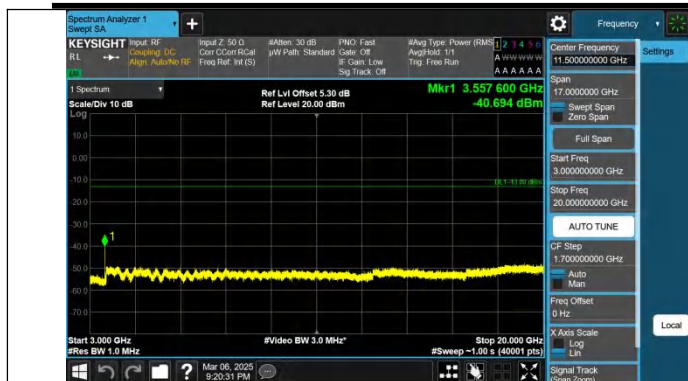
Band66-1.4MHz-QPSK-132665-1RB#0-3000~20000-PASS
