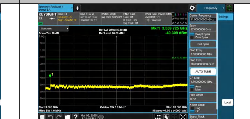
Band66-1.4MHz-QPSK-132665-1RB#5-3000~20000-PASS
