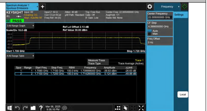
Band66-10MHz-QPSK-132022-50RB#0-PASS
