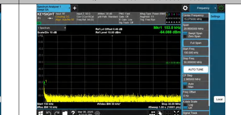
Band66-3MHz-QPSK-131987-1RB#0-0.15~30-PASS
