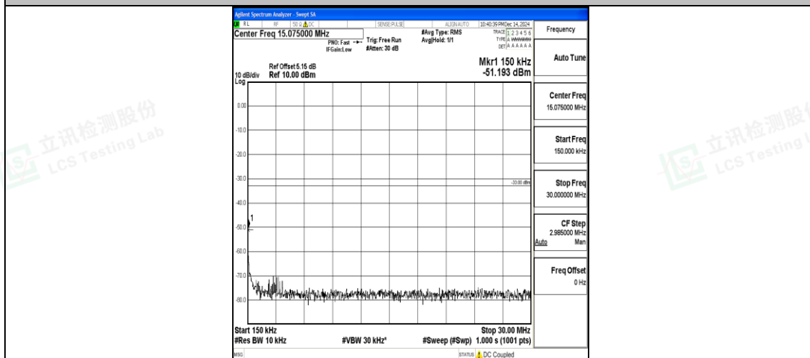
Band25_5MHz_16QAM_26665_1RB#0_0.15~30_0.15~30
