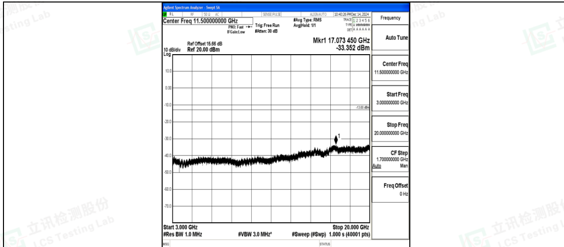
Band25_5MHz_QPSK_26665_1RB#0_3000~20000_3000~20000
