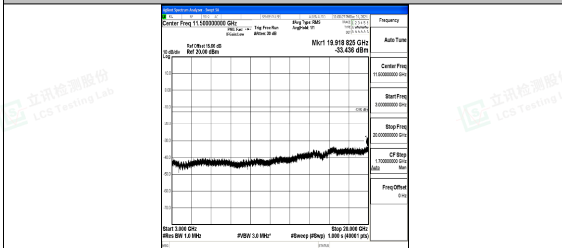
Band25_10MHz_16QAM_26640_1RB#0_3000~20000_3000~20000
