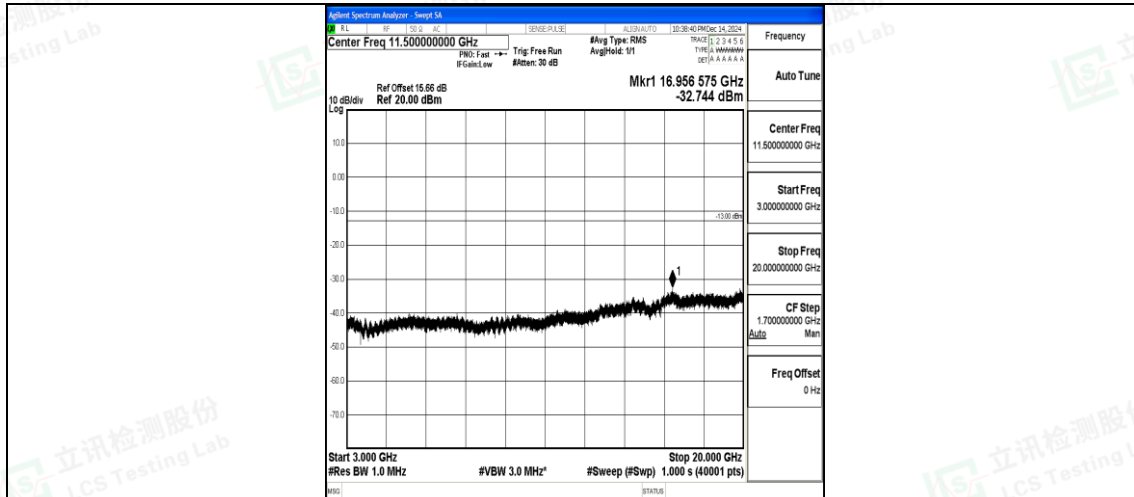
Band25_5MHz_16QAM_26065_1RB#0_3000~20000_3000~20000
