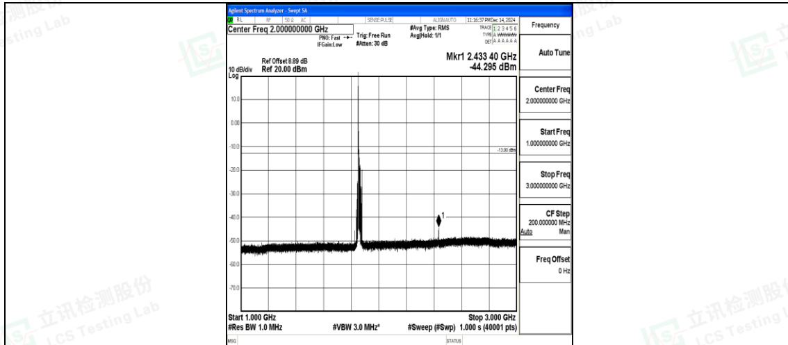
Band25_15MHz_QPSK_26115_1RB#0_1000~3000_1000~3000
