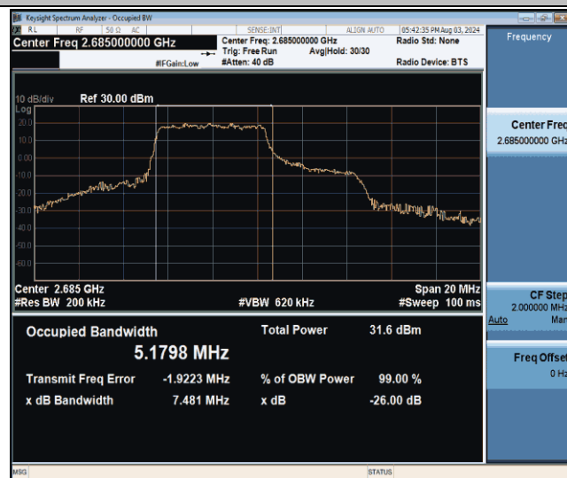
Band41-10MHz-16QAM-41540-27RB#0-PASS
