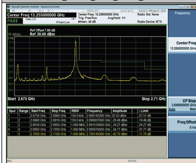
Band41_15MHz_QPSK_41515_1RB#74
