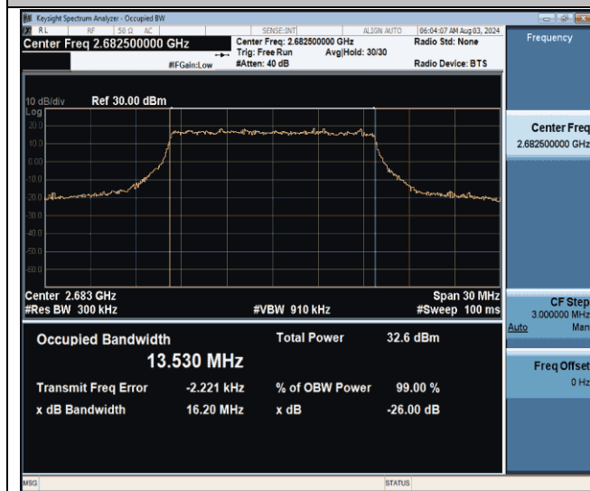
Band41-15MHz-QPSK-41515-75RB#0-PASS
