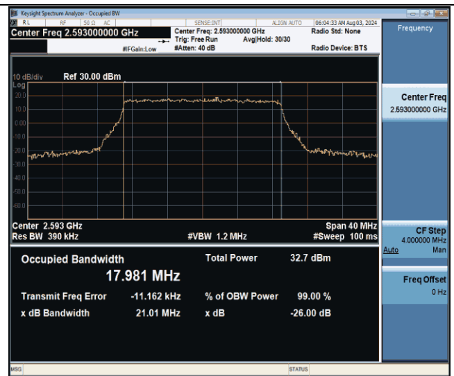
Band41-20MHz-QPSK-40620-100RB#0-PASS
