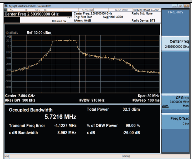
Band41-15MHz-16QAM-39725-27RB#0-PASS
