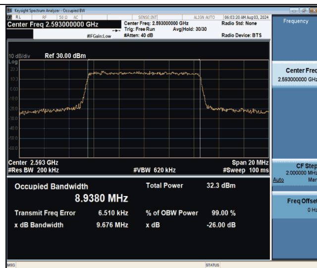
Band41-10MHz-QPSK-40620-50RB#0-PASS
