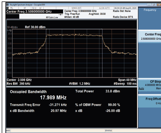
Band41-20MHz-QPSK-39750-100RB#0-PASS
