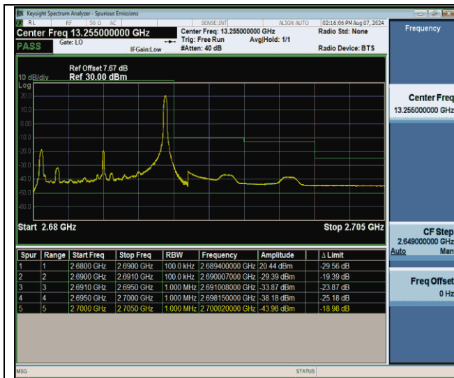
Band41_10MHz_QPSK_41540_1RB#49
