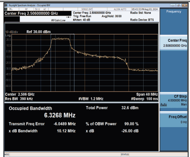
Band41-20MHz-16QAM-39750-27RB#0-PASS
