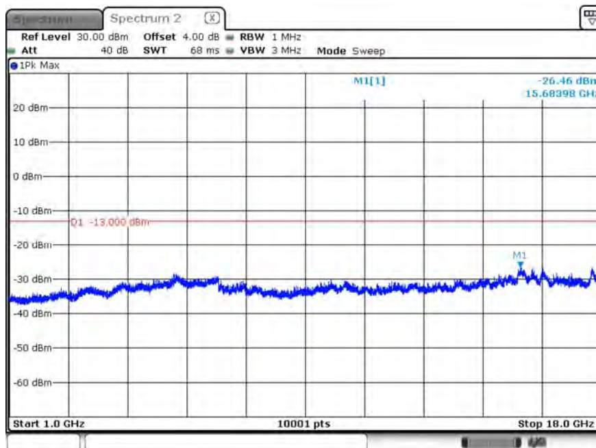
B5_CH20525_10M_1RB24_16-QAM_Above 1G
