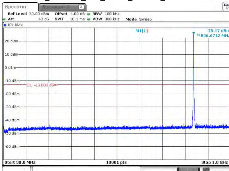
B5_CH20525_10M_1RB24_16-QAM_Below 1G
