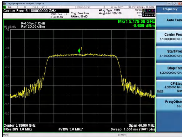
11AX20SISO-Ant1-5180-PASS
