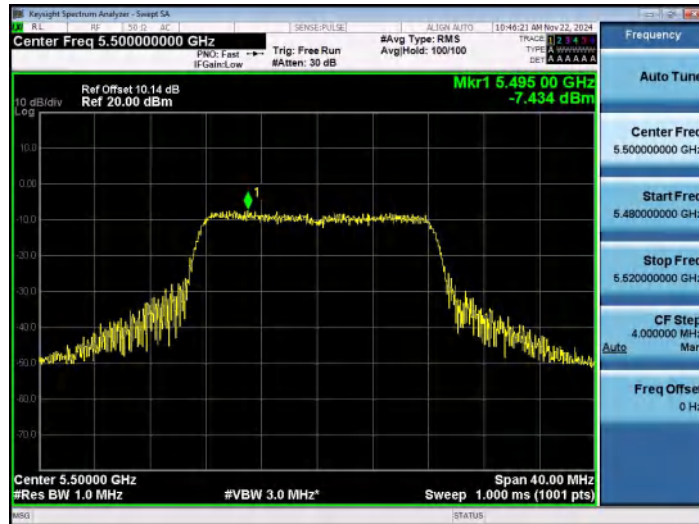
11A-Ant1-5500-PASS
