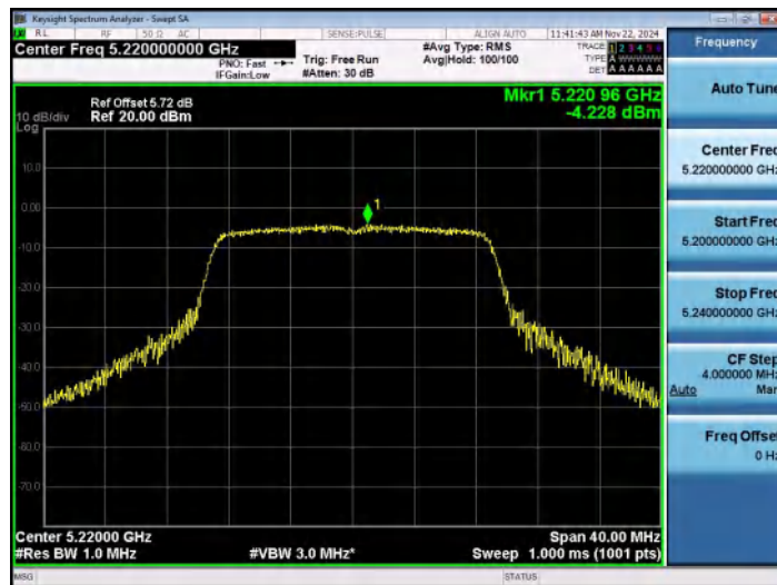
11AC20SISO-Ant1-5220-PASS
