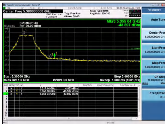
11N20SISO-Ant1-5320-PASS
