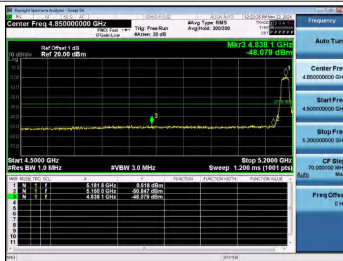
11AX20SISO-Ant1-5180-PASS
