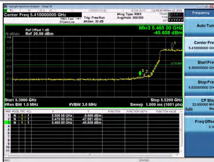
11AX40ISO-Ant1-5510-PASS
