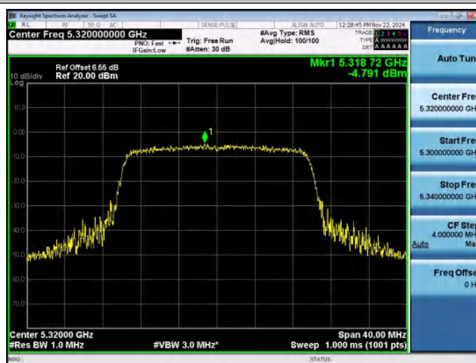
11AX20SISO-Ant1-5320-PASS
