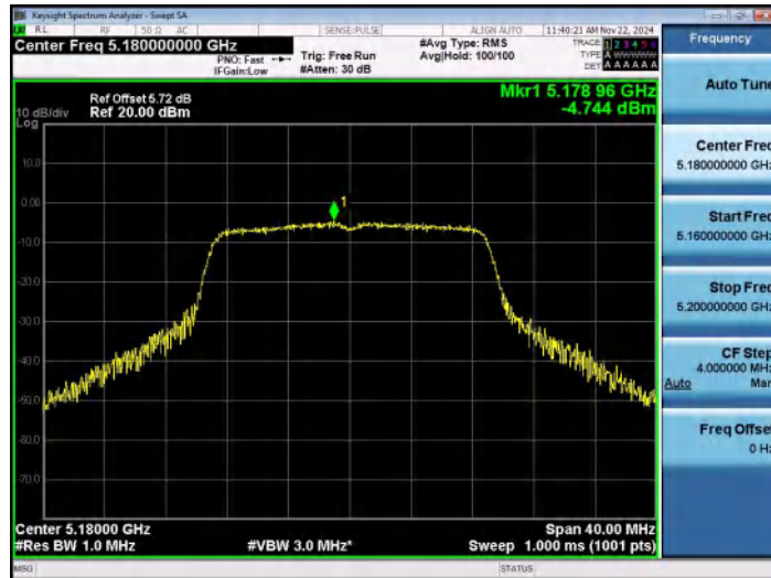
11AC20SISO-Ant1-5180-PASS
