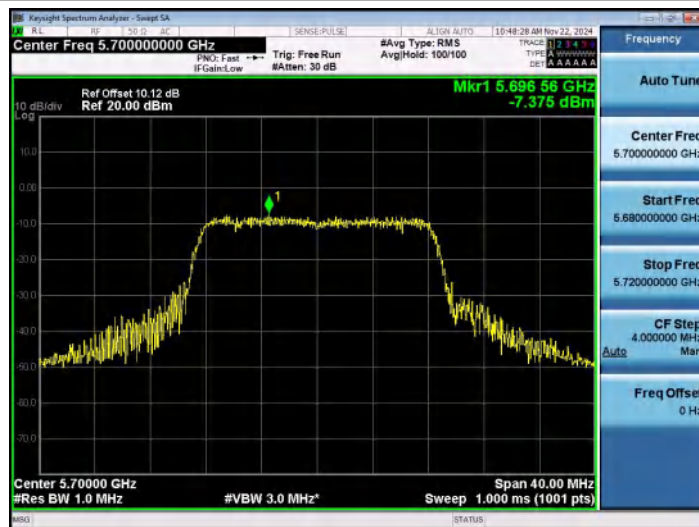
11A-Ant1-5700-PASS
