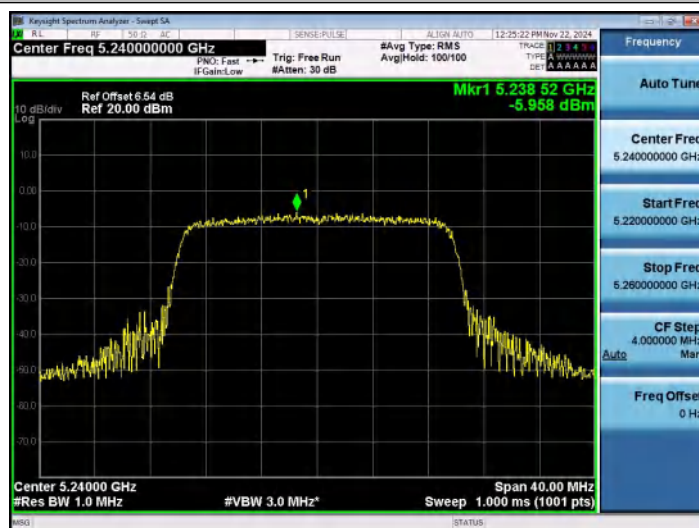
11AX20SISO-Ant1-5240-PASS
