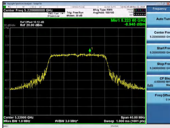
11A-Ant1-5220-PASS
