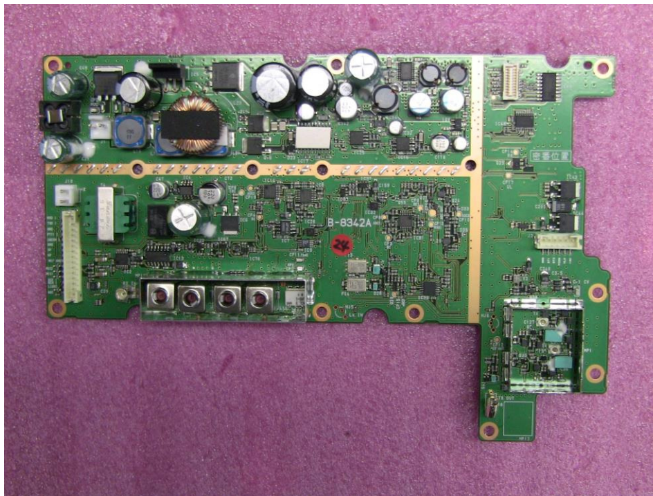
MAIN-C (TOP)
