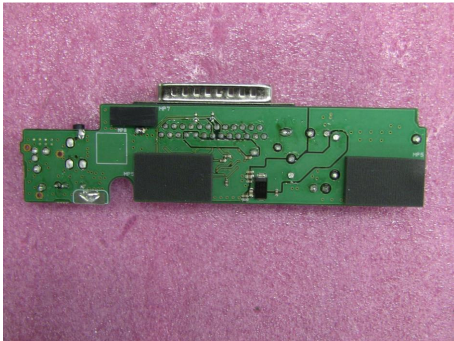
D-CONNECT-A(BOTTOM)
