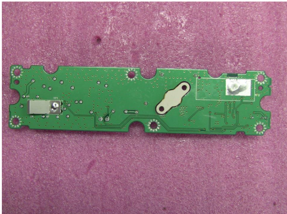
PA-C(BOTTOM)
