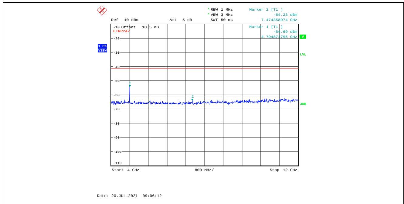
Plot 5.4.4.3.5. Conducted Spurious Emissions in Restricted Frequency Bands, High Power 2402 MHz, GFSK Modulation, 1 Mbps, 4 GHz - 12 GHz, Peak Detector
