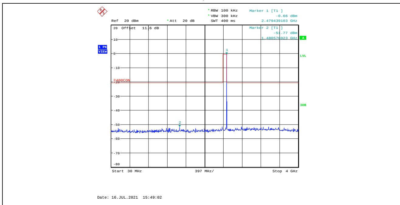
Plot 5.4.4.2.34. Conducted Spurious Emissions in Non-Restricted Frequency Bands, Low Power 2480 MHz, GFSK Modulation, 2 Mbps, 30 MHz – 4 GHz, Peak Detector
