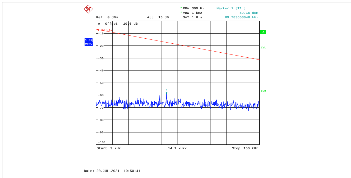
Plot 5.4.4.3.31. Conducted Spurious Emissions in Restricted Frequency Bands, High Power 2480 MHz, GFSK Modulation, 2 Mbps, 9 kHz - 150 kHz, Peak Detector
