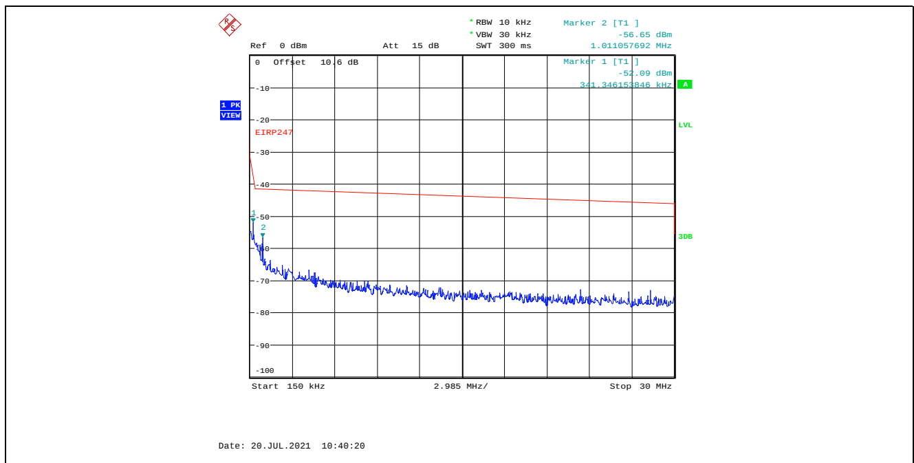
Plot 5.4.4.3.26. Conducted Spurious Emissions in Restricted Frequency Bands, High Power 2440 MHz, GFSK Modulation, 2 Mbps, 150 kHz - 30 MHz, Peak Detector
