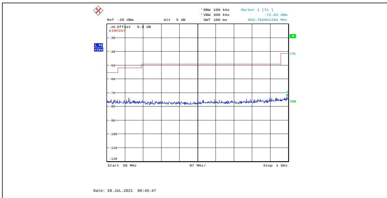
Plot 5.4.4.3.15. Conducted Spurious Emissions in Restricted Frequency Bands, High Power 2480 MHz, GFSK Modulation, 1 Mbps, 30 MHz - 1 GHz, Peak Detector
