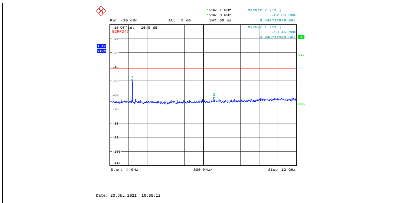
Plot 5.4.4.3.35. Conducted Spurious Emissions in Restricted Frequency Bands, High Power 2480 MHz, GFSK Modulation, 2 Mbps, 4 GHz - 12 GHz, Peak Detector
