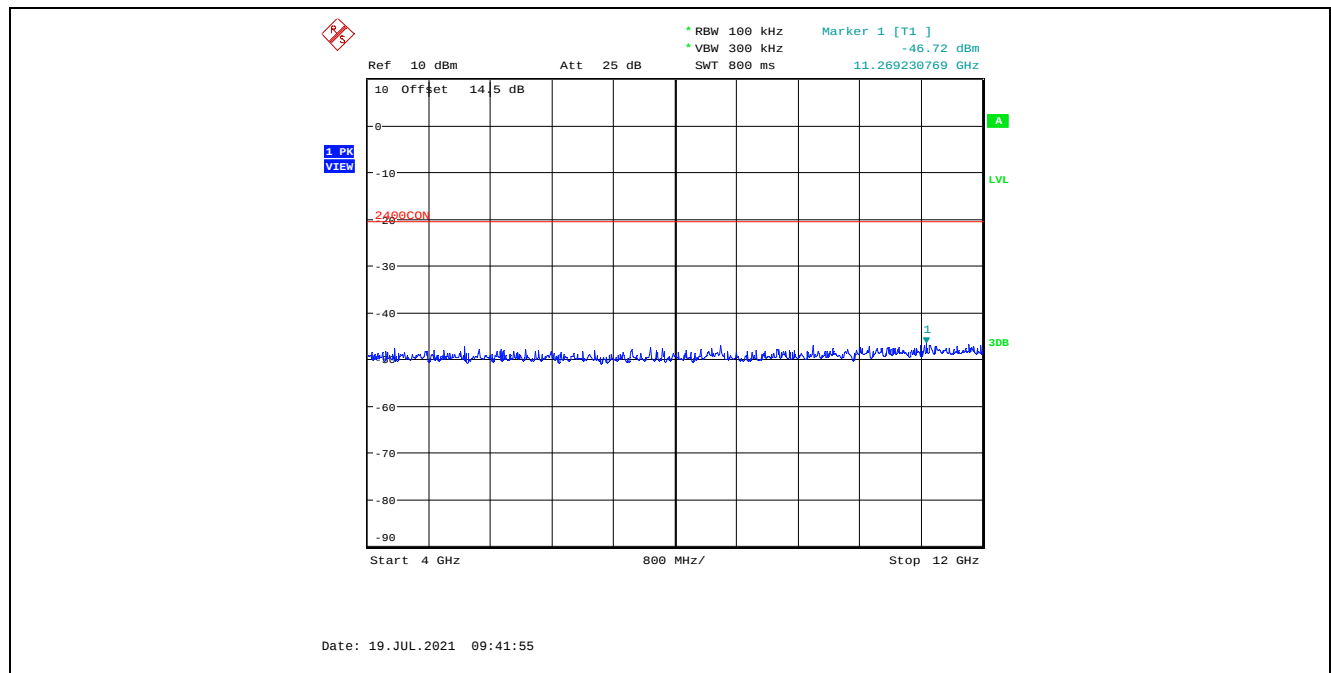
Plot 5.4.4.2.35. Conducted Spurious Emissions in Non-Restricted Frequency Bands, Low Power 2480 MHz, GFSK Modulation, 2 Mbps, 4 GHz – 12 GHz, Peak Detector
