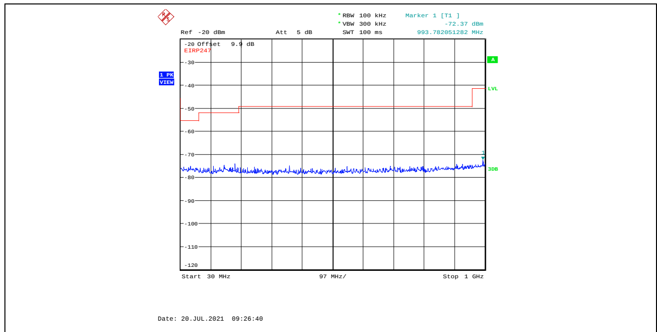
Plot 5.4.4.3.9. Conducted Spurious Emissions in Restricted Frequency Bands, High Power 2440 MHz, GFSK Modulation, 1 Mbps, 30 MHz - 1 GHz, Peak Detector
