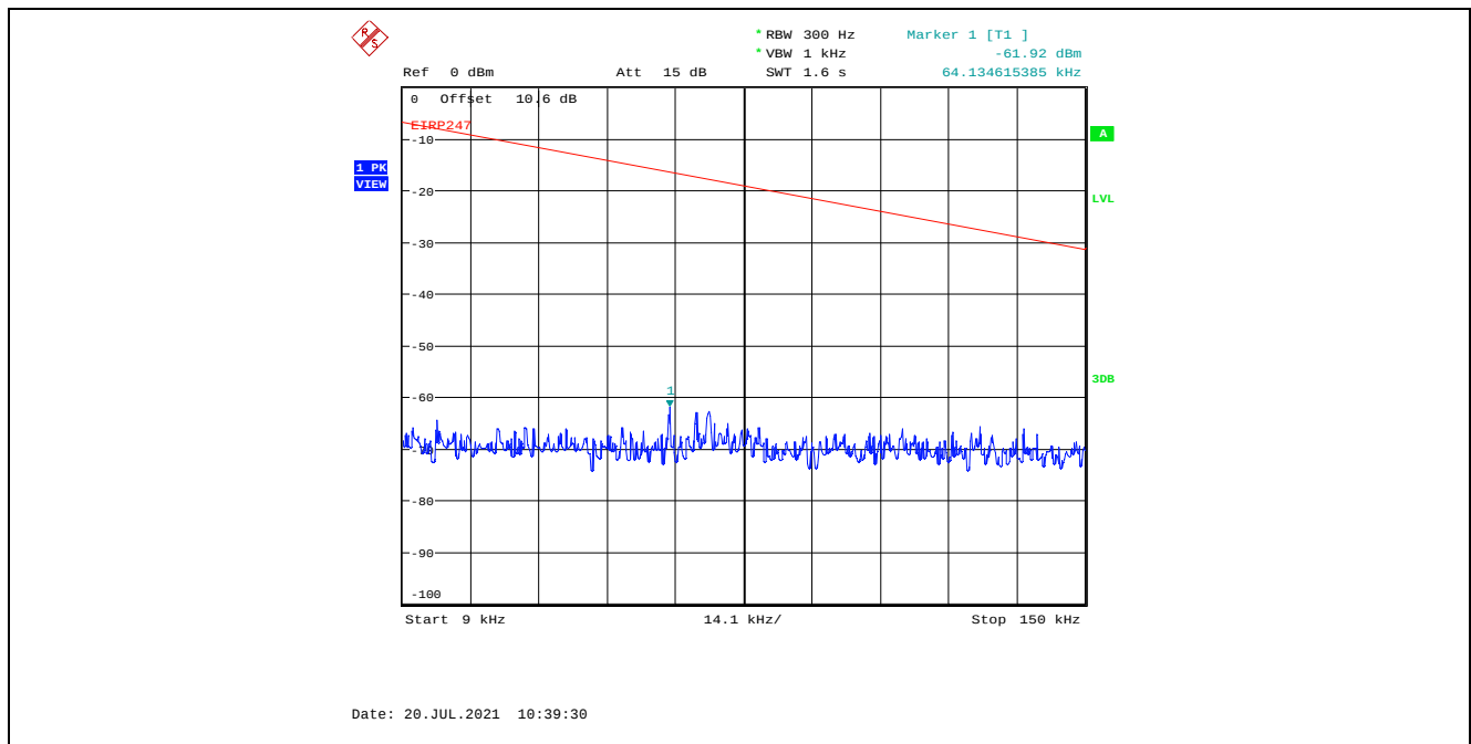
Plot 5.4.4.3.25. Conducted Spurious Emissions in Restricted Frequency Bands, High Power 2440 MHz, GFSK Modulation, 2 Mbps, 9 kHz - 150 kHz, Peak Detector
