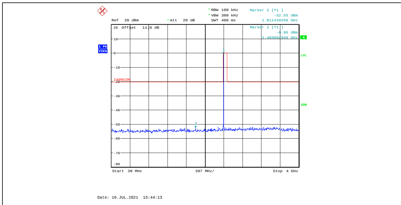
Plot 5.4.4.2.28. Conducted Spurious Emissions in Non-Restricted Frequency Bands, Low Power 2402 MHz, GFSK Modulation, 2 Mbps, 30 MHz – 4 GHz, Peak Detector
