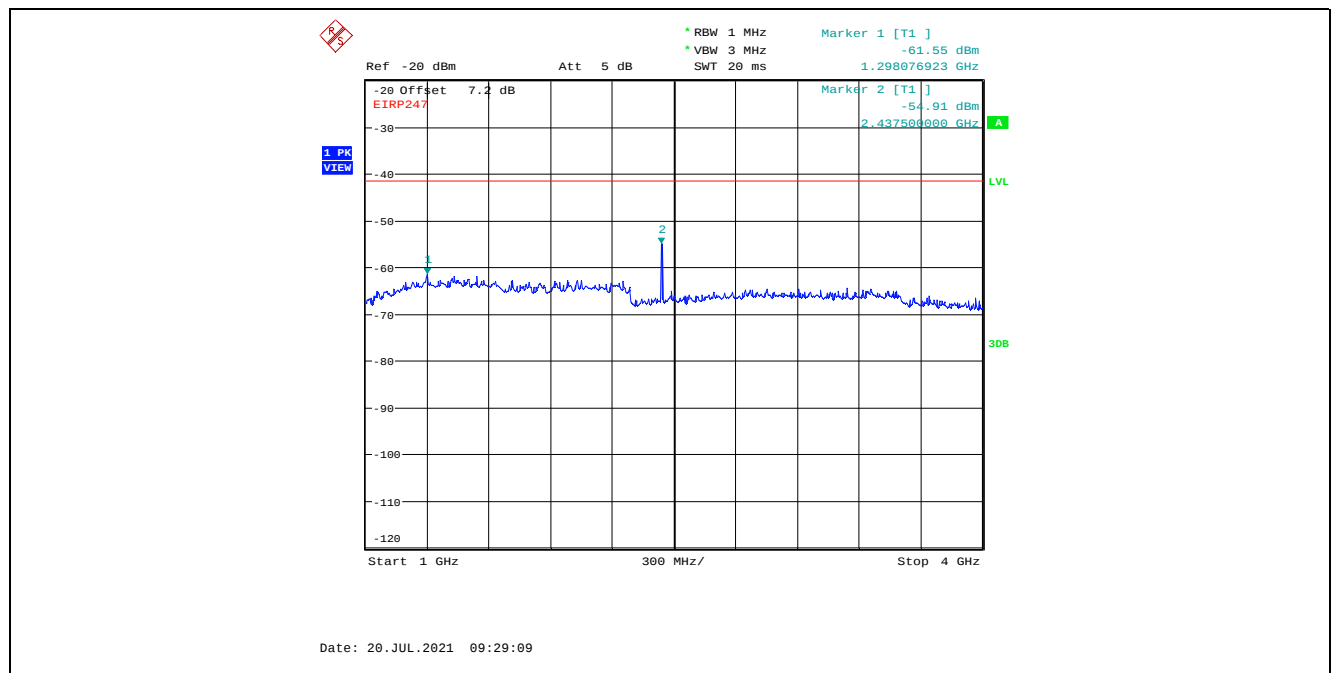
Plot 5.4.4.3.10. Conducted Spurious Emissions in Restricted Frequency Bands, High Power 2440 MHz, GFSK Modulation, 1 Mbps, 1 GHz - 4 GHz, Peak Detector
