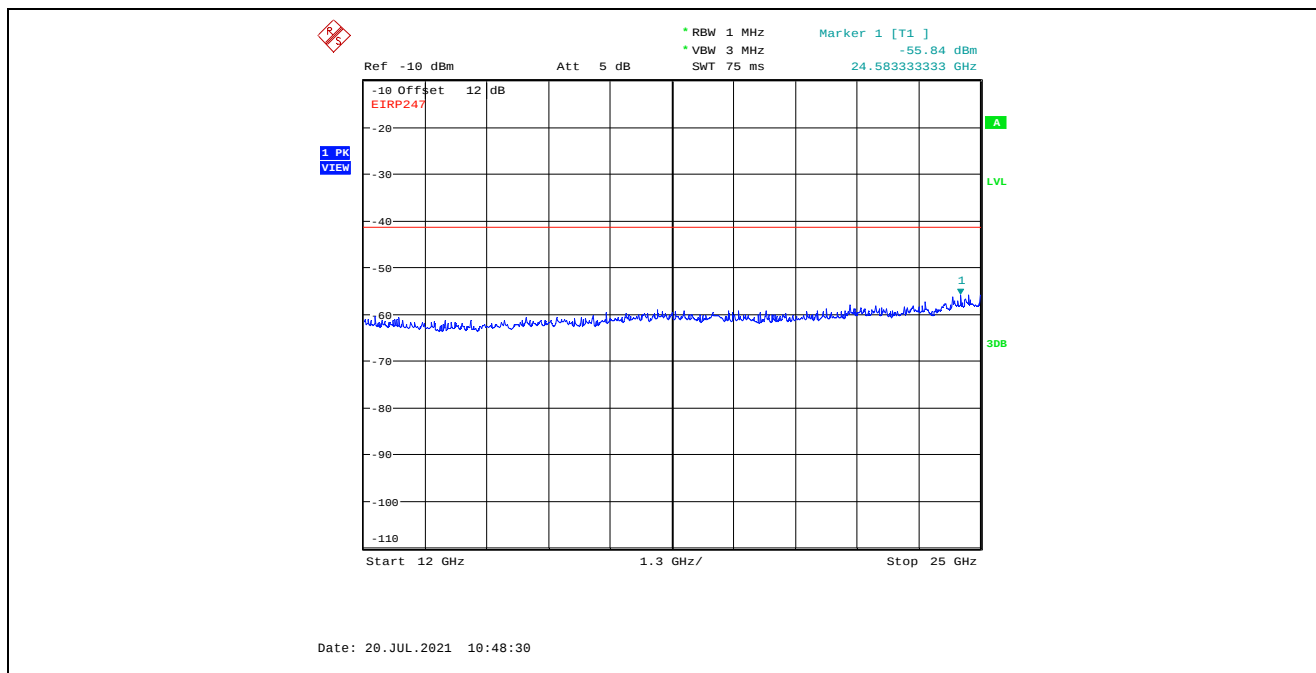
Plot 5.4.4.3.36. Conducted Spurious Emissions in Restricted Frequency Bands, High Power 2480 MHz, GFSK Modulation, 2 Mbps, 12 GHz - 25 GHz, Peak Detector
