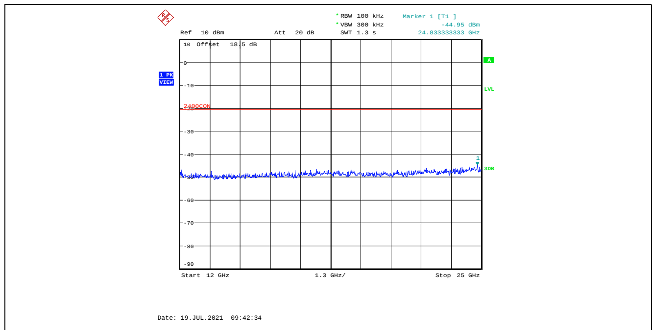
Plot 5.4.4.2.36. Conducted Spurious Emissions in Non-Restricted Frequency Bands, Low Power 2480 MHz, GFSK Modulation, 2 Mbps, 12 GHz – 25 GHz, Peak Detector
