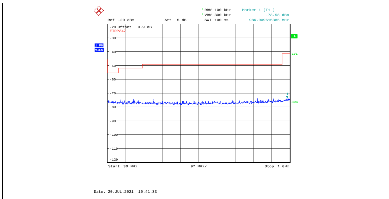
Plot 5.4.4.3.27. Conducted Spurious Emissions in Restricted Frequency Bands, High Power 2440 MHz, GFSK Modulation, 2 Mbps, 30 MHz - 1 GHz, Peak Detector
