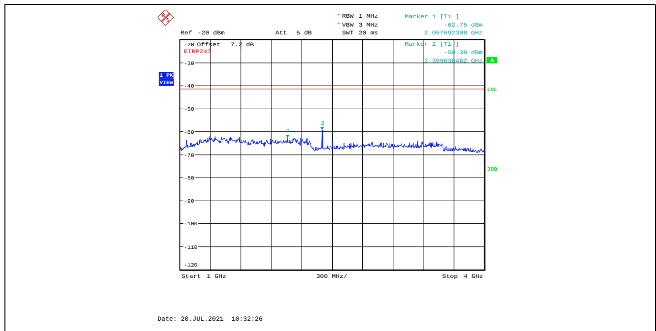
Plot 5.4.4.3.22. Conducted Spurious Emissions in Restricted Frequency Bands, High Power 2402 MHz, GFSK Modulation, 2 Mbps, 1 GHz - 4 GHz, Peak Detector
