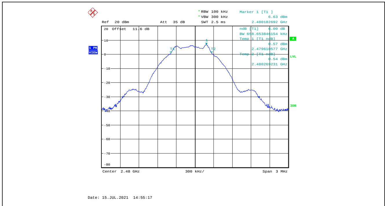
Plot 5.2.4.3. 6 dB Bandwidth, GFSK Modulation, 6 dBm Power Setting, 2480 MHz, 1 Mbps
