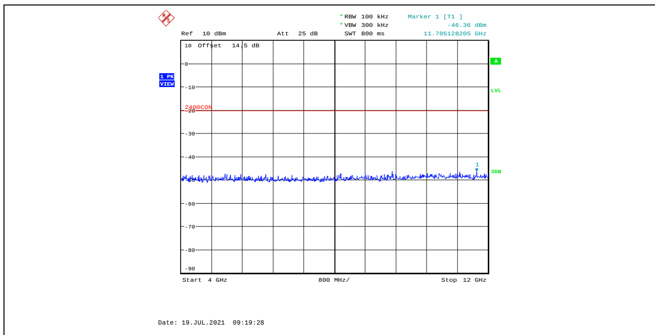
Plot 5.4.4.2.17. Conducted Spurious Emissions in Non-Restricted Frequency Bands, Low Power 2480 MHz, GFSK Modulation, 1 Mbps, 4 GHz – 12 GHz, Peak Detector
