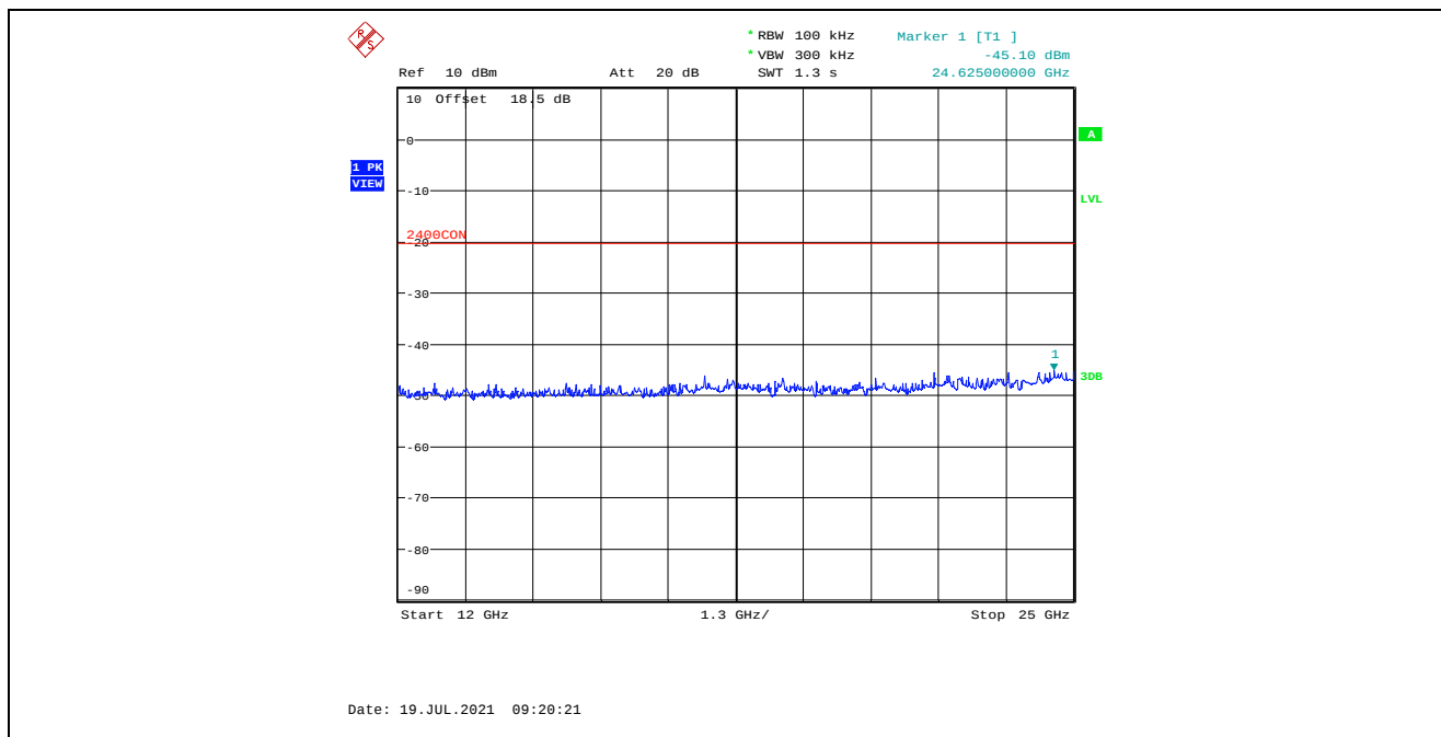
Plot 5.4.4.2.18. Conducted Spurious Emissions in Non-Restricted Frequency Bands, Low Power 2480 MHz, GFSK Modulation, 1 Mbps, 12 GHz – 25 GHz, Peak Detector
