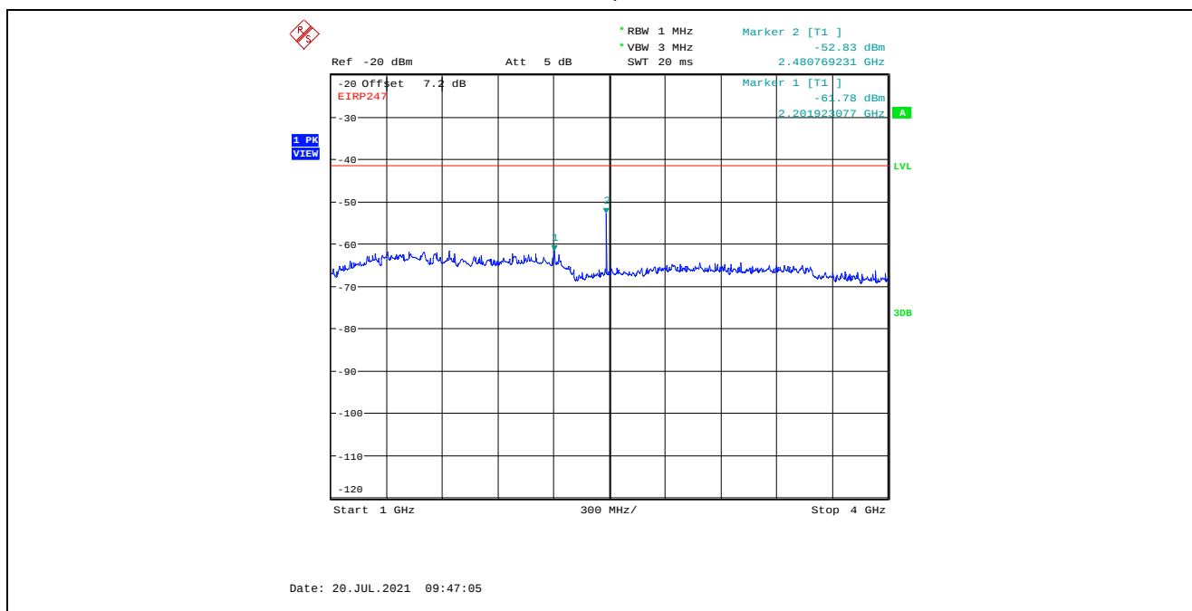
Plot 5.4.4.3.16. Conducted Spurious Emissions in Restricted Frequency Bands, High Power 2480 MHz, GFSK Modulation, 1 Mbps, 1 GHz - 4 GHz, Peak Detector
