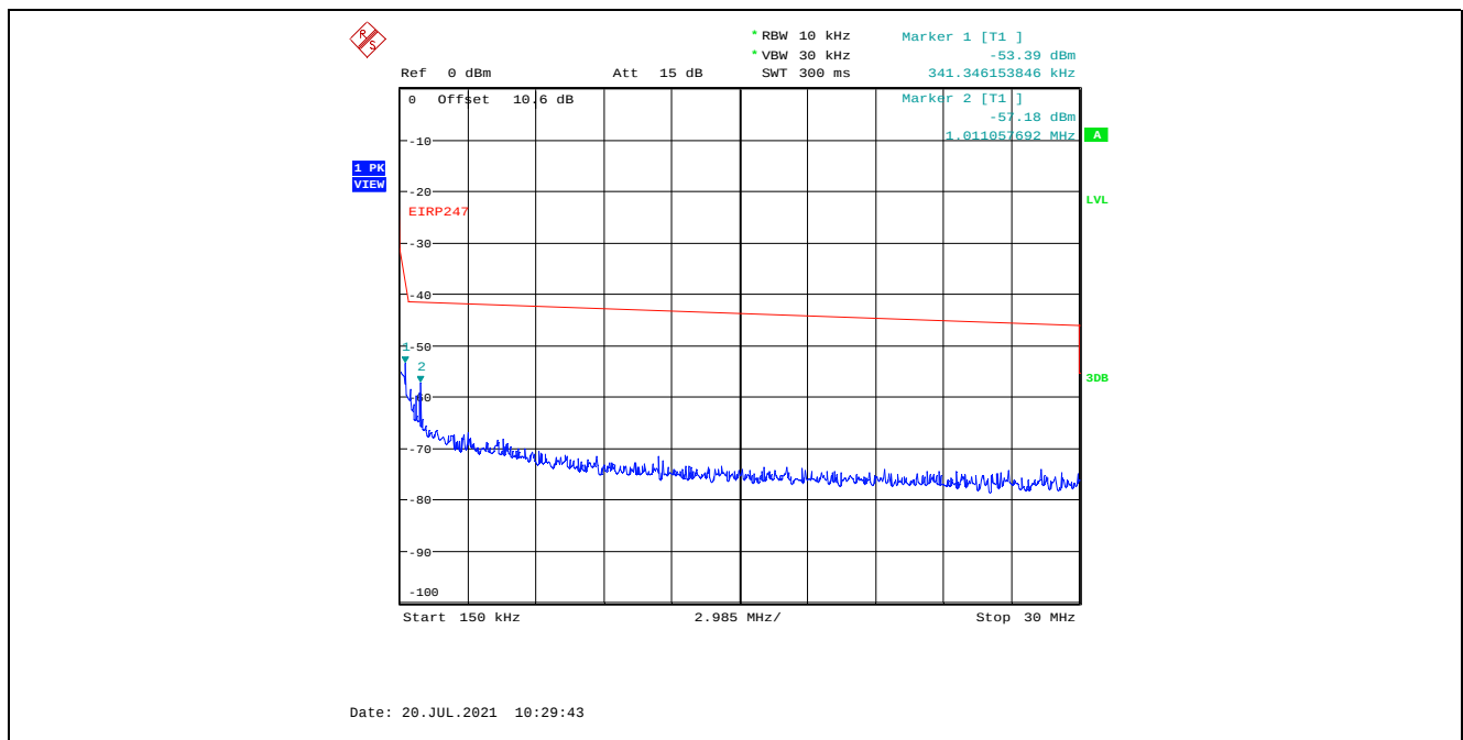
Plot 5.4.4.3.20. Conducted Spurious Emissions in Restricted Frequency Bands, High Power 2402 MHz, GFSK Modulation, 2 Mbps, 150 kHz - 30 MHz, Peak Detector
