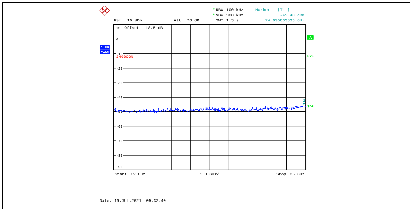
Plot 5.4.4.2.27. Conducted Spurious Emissions in Non-Restricted Frequency Bands, High Power 2480 MHz, GFSK Modulation, 2 Mbps, 12 GHz – 25 GHz, Peak Detector
