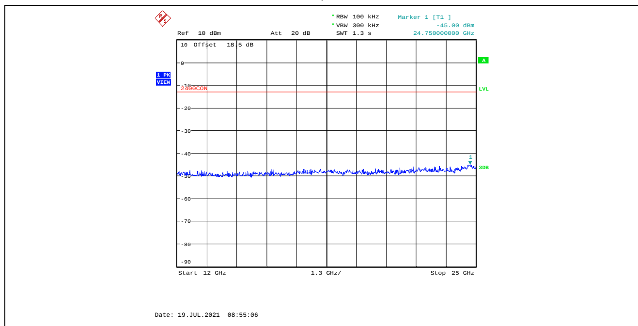
Plot 5.4.4.2.6. Conducted Spurious Emissions in Non-Restricted Frequency Bands, High Power 2440 MHz, GFSK Modulation, 1 Mbps, 12 GHz – 25 GHz, Peak Detector
