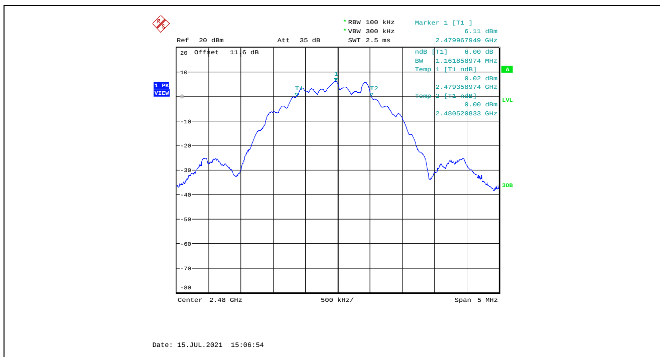
Plot 5.2.4.6. 6 dB Bandwidth, GFSK Modulation, 6 dBm Power Setting, 2480 MHz, 2 Mbps
