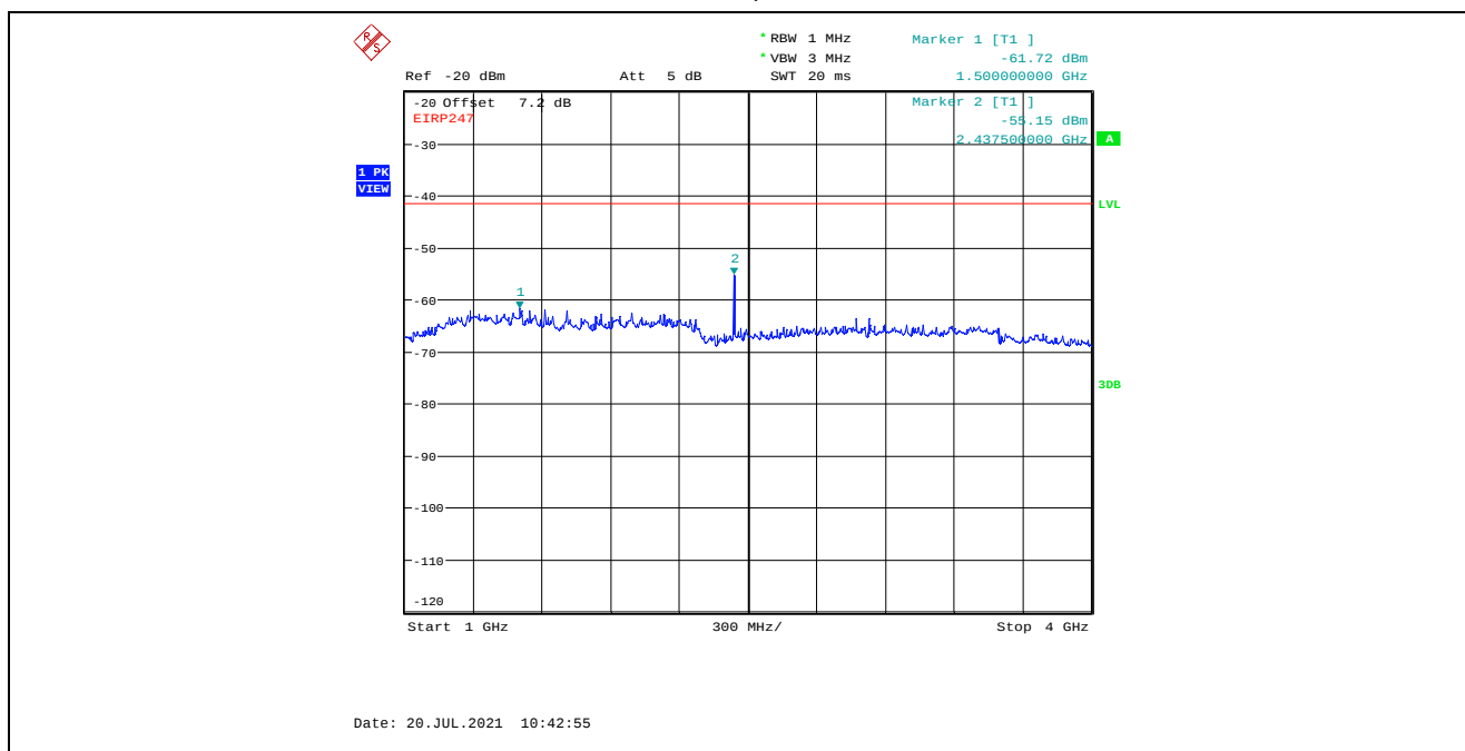
Plot 5.4.4.3.28. Conducted Spurious Emissions in Restricted Frequency Bands, High Power 2440 MHz, GFSK Modulation, 2 Mbps, 1 GHz - 4 GHz, Peak Detector
