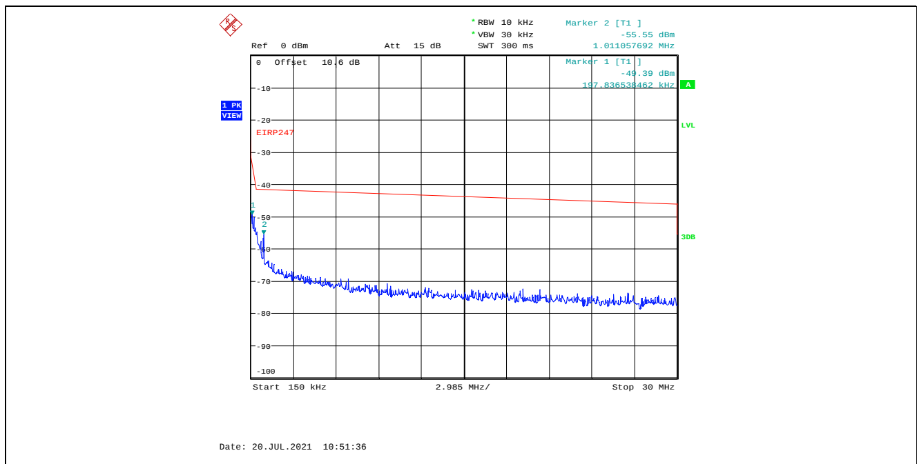
Plot 5.4.4.3.32. Conducted Spurious Emissions in Restricted Frequency Bands, High Power 2480 MHz, GFSK Modulation, 2 Mbps, 150 kHz - 30 MHz, Peak Detector
