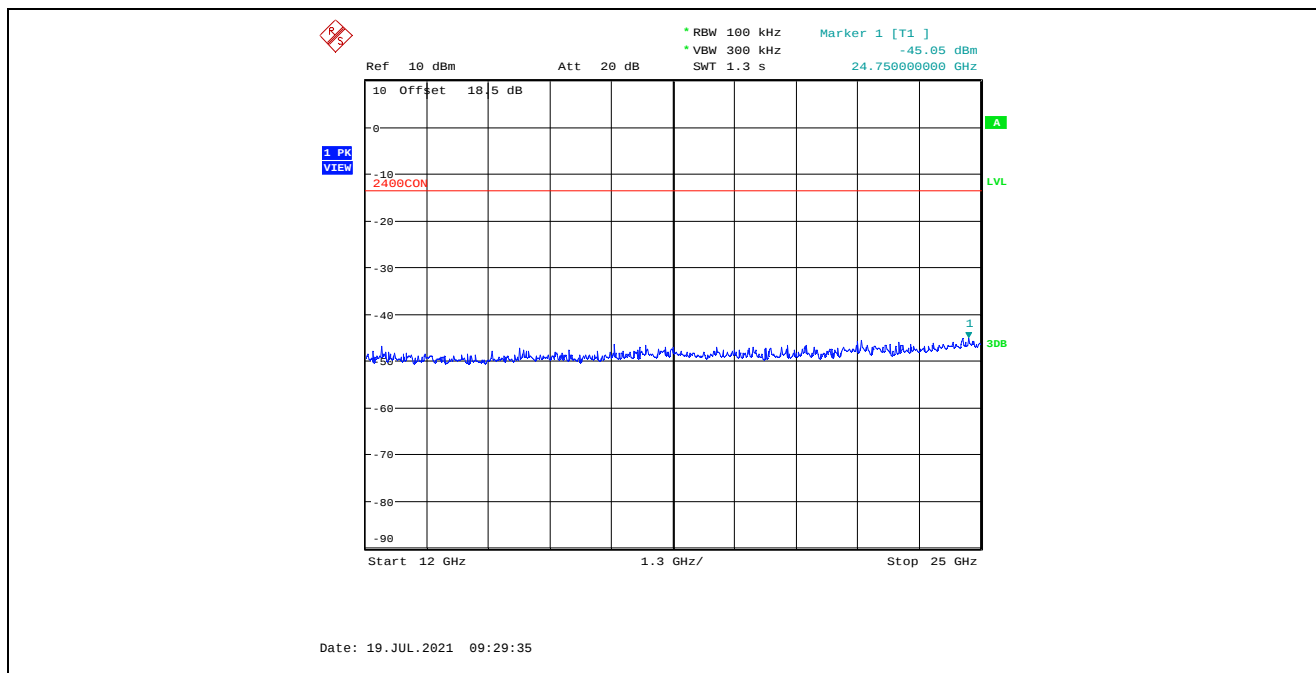
Plot 5.4.4.2.24. Conducted Spurious Emissions in Non-Restricted Frequency Bands, High Power 2440 MHz, GFSK Modulation, 2 Mbps, 12 GHz – 25 GHz, Peak Detector
