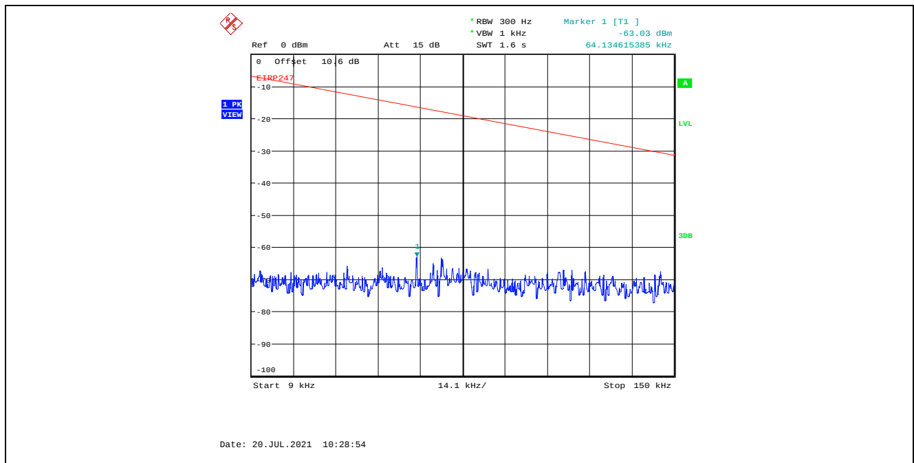
Plot 5.4.4.3.19. Conducted Spurious Emissions in Restricted Frequency Bands, High Power 2402 MHz, GFSK Modulation, 2 Mbps, 9 kHz - 150 kHz, Peak Detector
