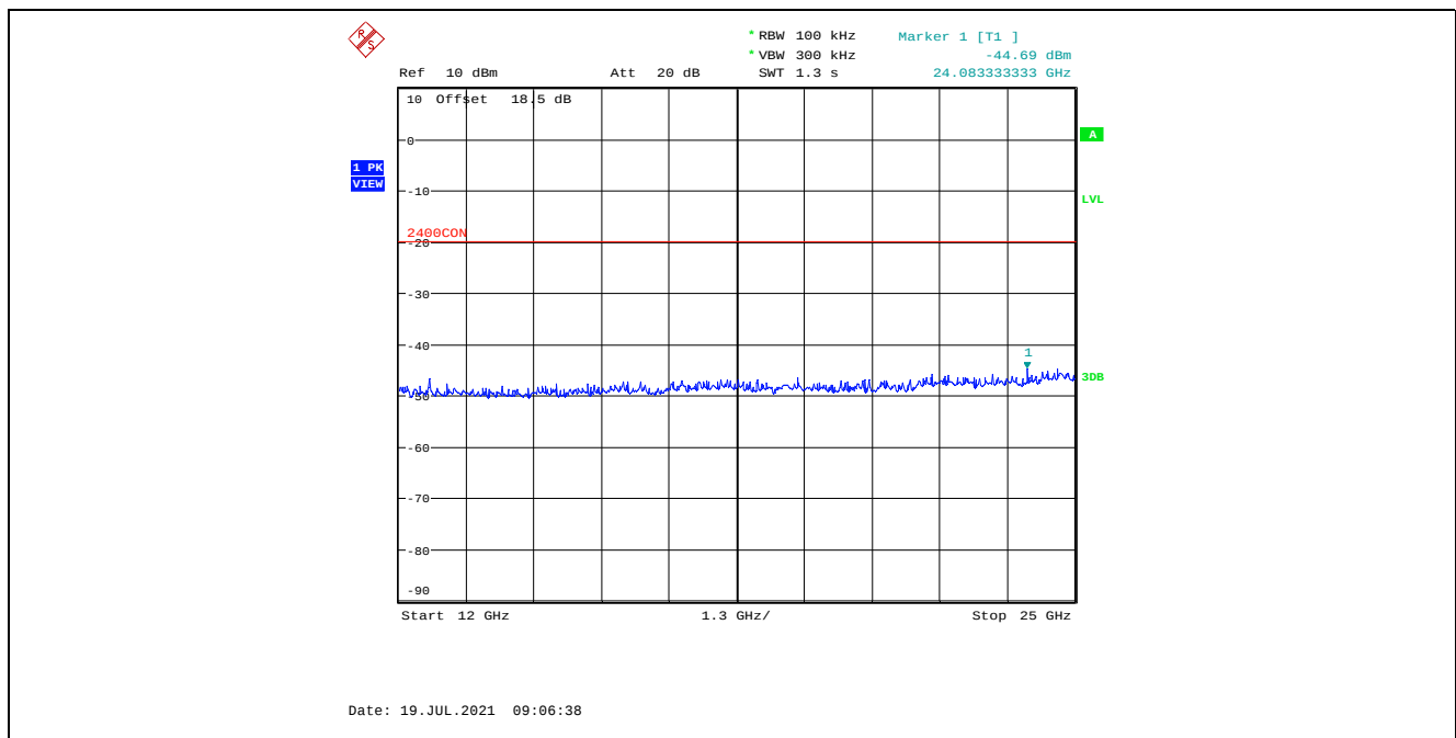
Plot 5.4.4.2.12. Conducted Spurious Emissions in Non-Restricted Frequency Bands, Low Power 2402 MHz, GFSK Modulation, 1 Mbps, 12 GHz – 25 GHz, Peak Detector
