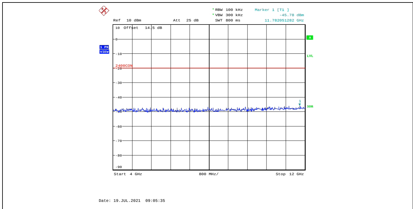
Plot 5.4.4.2.11. Conducted Spurious Emissions in Non-Restricted Frequency Bands, Low Power 2402 MHz, GFSK Modulation, 1 Mbps, 4 GHz – 12 GHz, Peak Detector
