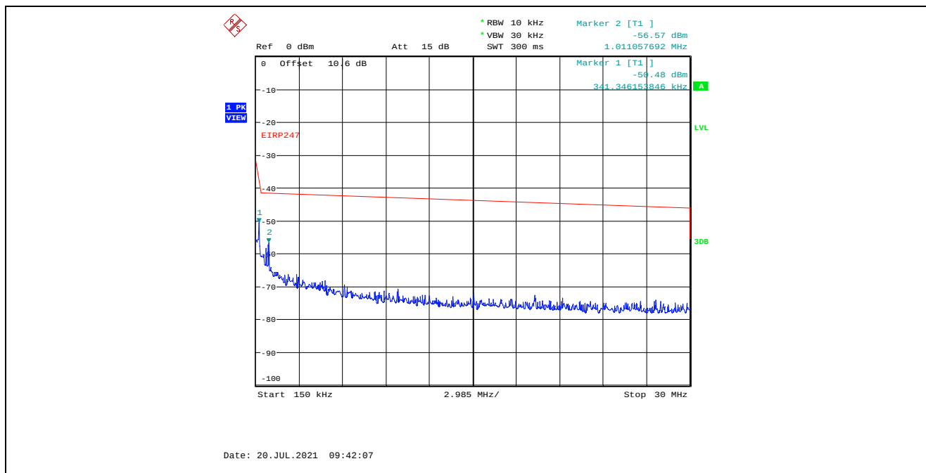
Plot 5.4.4.3.8. Conducted Spurious Emissions in Restricted Frequency Bands, High Power 2440 MHz, GFSK Modulation, 1 Mbps, 150 kHz - 30 MHz, Peak Detector
