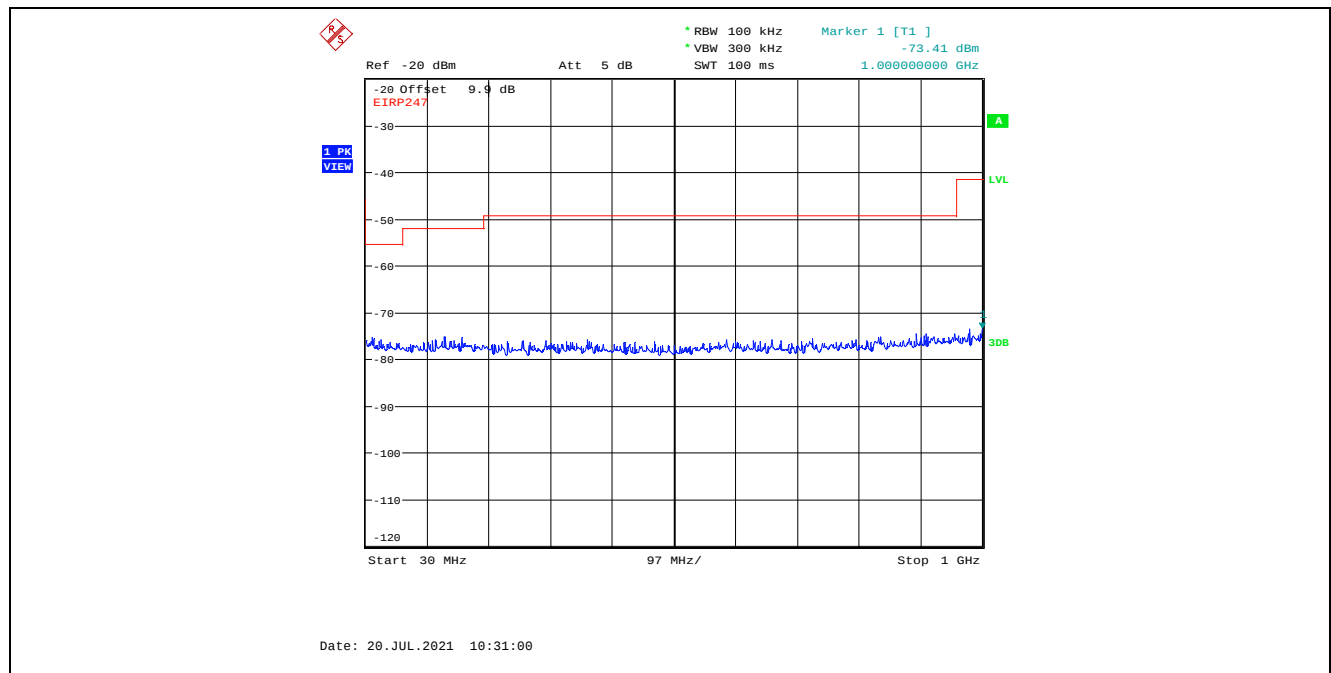
Plot 5.4.4.3.21. Conducted Spurious Emissions in Restricted Frequency Bands, High Power 2402 MHz, GFSK Modulation, 2 Mbps, 30 MHz - 1 GHz, Peak Detector
