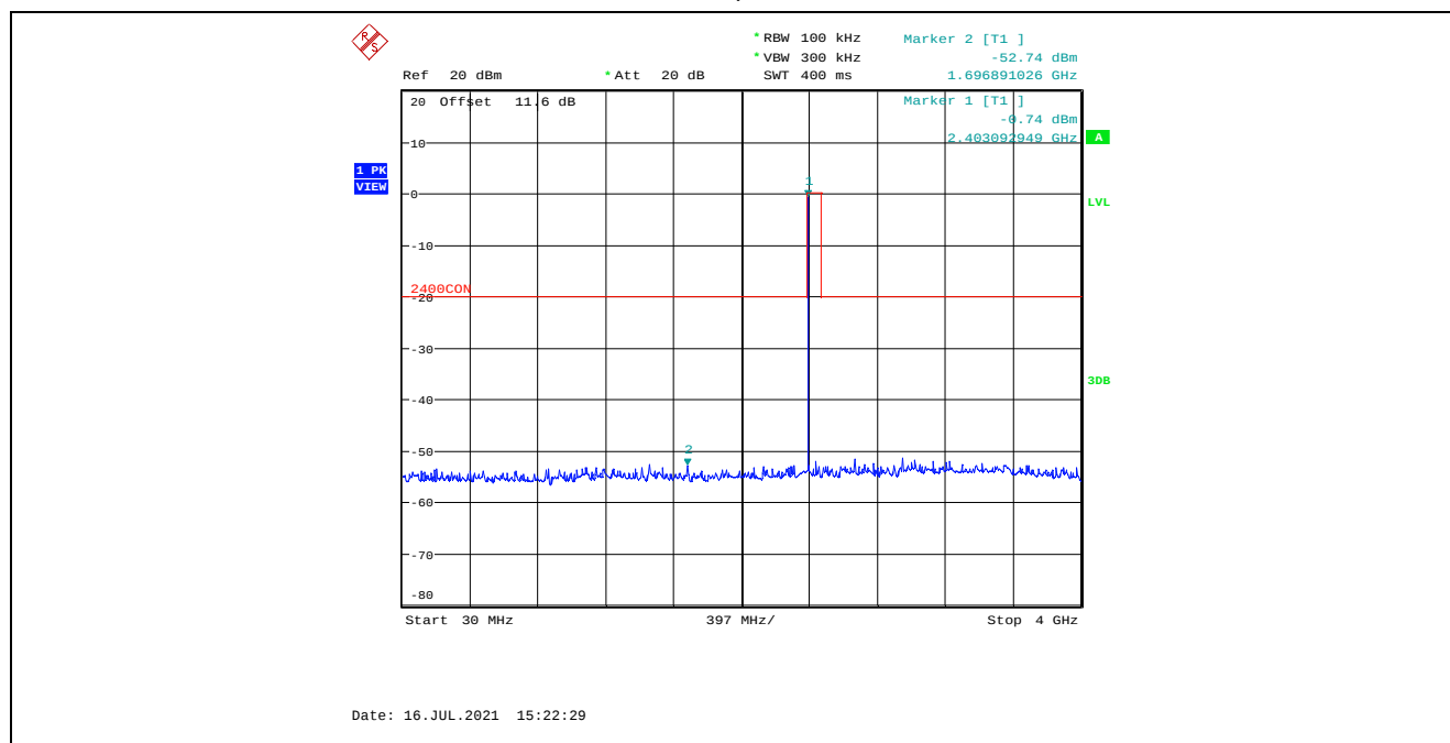
Plot 5.4.4.2.10. Conducted Spurious Emissions in Non-Restricted Frequency Bands, Low Power 2402 MHz, GFSK Modulation, 1 Mbps, 30 MHz – 4 GHz, Peak Detector
