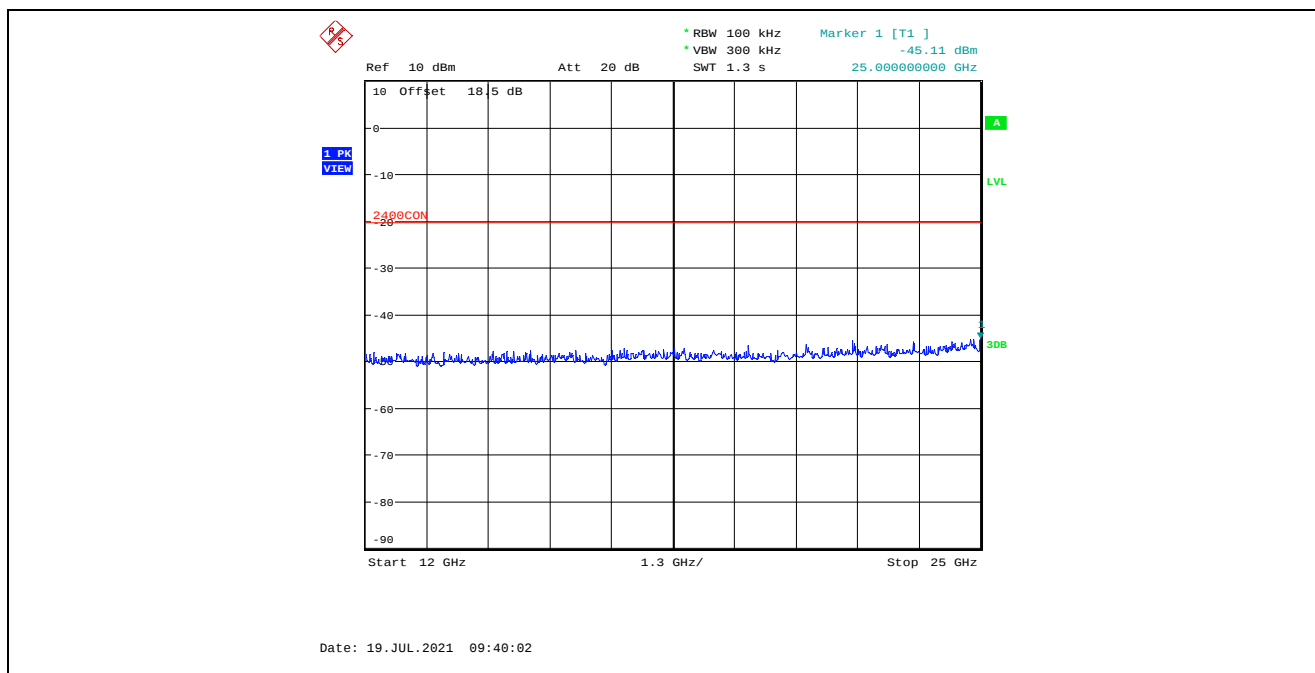
Plot 5.4.4.2.33. Conducted Spurious Emissions in Non-Restricted Frequency Bands, Low Power 2440 MHz, GFSK Modulation, 2 Mbps, 12 GHz – 25 GHz, Peak Detector
