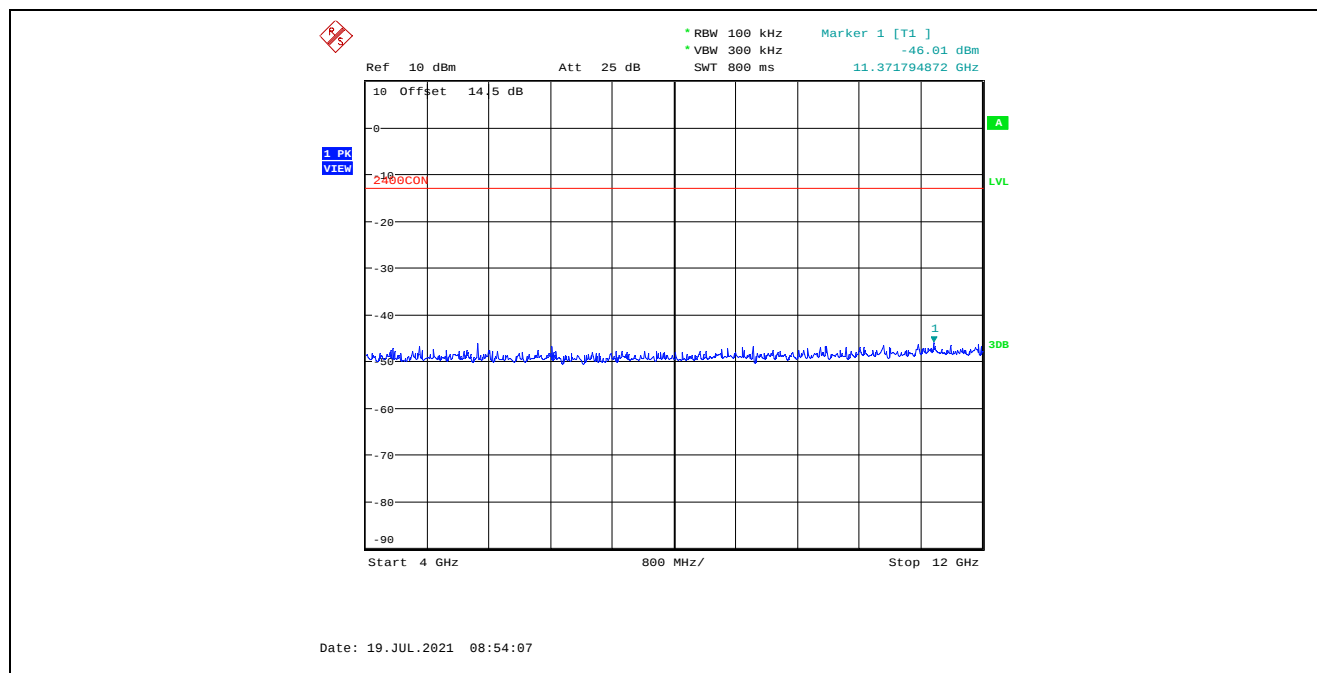
Plot 5.4.4.2.5. Conducted Spurious Emissions in Non-Restricted Frequency Bands, High Power 2440 MHz, GFSK Modulation, 1 Mbps, 4 GHz – 12 GHz, Peak Detector
