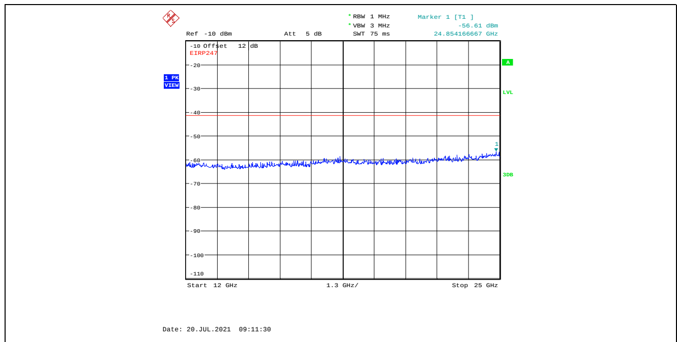
Plot 5.4.4.3.6. Conducted Spurious Emissions in Restricted Frequency Bands, High Power 2402 MHz, GFSK Modulation, 1 Mbps, 12 GHz - 25 GHz, Peak Detector
