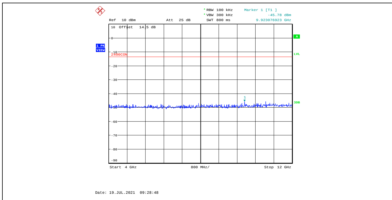
Plot 5.4.4.2.23. Conducted Spurious Emissions in Non-Restricted Frequency Bands, High Power 2440 MHz, GFSK Modulation, 2 Mbps, 4 GHz – 12 GHz, Peak Detector
