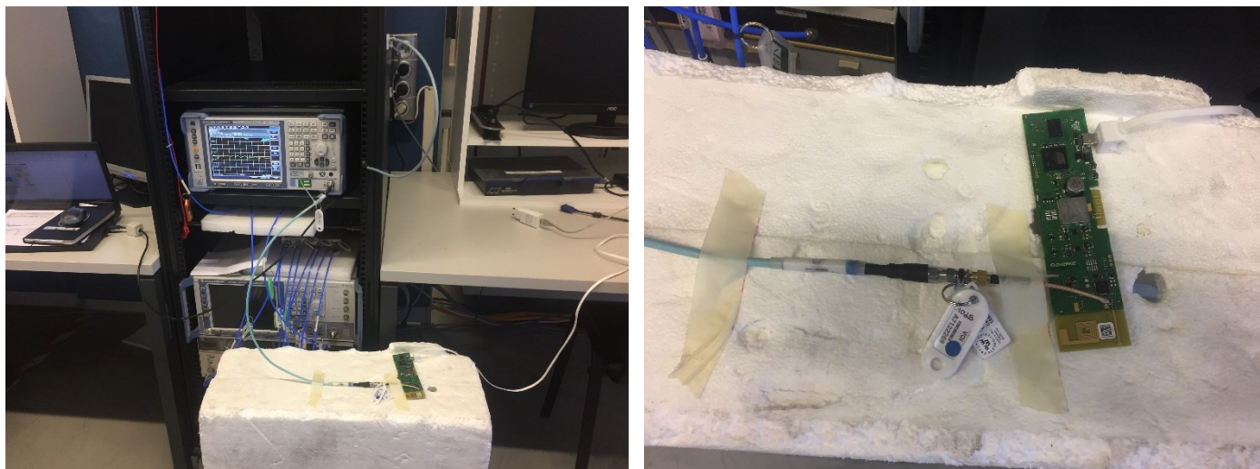
Photograph for Unwanted Emission into non-restricted frequency bands at the band edge
