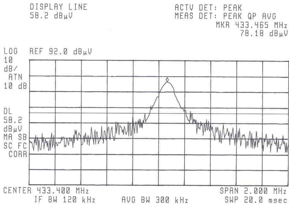
Figure 5.2 Occupied Bandwidth
