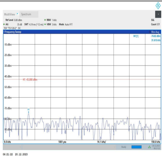
2-2-10MHz-20MHz-64QAM-64QAM-18655-18799-50RB#0-10 ORB#0-0.009~0.15MHz-PASS
