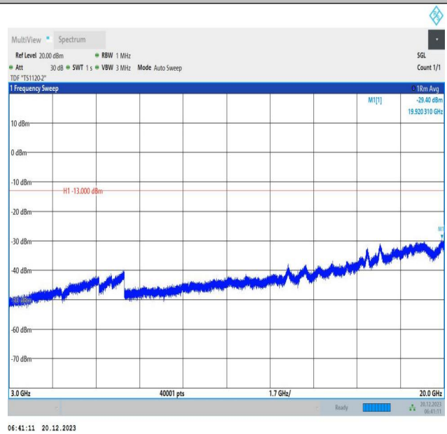
2-2-10MHz-20MHz-16QAM-16QAM-18806-18950-1RB#0-1RB #99-3000~20000MHz-PASS
