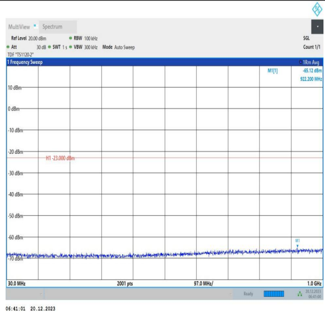
2-2-10MHz-20MHz-16QAM-16QAM-18806-18950-1RB#0-1RB #99-30~1000MHz-PASS
