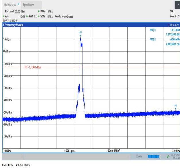
2-2-10MHz-20MHz-QPSK-QPSK-18806-18950-50RB#0-100R B#0-1000~3000MHz-PASS
