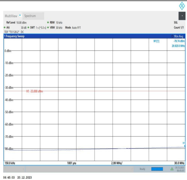
2-2-10MHz-20MHz-16QAM-16QAM-18806-18950-50RB#0-10 ORB#0-0.15~30MHz-PASS
