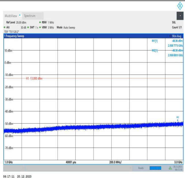
2-2-10MHz-20MHz-64QAM-64QAM-18655-18799-1RB#0-1RB #99-1000~3000MHz-PASS
