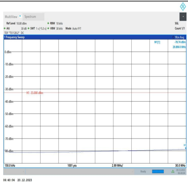
2-2-10MHz-20MHz-QPSK-QPSK-18806-18950-1RB#0-1RB#9 9-0.15~30MHz-PASS
