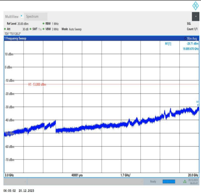
2-2-10MHz-20MHz-64QAM-64QAM-18655-18799-1RB#49-0R B#0-3000~20000MHz-PASS
