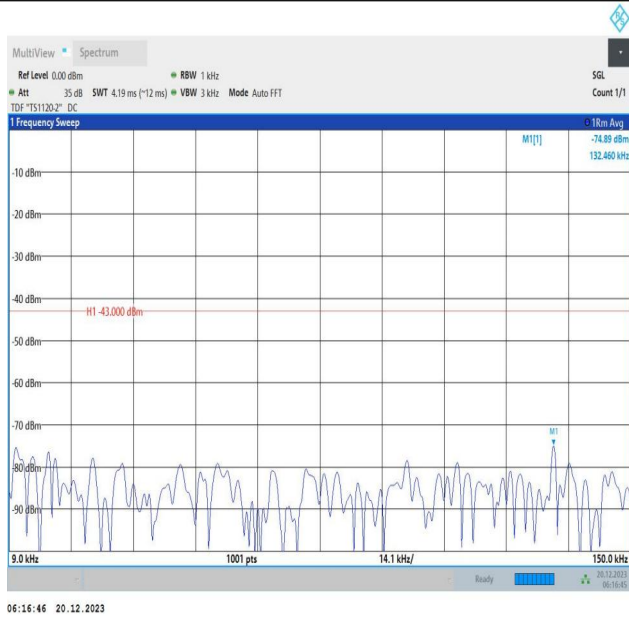
2-2-10MHz-20MHz-64QAM-64QAM-18655-18799-1RB#0-1RB #99-0.009~0.15MHz-PASS
