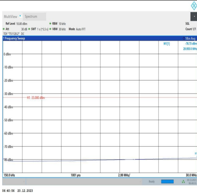
2-2-10MHz-20MHz-16QAM-16QAM-18806-18950-1RB#0-1RB #99-0.15~30MHz-PASS
