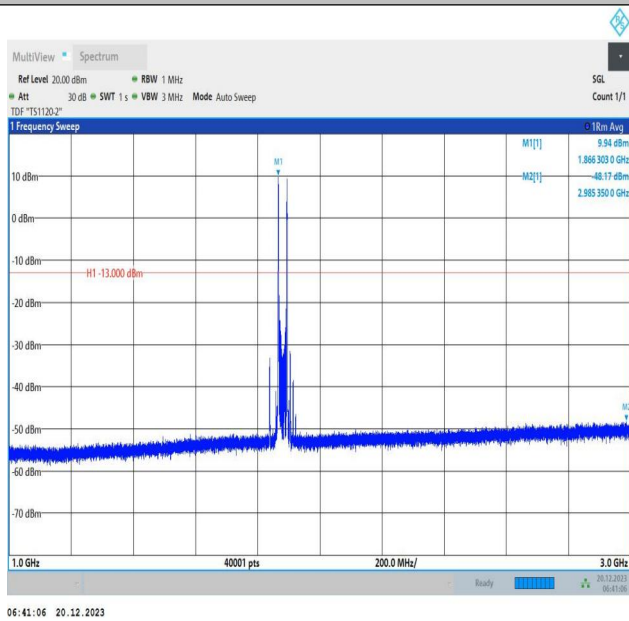
2-2-10MHz-20MHz-16QAM-16QAM-18806-18950-1RB#0-1RB #99-1000~3000MHz-PASS
