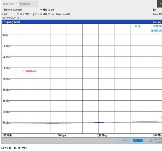
2-2-10MHz-15MHz-64QAM-64QAM-19005-19125-50RB#0-75 RB#0-0.15~30MHz-PASS
