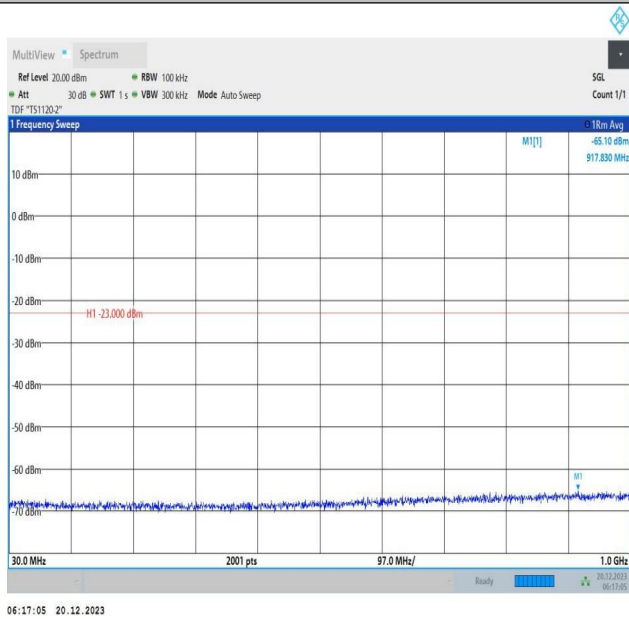
2-2-10MHz-20MHz-64QAM-64QAM-18655-18799-1RB#0-1RB #99-30~1000MHz-PASS
