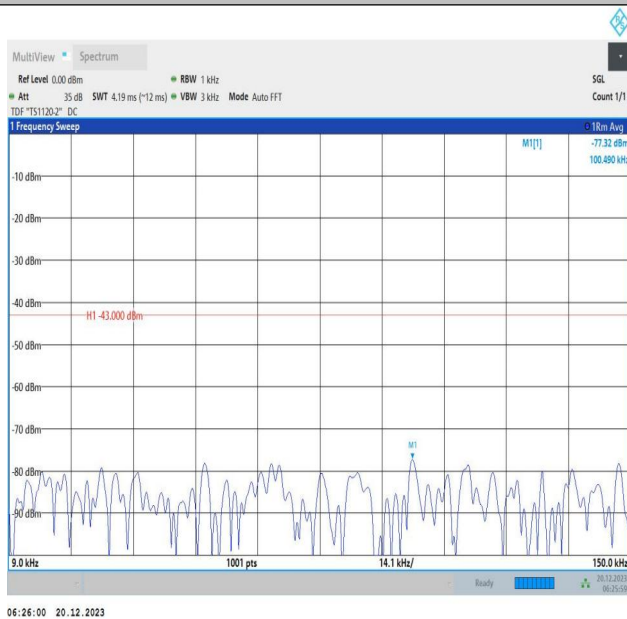
2-2-10MHz-20MHz-64QAM-64QAM-18806-18950-1RB#0-0RB #0-0.009~0.15MHz-PASS
