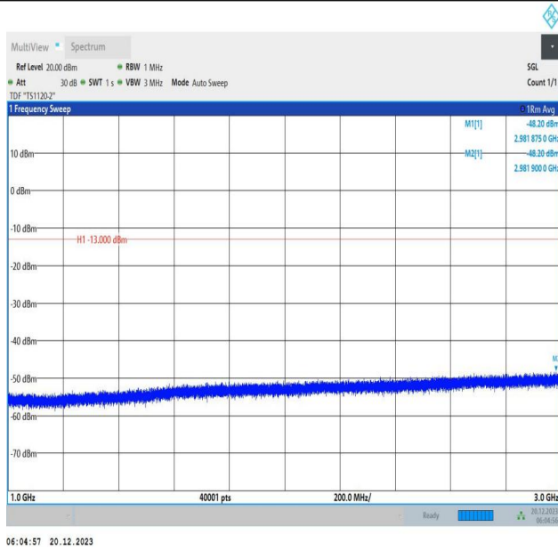
2-2-10MHz-20MHz-64QAM-64QAM-18655-18799-1RB#49-0R B#0-1000~3000MHz-PASS
