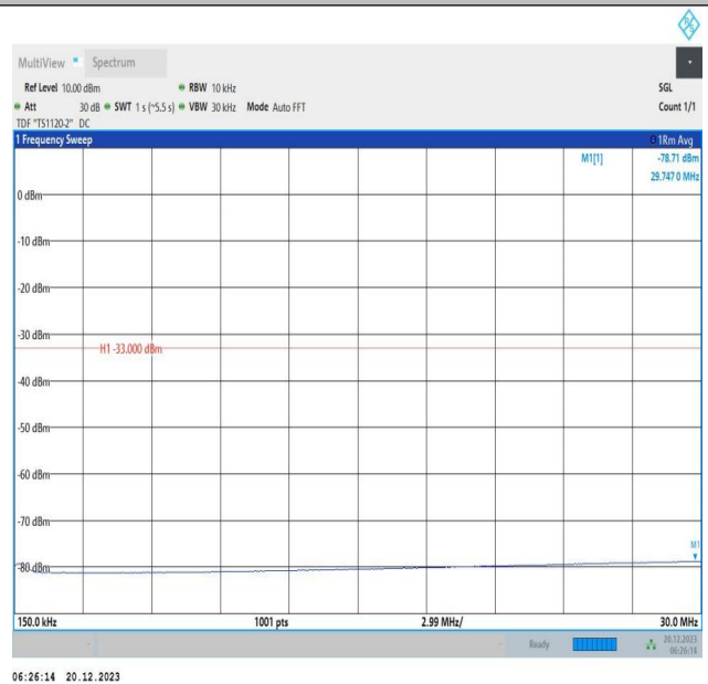
2-2-10MHz-20MHz-64QAM-64QAM-18806-18950-1RB#0-0RB #0-0.15~30MHz-PASS
