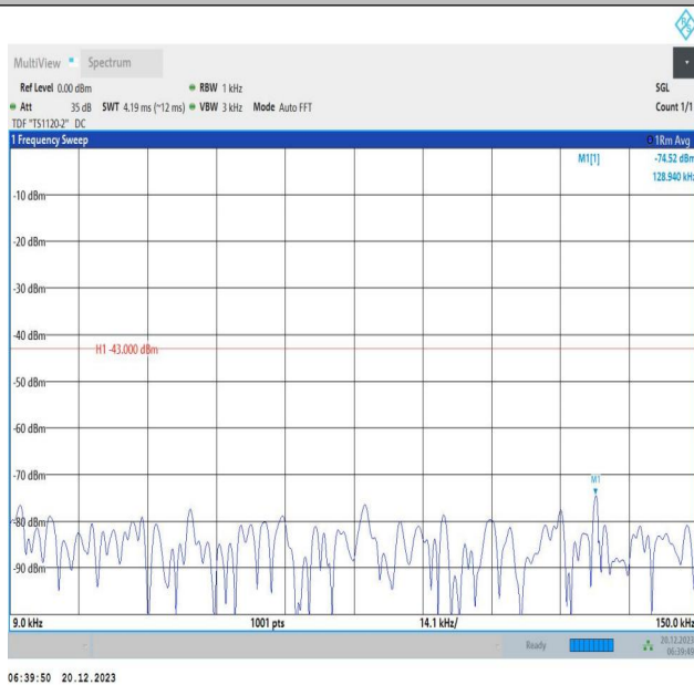
2-2-10MHz-20MHz-QPSK-QPSK-18806-18950-1RB#0-1RB#9 9-0.009~0.15MHz-PASS
