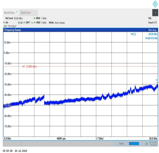
2-2-10MHz-15MHz-64QAM-64QAM-19005-19125-50RB#0-75 RB#0-3000~20000MHz-PASS
