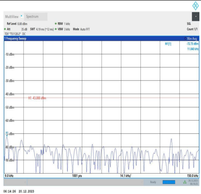
2-2-10MHz-20MHz-16QAM-16QAM-18655-18799-1RB#0-1RB #99-0.009~0.15MHz-PASS
