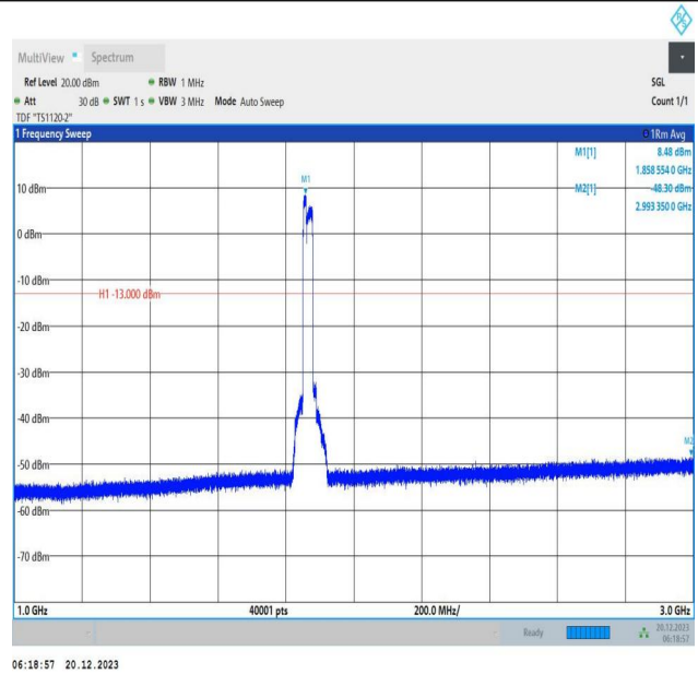
2-2-10MHz-20MHz-16QAM-16QAM-18655-18799-50RB#0-10 ORB#0-1000~3000MHz-PASS
