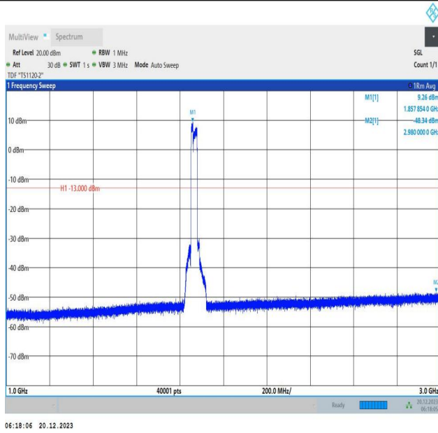
2-2-10MHz-20MHz-QPSK-QPSK-18655-18799-50RB#0-100R B#0-1000~3000MHz-PASS
