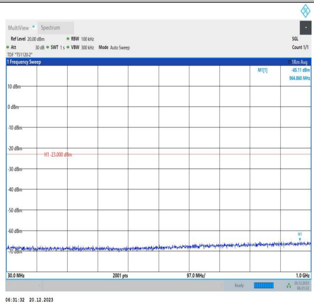
2-2-10MHz-20MHz-64QAM-64QAM-18806-18950-1RB#49-0R B#0-30~1000MHz-PASS
