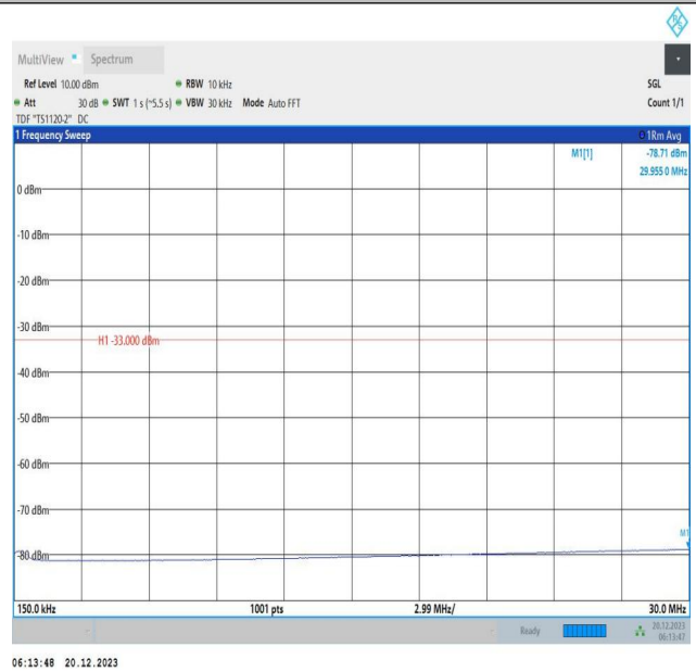
2-2-10MHz-20MHz-QPSK-QPSK-18655-18799-1RB#0-1RB#9 9-0.15~30MHz-PASS
