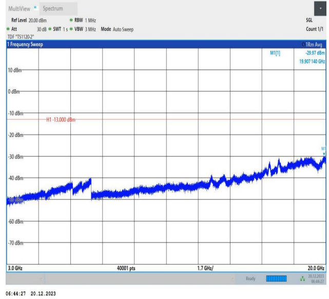
2-2-10MHz-20MHz-QPSK-QPSK-18806-18950-50RB#0-100R B#0-3000~20000MHz-PASS
