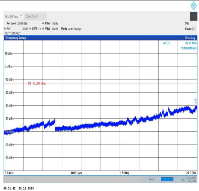
2-2-10MHz-20MHz-64QAM-64QAM-18806-18950-1RB#49-0R B#0-3000~20000MHz-PASS
