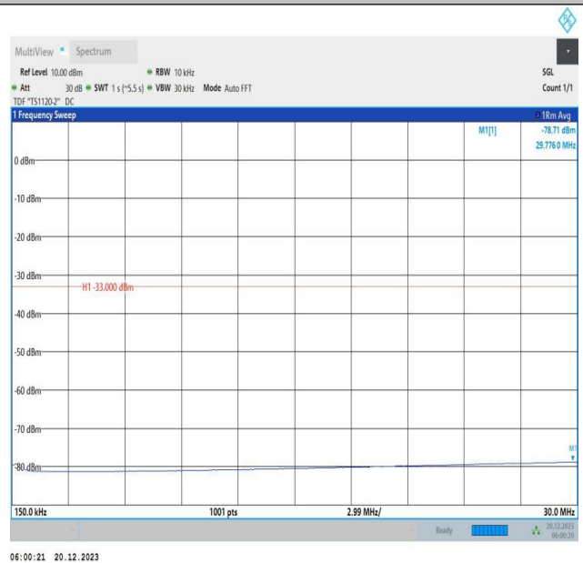
2-2-10MHz-20MHz-64QAM-64QAM-18655-18799-1RB#0-0RB #0-0.15~30MHz-PASS
