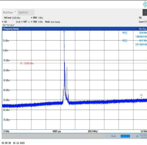
2-2-10MHz-20MHz-16QAM-16QAM-18655-18799-1RB#0-0RB #0-1000~3000MHz-PASS
