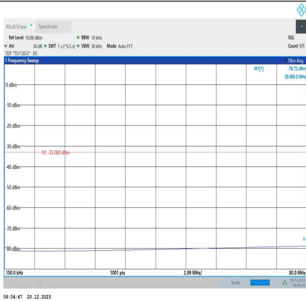
2-2-10MHz-20MHz-64QAM-64QAM-18655-18799-1RB#49-0R B#0-0.15~30MHz-PASS
