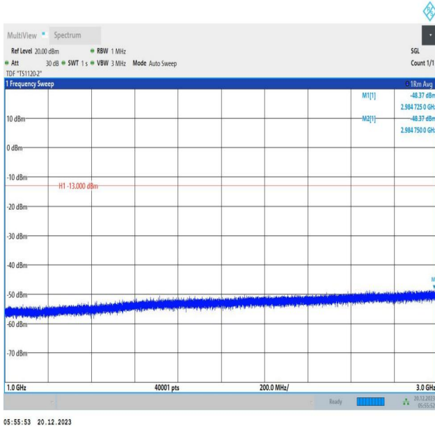
2-2-10MHz-15MHz-64QAM-64QAM-19005-19125-50RB#0-75 RB#0-1000~3000MHz-PASS
