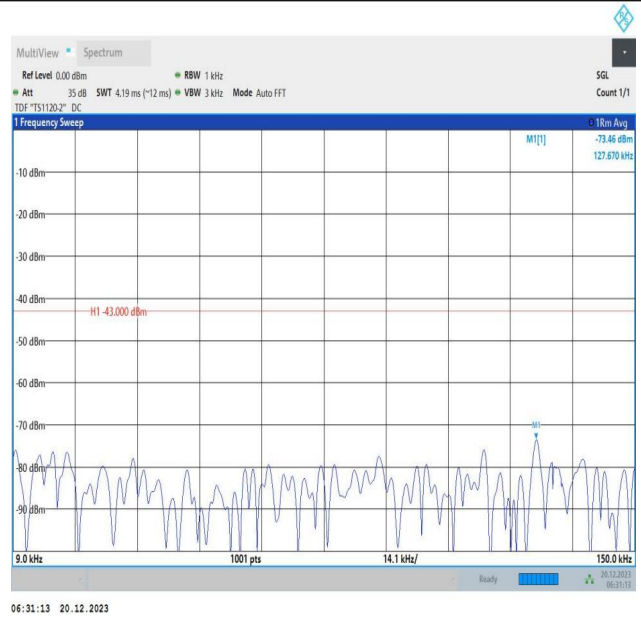
2-2-10MHz-20MHz-64QAM-64QAM-18806-18950-1RB#49-0R B#0-0.009~0.15MHz-PASS
