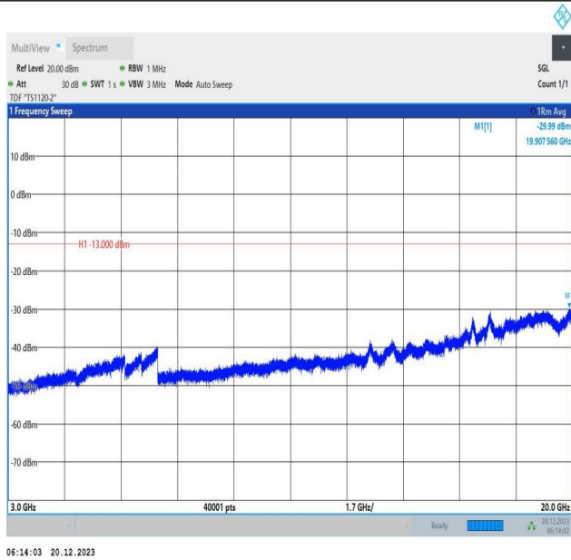
2-2-10MHz-20MHz-QPSK-QPSK-18655-18799-1RB#0-1RB#9 9-3000~20000MHz-PASS
