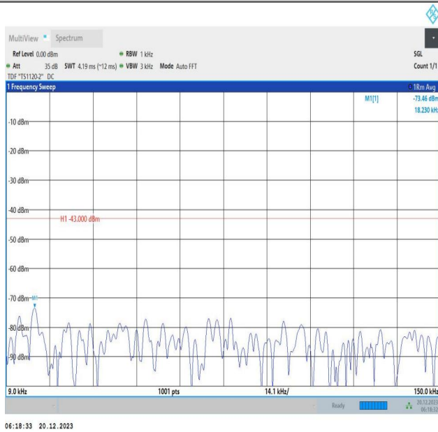
2-2-10MHz-20MHz-16QAM-16QAM-18655-18799-50RB#0-10 ORB#0-0.009~0.15MHz-PASS
