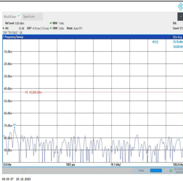
2-2-10MHz-20MHz-64QAM-64QAM-18655-18799-1RB#0-0RB #0-0.009~0.15MHz-PASS
