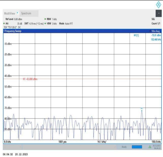
2-2-10MHz-20MHz-64QAM-64QAM-18655-18799-1RB#49-0R B#0-0.009~0.15MHz-PASS
