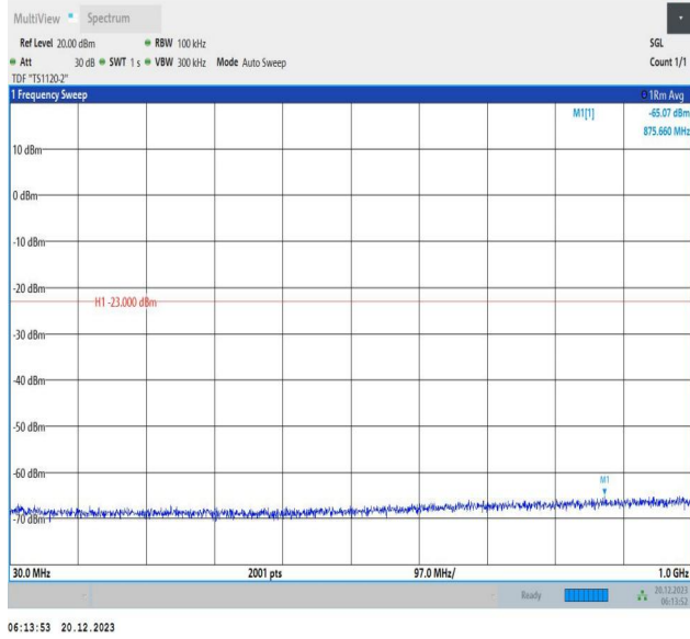
2-2-10MHz-20MHz-QPSK-QPSK-18655-18799-1RB#0-1RB#9 9-30~1000MHz-PASS
