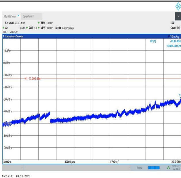
2-2-10MHz-20MHz-16QAM-16QAM-18655-18799-50RB#0-10 ORB#0-3000~20000MHz-PASS
