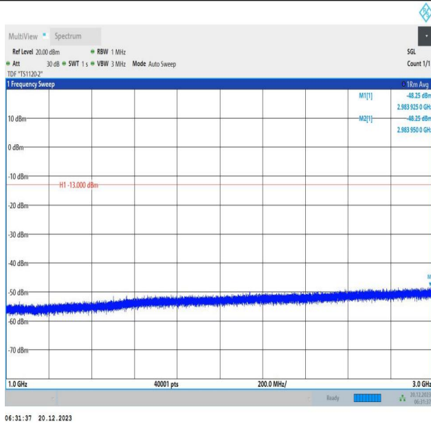
2-2-10MHz-20MHz-64QAM-64QAM-18806-18950-1RB#49-0R B#0-1000~3000MHz-PASS
