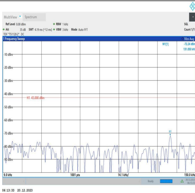
2-2-10MHz-20MHz-QPSK-QPSK-18655-18799-1RB#0-1RB#9 9-0.009~0.15MHz-PASS
