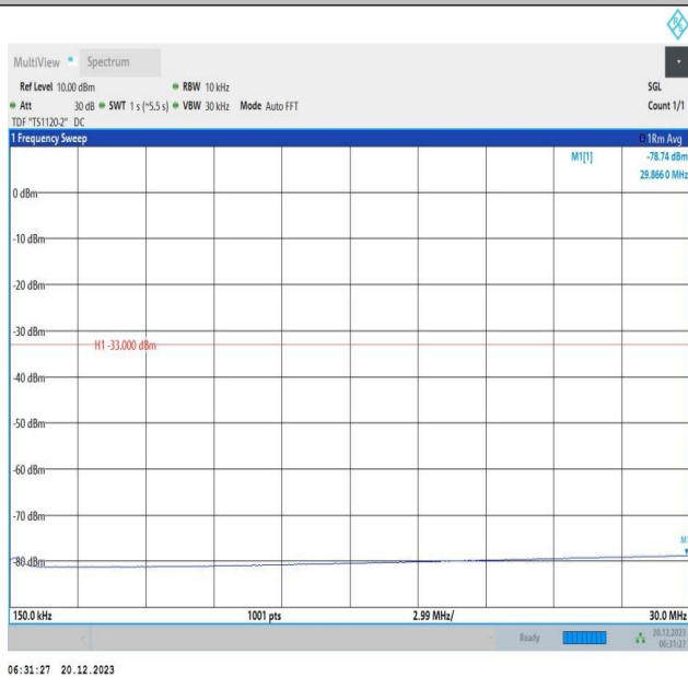
2-2-10MHz-20MHz-64QAM-64QAM-18806-18950-1RB#49-0R B#0-0.15~30MHz-PASS
