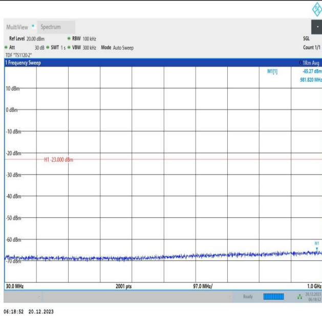
2-2-10MHz-20MHz-16QAM-16QAM-18655-18799-50RB#0-10 ORB#0-30~1000MHz-PASS
