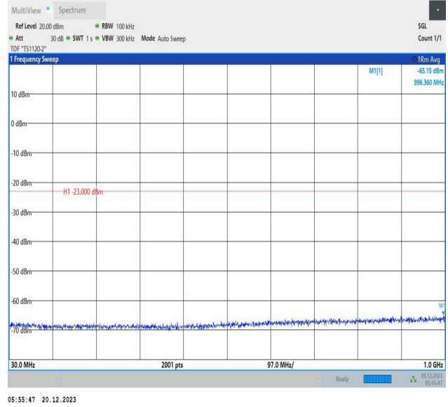
2-2-10MHz-15MHz-64QAM-64QAM-19005-19125-50RB#0-75 RB#0-30~1000MHz-PASS
