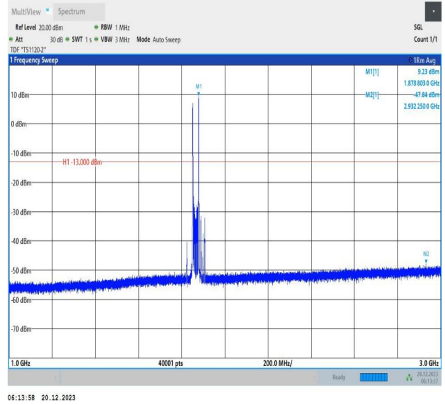
2-2-10MHz-20MHz-QPSK-QPSK-18655-18799-1RB#0-1RB#9 9-1000~3000MHz-PASS
