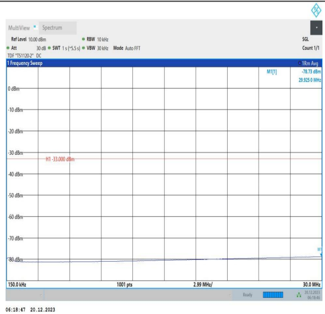
2-2-10MHz-20MHz-16QAM-16QAM-18655-18799-50RB#0-10 ORB#0-0.15~30MHz-PASS
