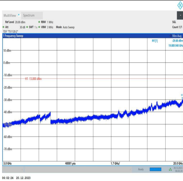
2-2-10MHz-20MHz-16QAM-16QAM-18655-18799-1RB#49-0R B#0-3000~20000MHz-PASS
