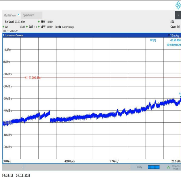
2-2-10MHz-20MHz-16QAM-16QAM-18806-18950-1RB#49-0R B#0-3000~20000MHz-PASS
