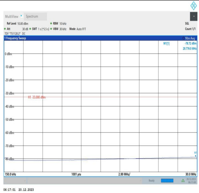
2-2-10MHz-20MHz-64QAM-64QAM-18655-18799-1RB#0-1RB #99-0.15~30MHz-PASS
