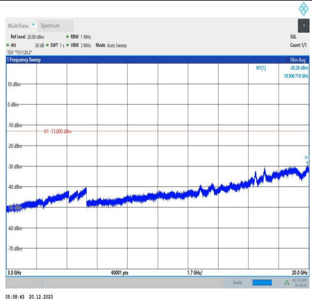
2-2-10MHz-20MHz-16QAM-16QAM-18655-18799-1RB#0-0RB #0-3000~20000MHz-PASS
