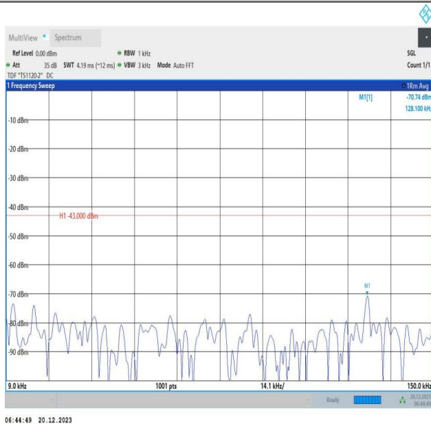
2-2-10MHz-20MHz-16QAM-16QAM-18806-18950-50RB#0-10 ORB#0-0.009~0.15MHz-PASS
