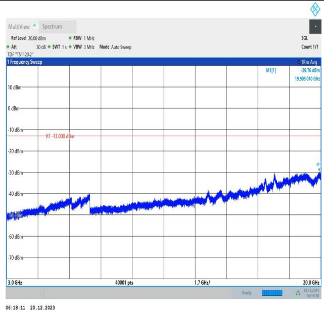
2-2-10MHz-20MHz-QPSK-QPSK-18655-18799-50RB#0-100R B#0-3000~20000MHz-PASS
