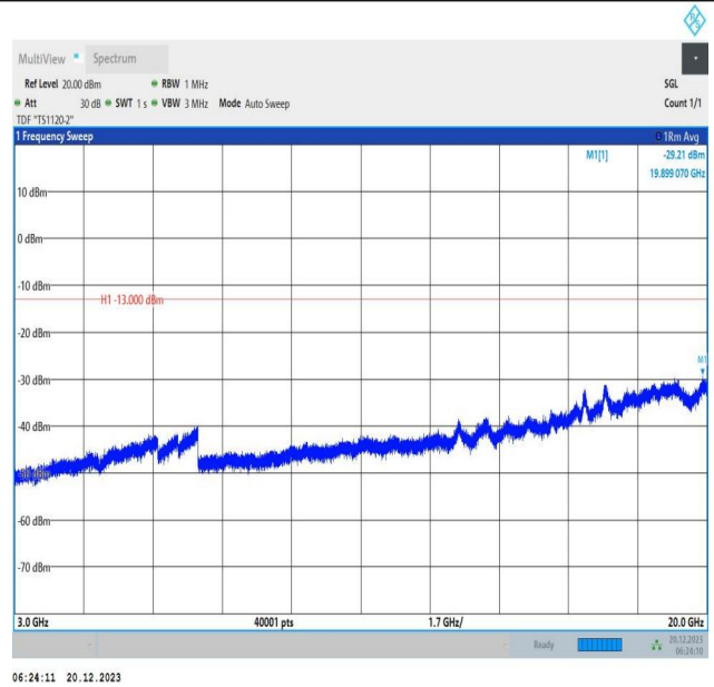
2-2-10MHz-20MHz-16QAM-16QAM-18806-18950-1RB#0-0RB #0-3000~20000MHz-PASS
