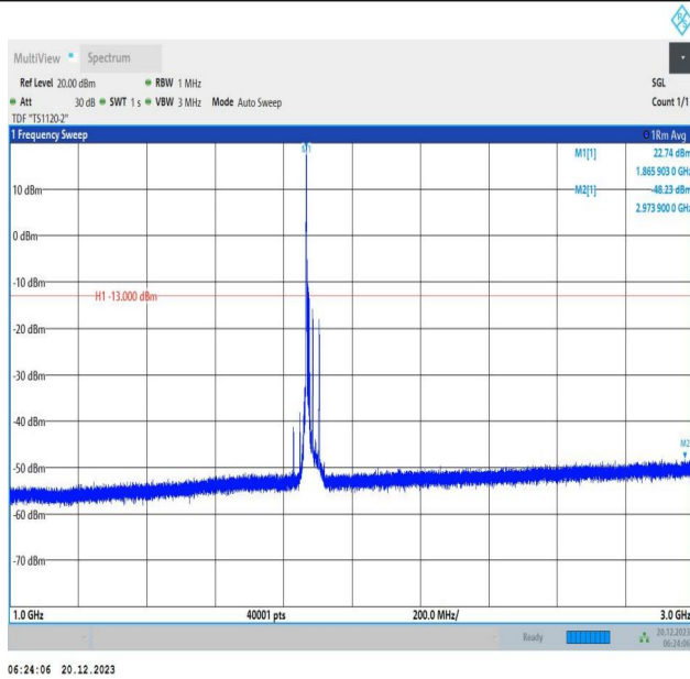
2-2-10MHz-20MHz-16QAM-16QAM-18806-18950-1RB#0-0RB #0-1000~3000MHz-PASS
