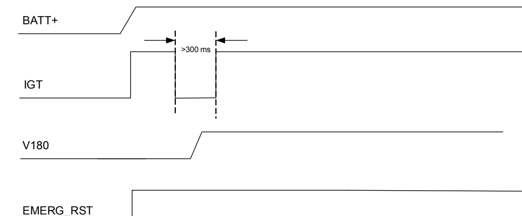
Figure 23: IGT timing
