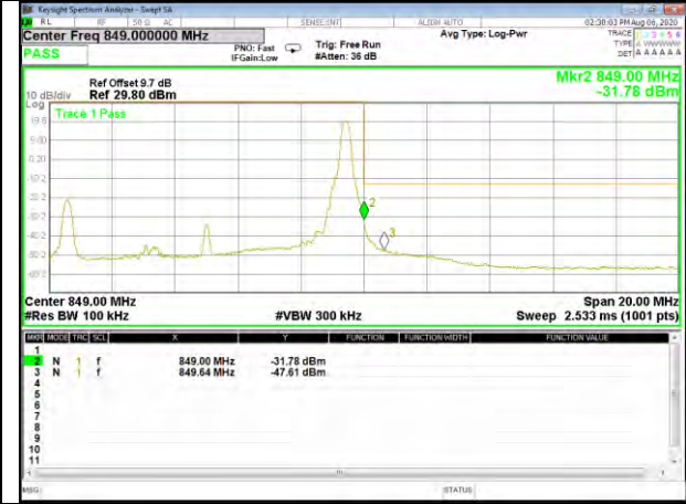
Band5_10M_QPSK_High_1-RB
