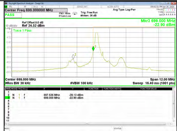
Band12_1.4M_QPSK_Low_Full-RB
