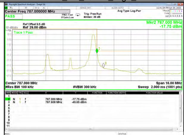
Band13_5M_QPSK_High_1-RB
