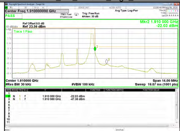
Band2_3M_16QAM_High_1-RB
