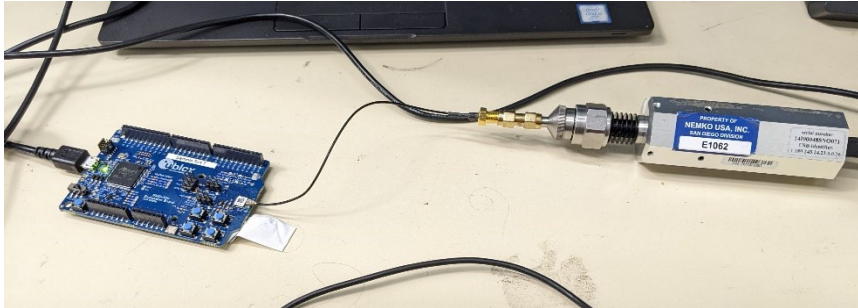
Figure 7 – Test setup – conducted antenna port measurements
