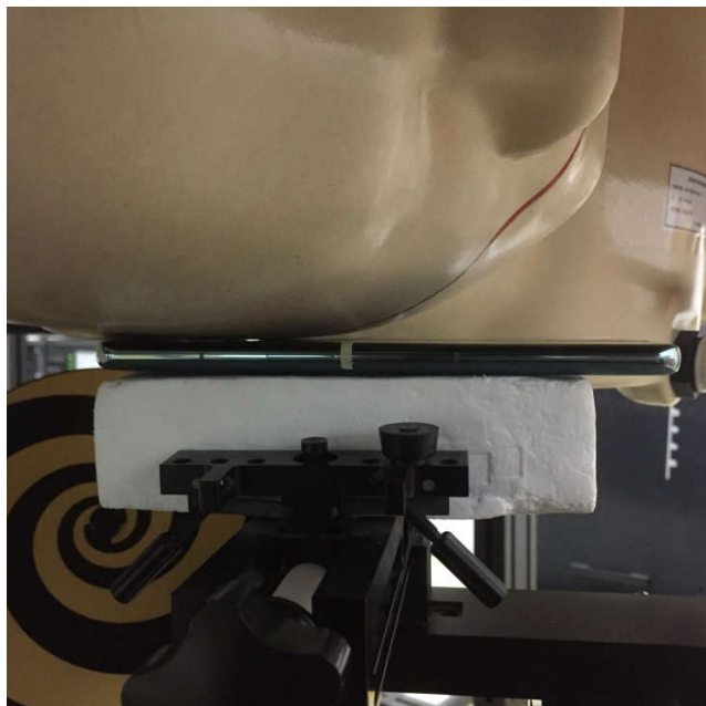
Right Cheek, Test Separation 0 mm
