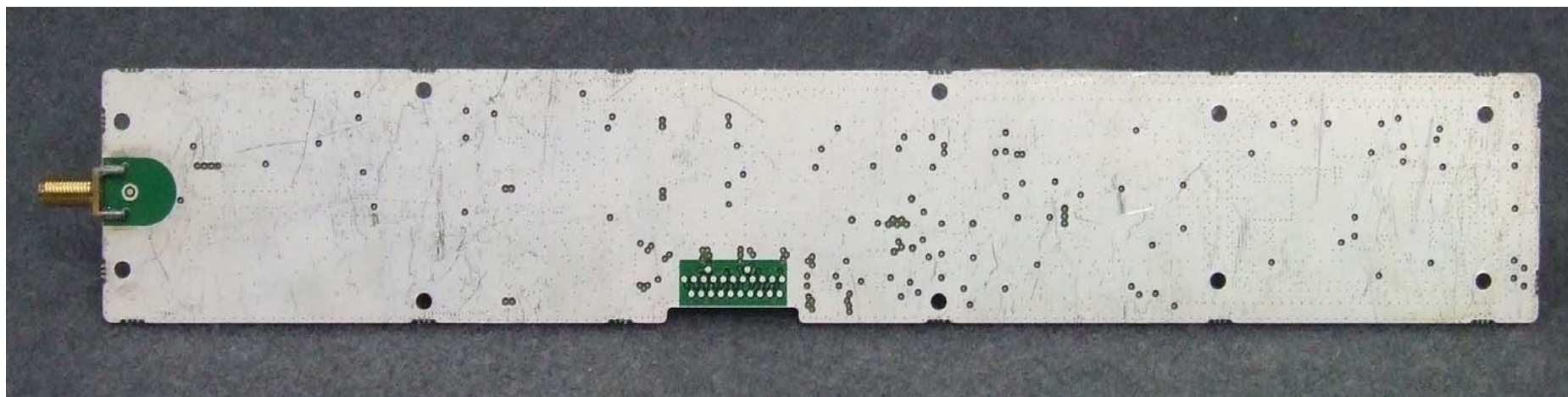
Photograph 12: TXF PCB – Bottom.
