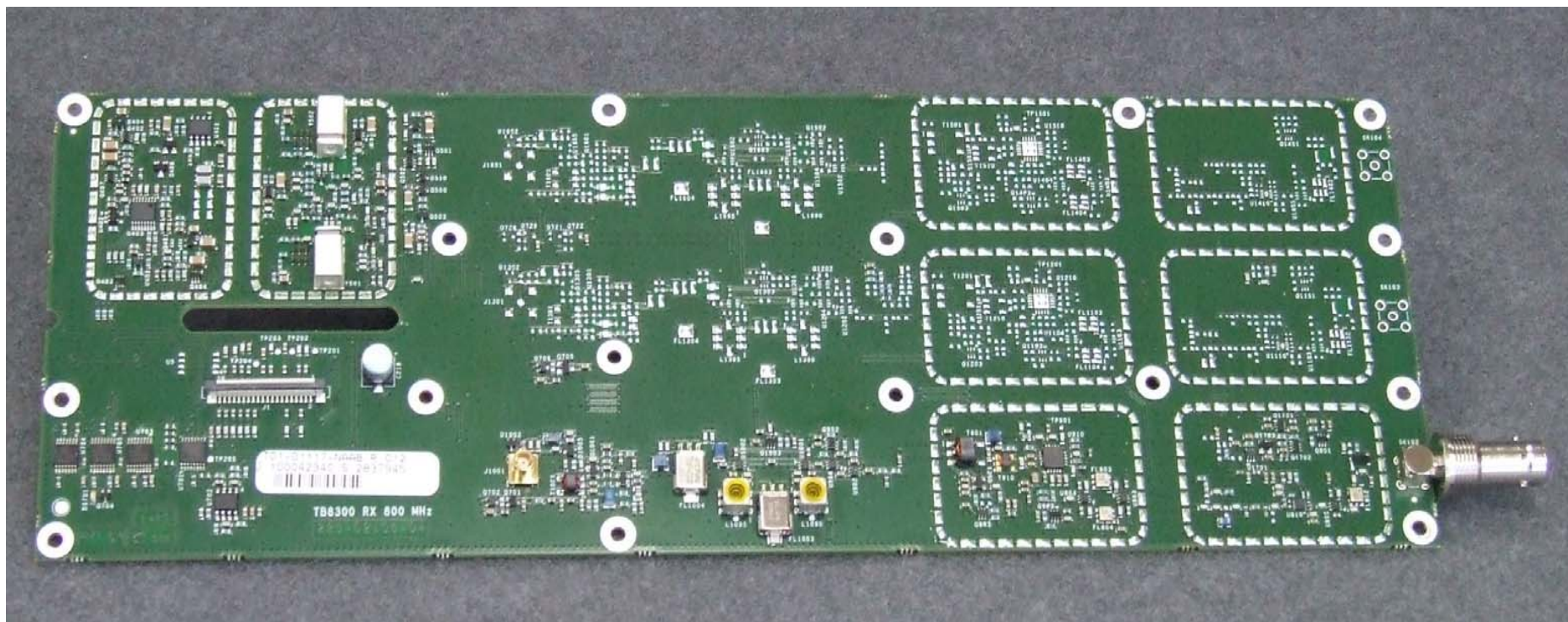
Photograph 05: Rx PCB – Top. Shields Removed
