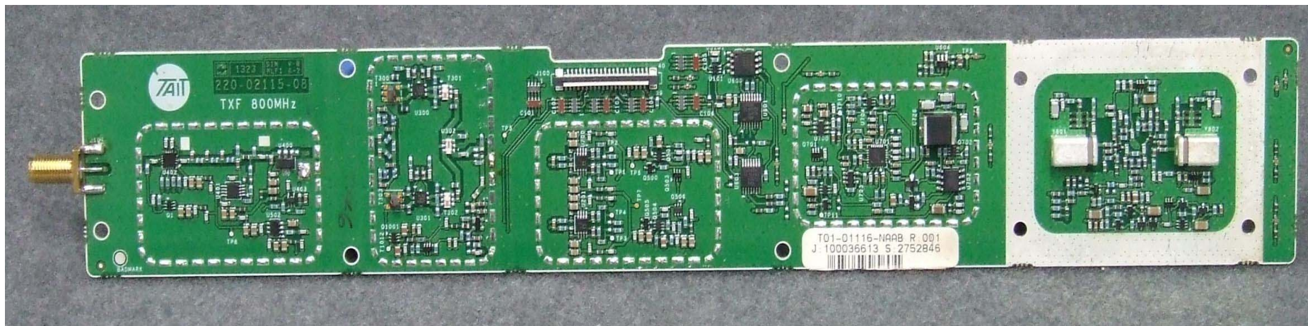
Photograph 11: TXF PCB – Top. Shields Removed
