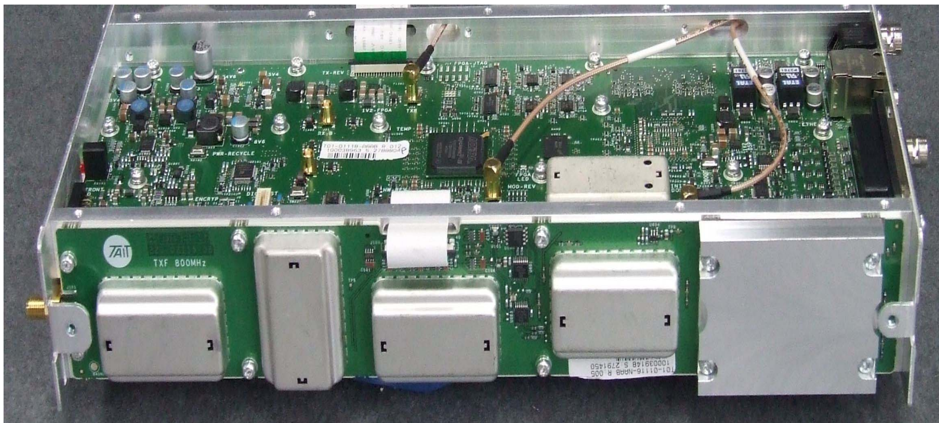
Photograph 10: TXF PCB – Top
