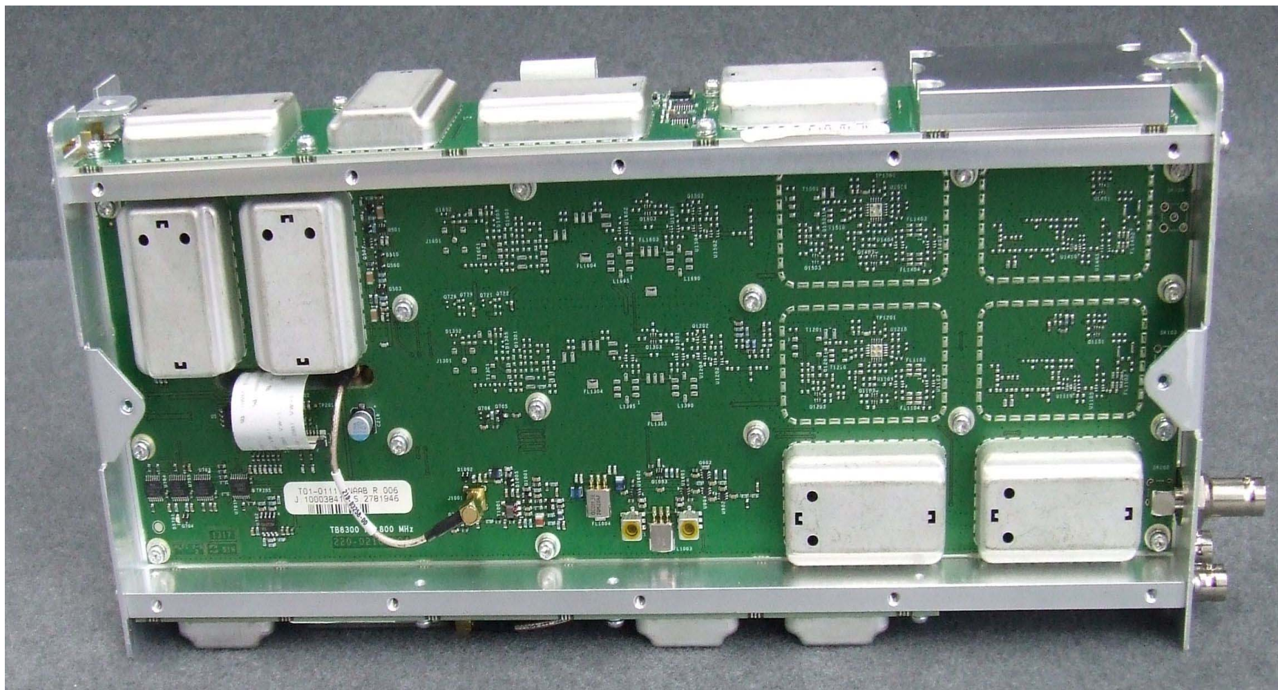
Photograph 04: Rx PCB - Top
