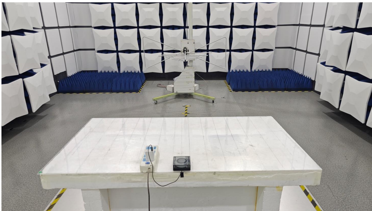
Radiated Emission Below 1GHz
