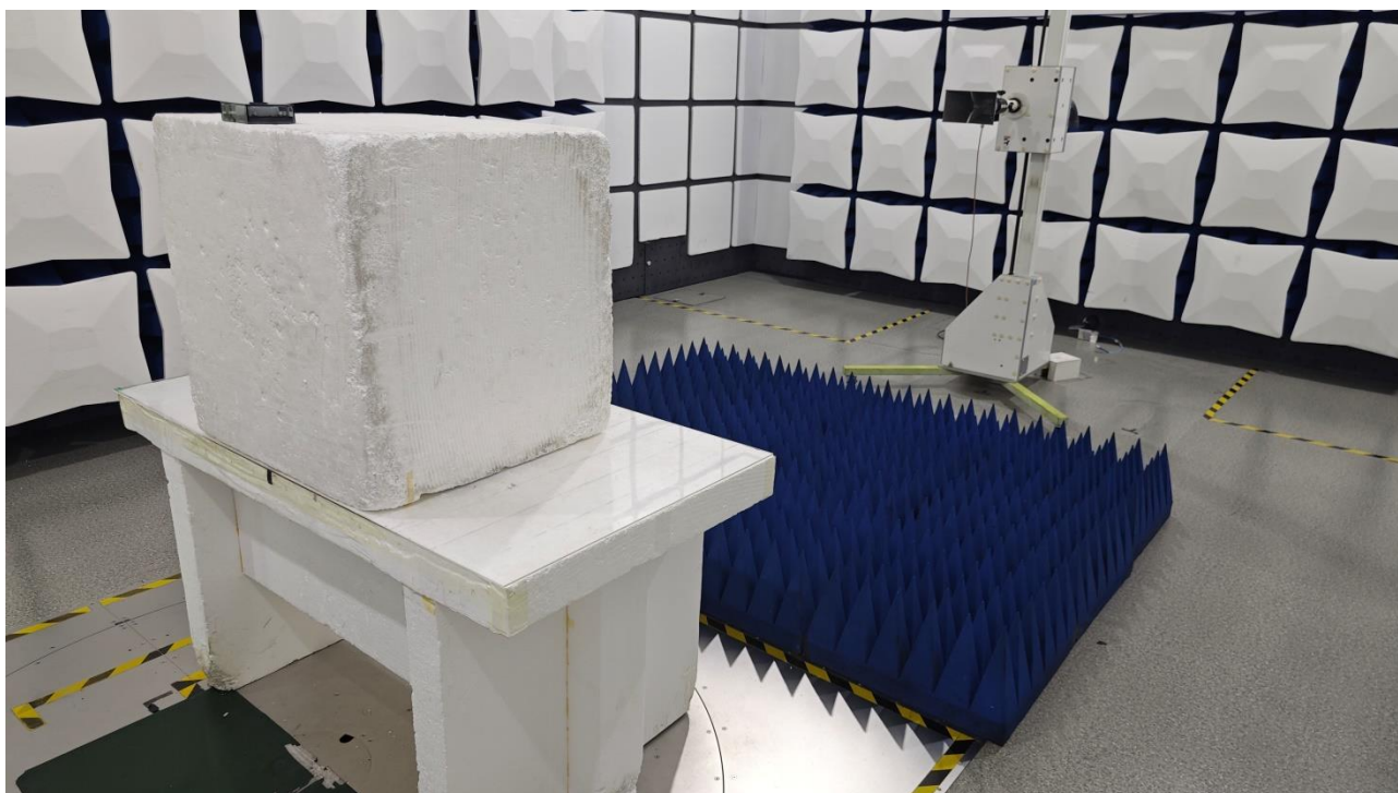
Radiated Emission Above 1GHz
