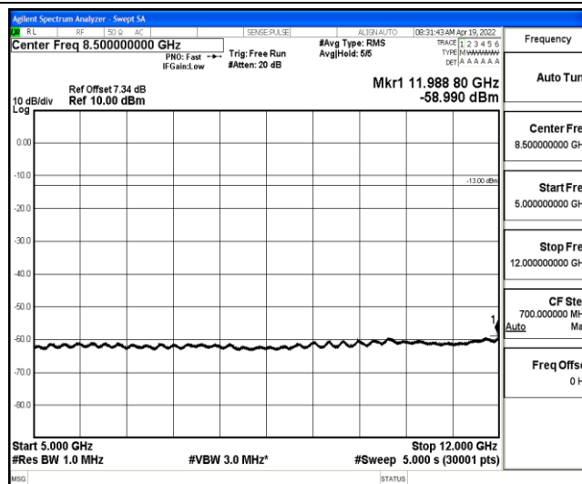
Band5-1.4MHz-16QAM-20643-1-0-High-5000-12000--58.99-PASS
