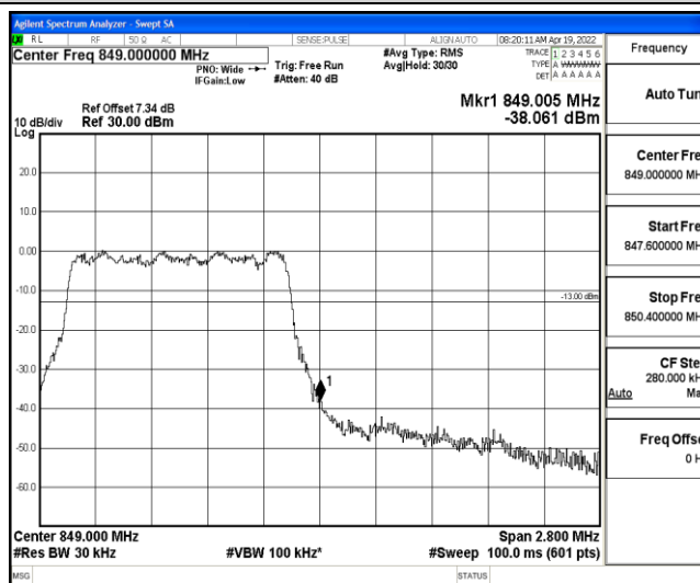
Band5-1.4MHz-16QAM-20643-6-0-Low--38.06-PASS
