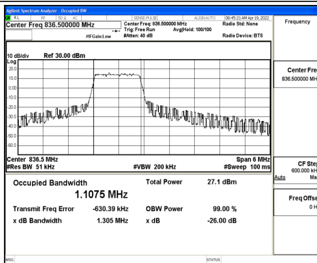
Band5-3MHz-QPSK-20525-6-0-Low-1.1075-1.305-PASS
