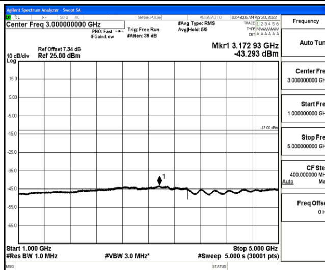
Band5-1.4MHz-16QAM-20525-1-0-Low-1000-5000--43.29-PASS
