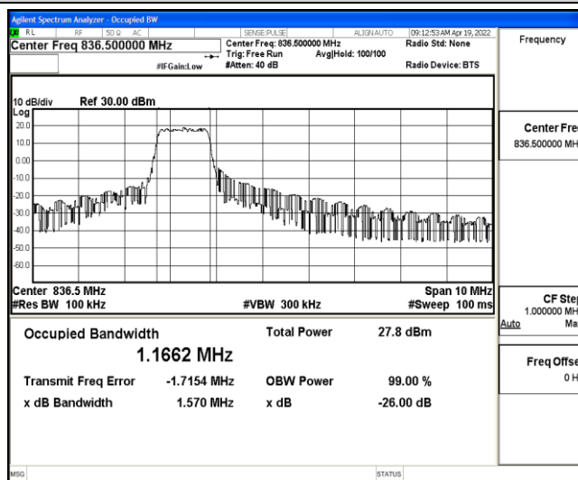
Band5-5MHz-QPSK-20525-6-0-Low-1.1662-1.570-PASS
