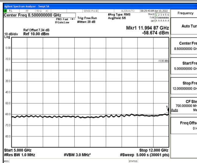
Band5-1.4MHz-QPSK-20643-1-0-High-5000-12000--58.67-PASS
