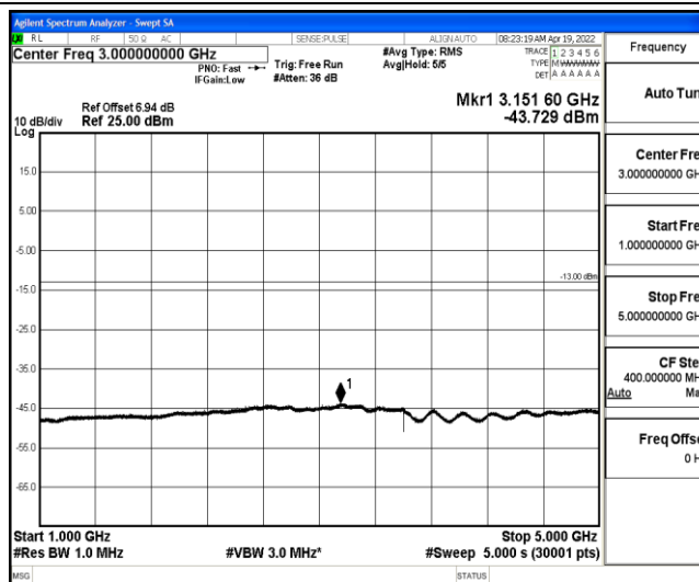
Band5-1.4MHz-16QAM-20407-1-0-Low-1000-5000--43.73-PASS
