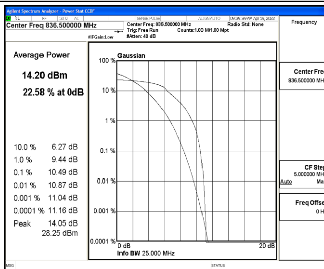
Band5-10MHz-16QAM-20525-6-0-Low-10.49-&lt;=13-PASS
