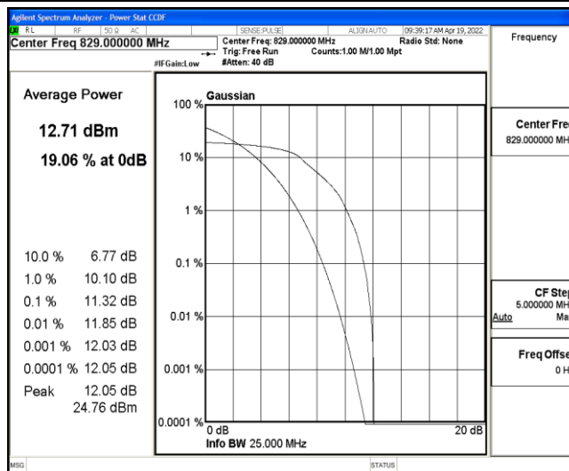
Band5-10MHz-16QAM-20450-6-0-Low-11.32-&lt;=13-PASS
