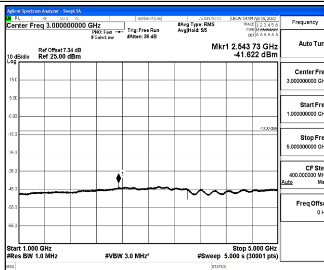
Band5-1.4MHz-QPSK-20643-1-0-High-1000-5000--41.62-PASS
