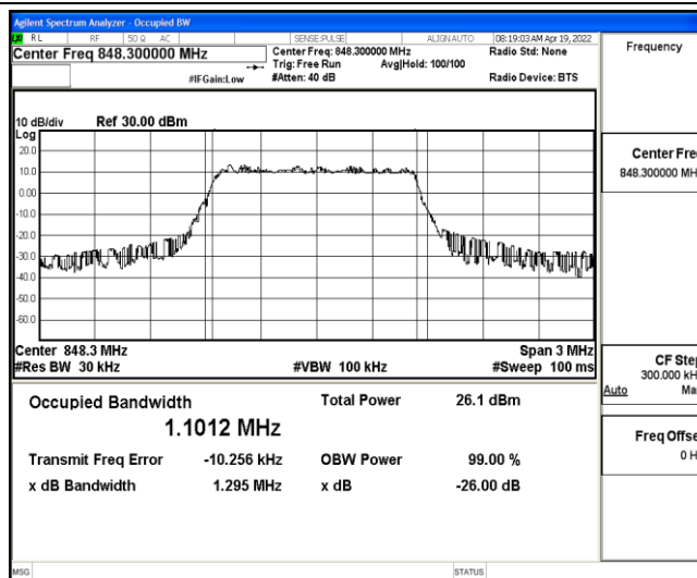
Band5-1.4MHz-QPSK-20643-6-0-High-1.1012-1.295-PASS
