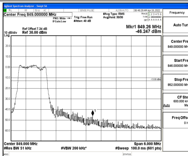
Band5-3MHz-16QAM-20635-6-0-Low--46.25-PASS
