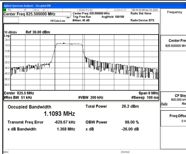
Band5-3MHz-QPSK-20415-6-0-Low-1.1093-1.368-PASS
