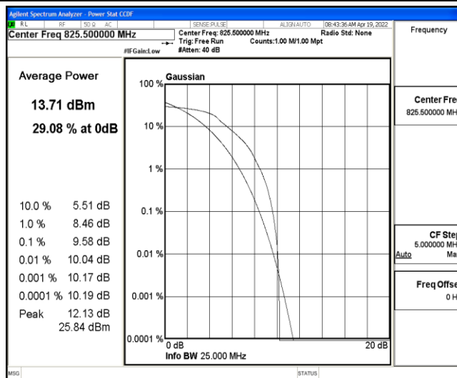
Band5-3MHz-16QAM-20415-6-0-Low-9.58-&lt;=13-PASS
