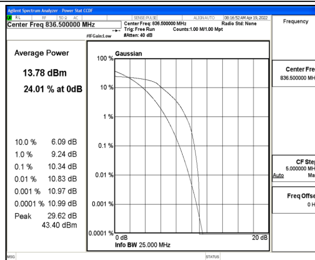
Band5-1.4MHz-16QAM-20525-6-0-Low-10.34-&lt;=13-PASS
