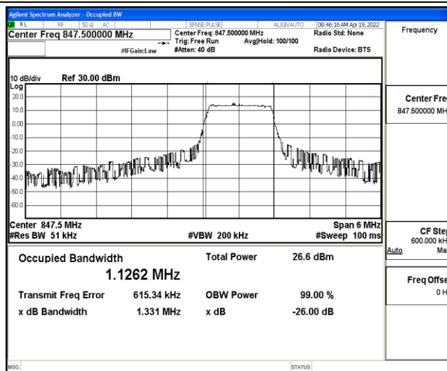
Band5-3MHz-16QAM-20635-6-0-High-1.1262-1.331-PASS
