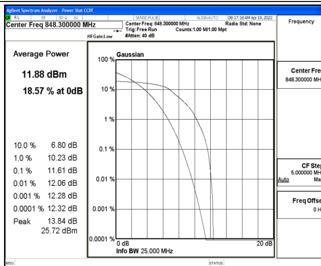
Band5-1.4MHz-16QAM-20643-6-0-Low-11.61-&lt;=13-PASS
