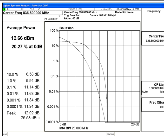
Band5-3MHz-16QAM-20525-6-0-Low-11.14-&lt;=13-PASS
