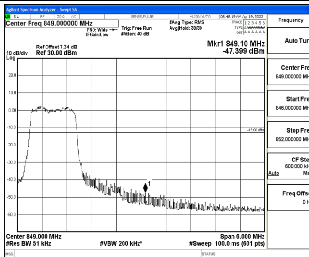
Band5-3MHz-QPSK-20635-6-0-Low--47.40-PASS
