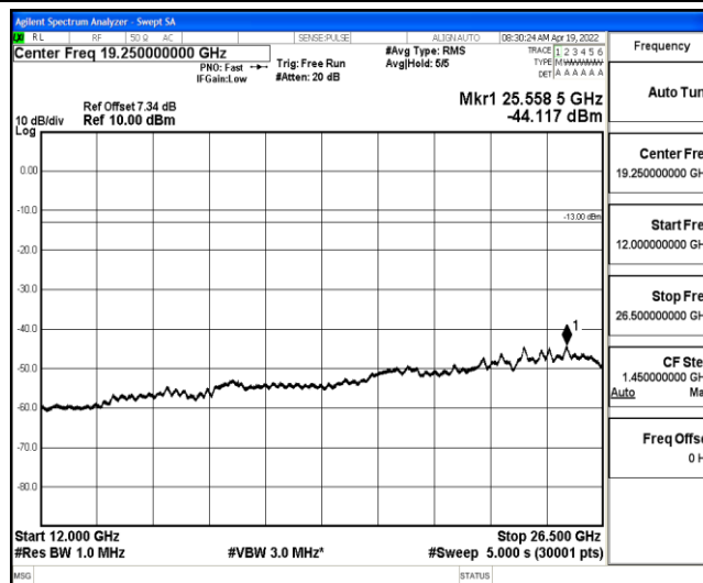
Band5-1.4MHz-QPSK-20643-1-0-High-12000-26500--44.12-PASS
