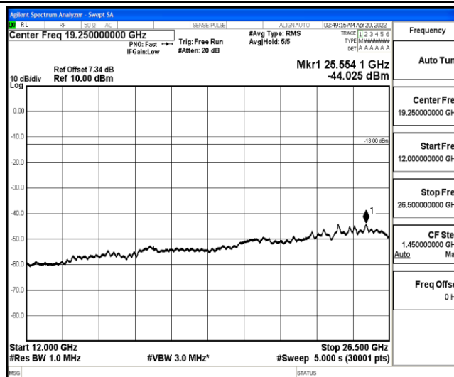
Band5-1.4MHz-16QAM-20525-1-0-Low-12000-26500--44.03-PASS
