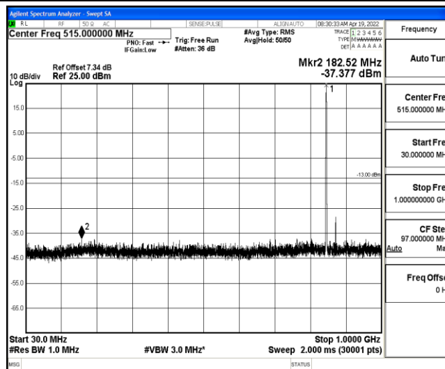
Band5-1.4MHz-16QAM-20643-1-0-High-30-1000--37.38-PASS
