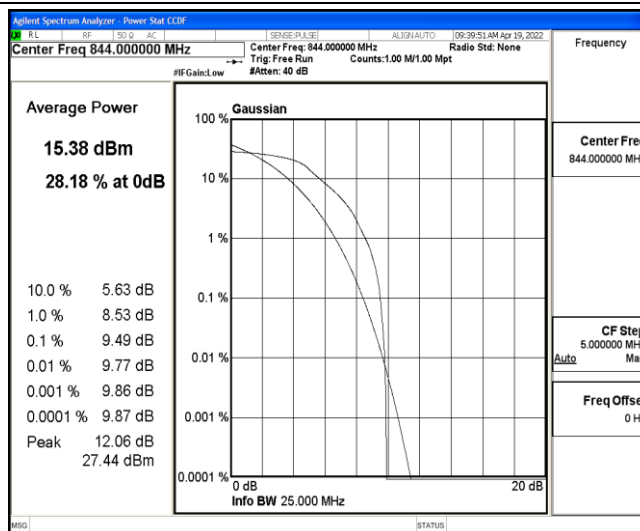
Band5-10MHz-QPSK-20600-6-0-Low-9.49-&lt;=13-PASS
