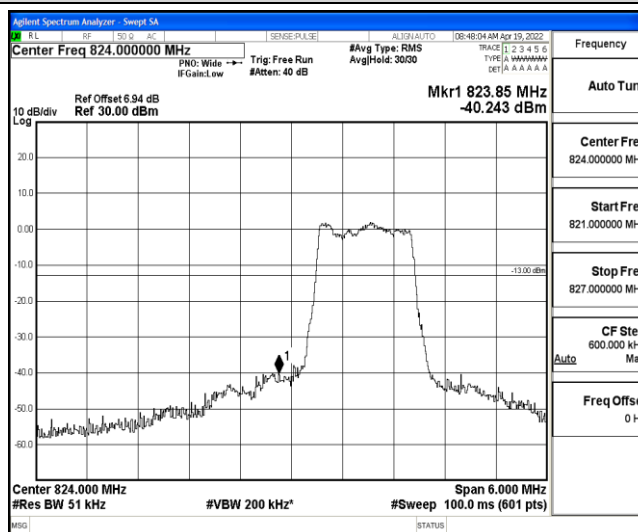
Band5-3MHz-16QAM-20415-6-0-Low--40.24-PASS
