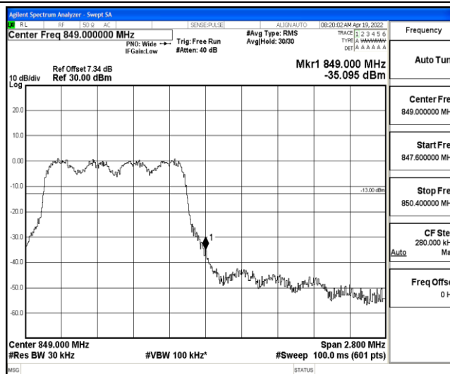
Band5-1.4MHz-QPSK-20643-6-0-Low--35.09-PASS
