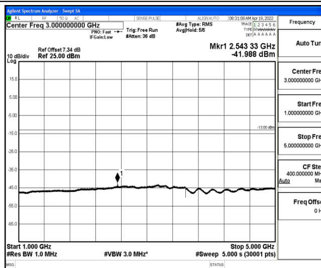
Band5-1.4MHz-16QAM-20643-1-0-High-1000-5000--41.99-PASS
