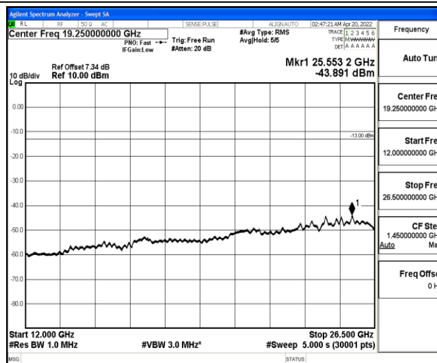
Band5-1.4MHz-QPSK-20525-1-0-Low-12000-26500--43.89-PASS
