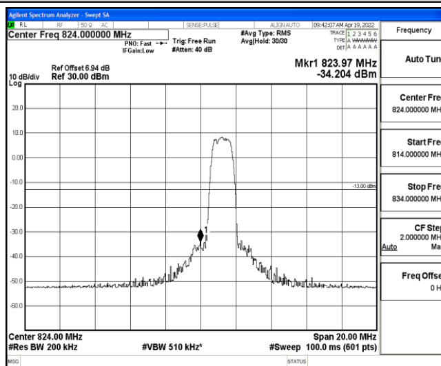
Band5-10MHz-QPSK-20450-6-0-Low--34.20-PASS
