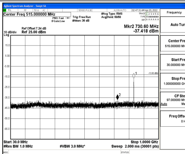
Band5-1.4MHz-16QAM-20525-1-0-Low-30-1000--37.42-PASS
