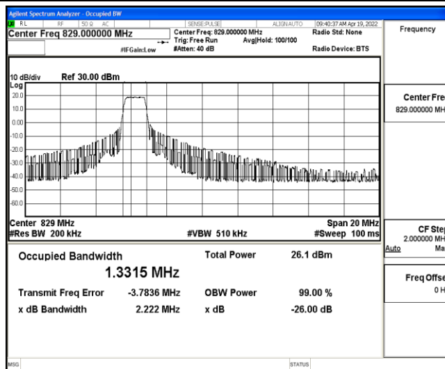
Band5-10MHz-16QAM-20450-6-0-Low-1.3315-2.222-PASS
