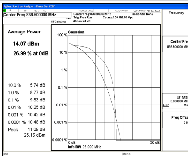
Band5-3MHz-QPSK-20525-6-0-Low-9.83-&lt;=13-PASS
