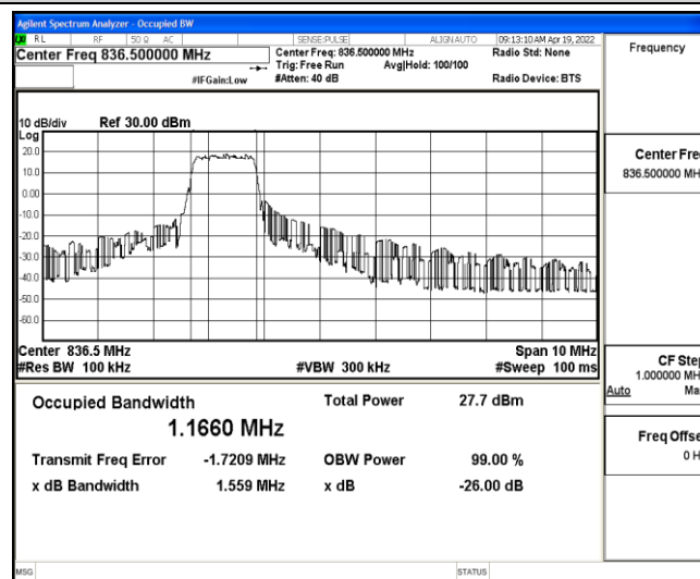
Band5-5MHz-16QAM-20525-6-0-Low-1.1660-1.559-PASS
