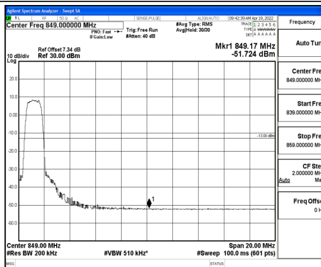
Band5-10MHz-16QAM-20600-6-0-Low--51.72-PASS
