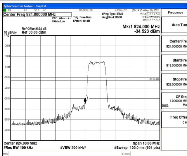
Band5-5MHz-16QAM-20425-6-0-Low--34.52-PASS
