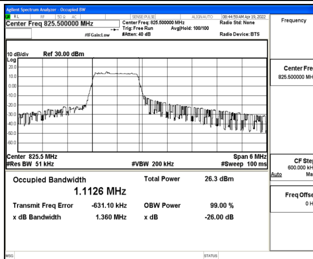
Band5-3MHz-16QAM-20415-6-0-Low-1.1126-1.360-PASS
