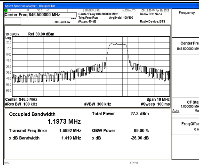
Band5-5MHz-QPSK-20625-6-0-High-1.1973-1.419-PASS
