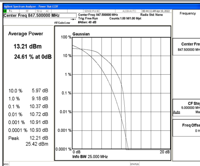
Band5-3MHz-QPSK-20635-6-0-Low-10.37-&lt;=13-PASS
