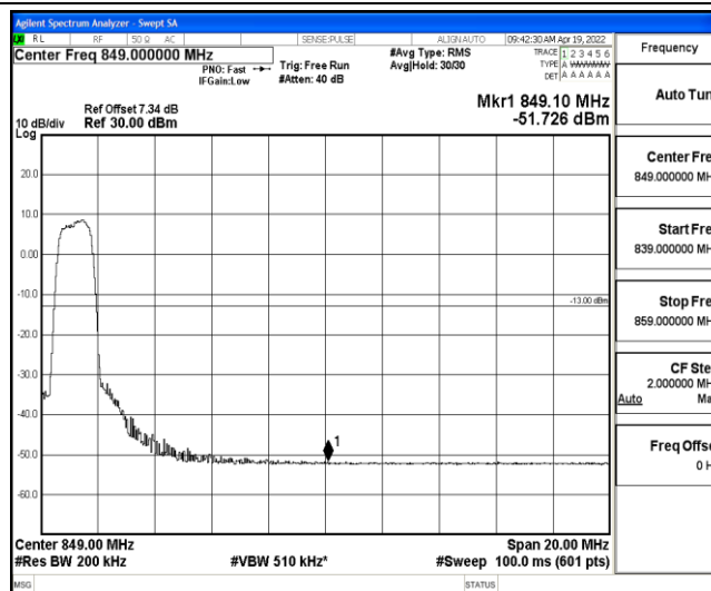
Band5-10MHz-QPSK-20600-6-0-Low--51.73-PASS
