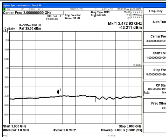
Band5-1.4MHz-QPSK-20407-1-0-Low-1000-5000--43.21-PASS
