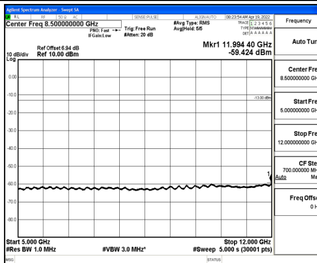
Band5-1.4MHz-16QAM-20407-1-0-Low-5000-12000--59.42-PASS
