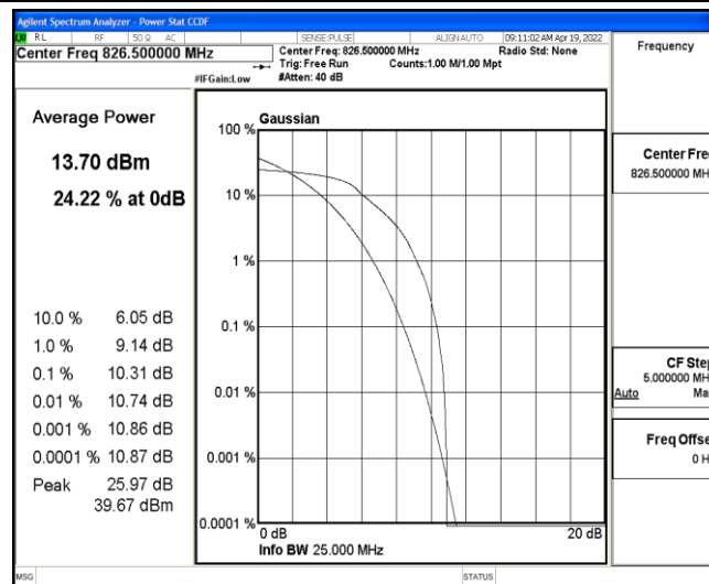
Band5-5MHz-QPSK-20425-6-0-Low-10.31-13-PASS
