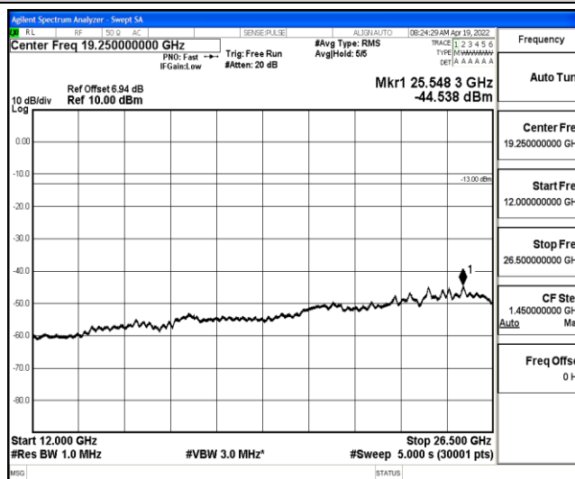
Band5-1.4MHz-16QAM-20407-1-0-Low-12000-26500--44.54-PASS
