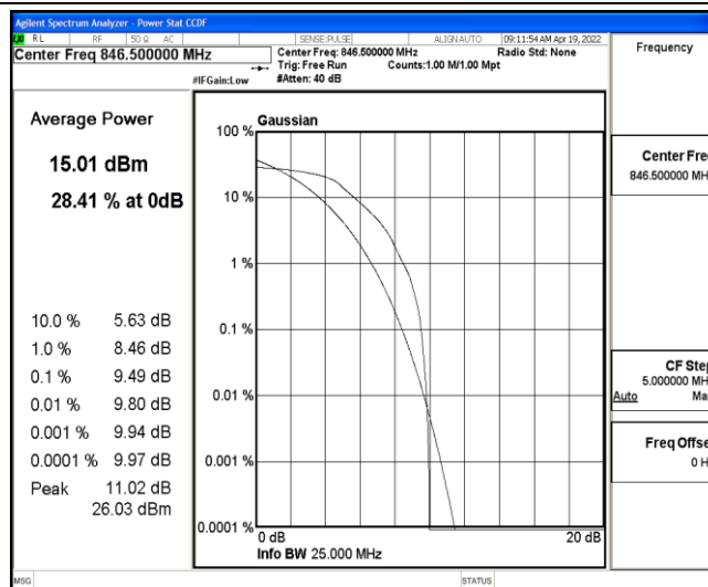
Band5-5MHz-16QAM-20625-6-0-Low-9.49-&lt;=13-PASS
