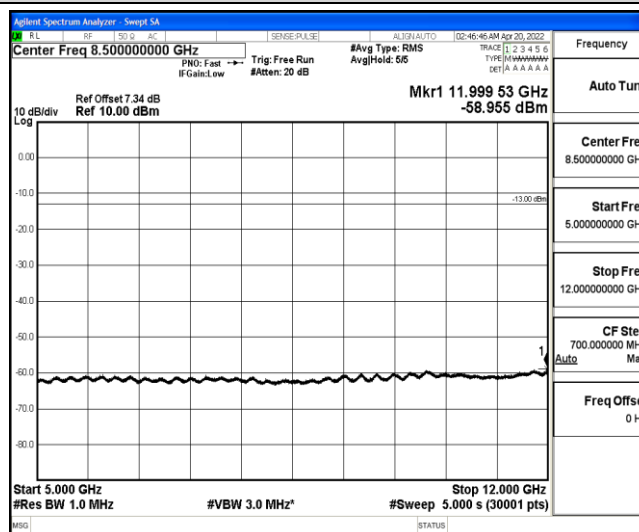
Band5-1.4MHz-QPSK-20525-1-0-Low-5000-12000--58.96-PASS
