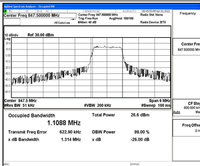
Band5-3MHz-QPSK-20635-6-0-High-1.1088-1.314-PASS
