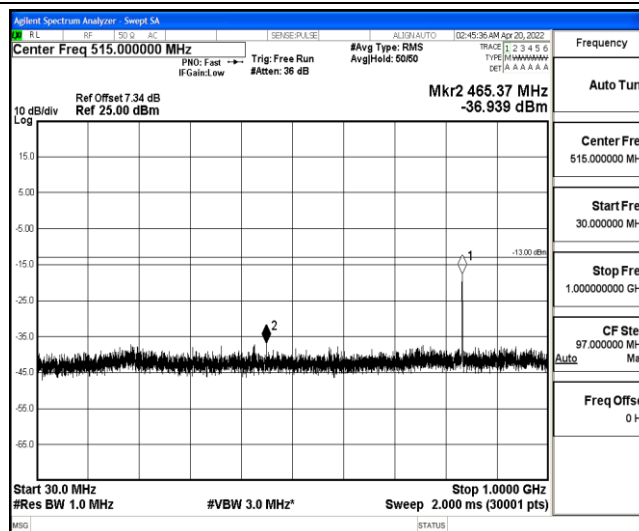
Band5-1.4MHz-QPSK-20525-1-0-Low-30-1000--36.94-PASS
