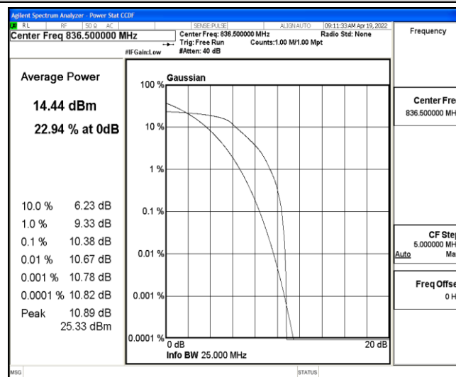
Band5-5MHz-16QAM-20525-6-0-Low-10.38-&lt;=13-PASS
