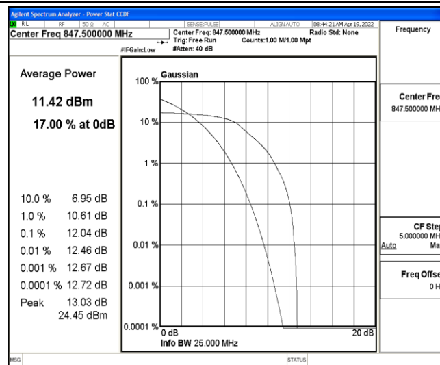
Band5-3MHz-16QAM-20635-6-0-Low-12.04-13-PASS
