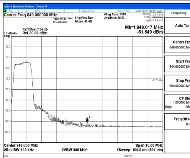
Band5-5MHz-QPSK-20625-6-0-Low--51.55-PASS
