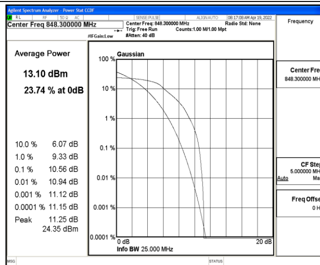
Band5-1.4MHz-QPSK-20643-6-0-Low-10.56-&lt;=13-PASS
