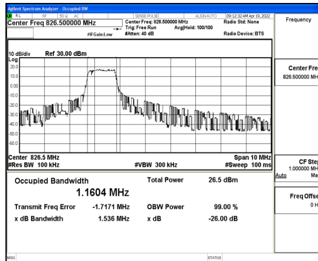
Band5-5MHz-16QAM-20425-6-0-Low-1.1604-1.536-PASS
