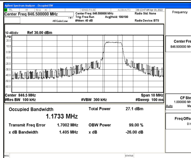
Band5-5MHz-16QAM-20625-6-0-High-1.1733-1.405-PASS
