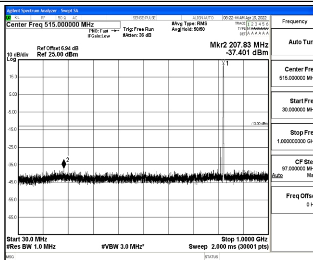
Band5-1.4MHz-16QAM-20407-1-0-Low-30-1000--37.4-PASS
