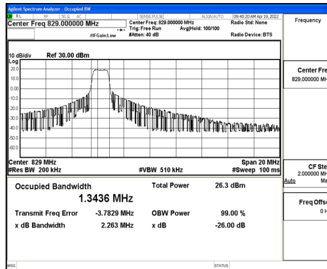
Band5-10MHz-QPSK-20450-6-0-Low-1.3436-2.263-PASS
