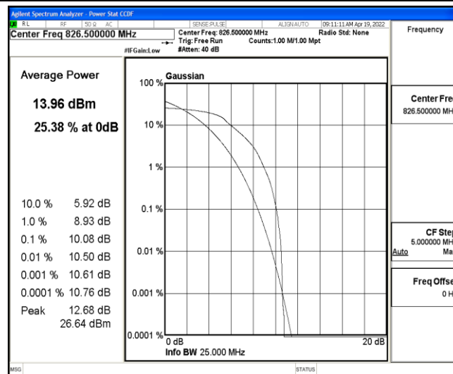
Band5-5MHz-16QAM-20425-6-0-Low-10.08-&lt;=13-PASS
