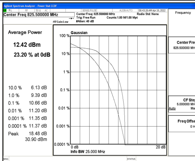
Band5-3MHz-QPSK-20415-6-0-Low-10.66-&lt;=13-PASS
