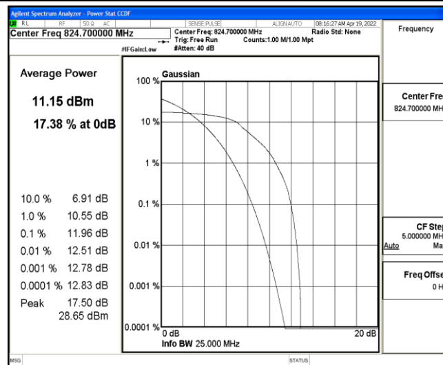
Band5-1.4MHz-16QAM-20407-6-0-Low-11.96-&lt;=13-PASS
