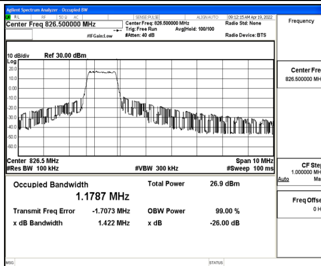
Band5-5MHz-QPSK-20425-6-0-Low-1.1787-1.422-PASS
