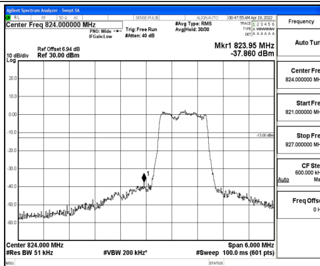
Band5-3MHz-QPSK-20415-6-0-Low--37.86-PASS
