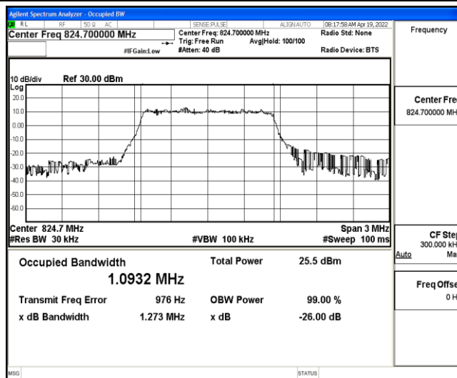
Band5-1.4MHz-16QAM-20407-6-0-Low-1.0932-1.273-PASS
