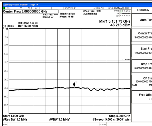
Band5-1.4MHz-QPSK-20525-1-0-Low-1000-5000--43.22-PASS
