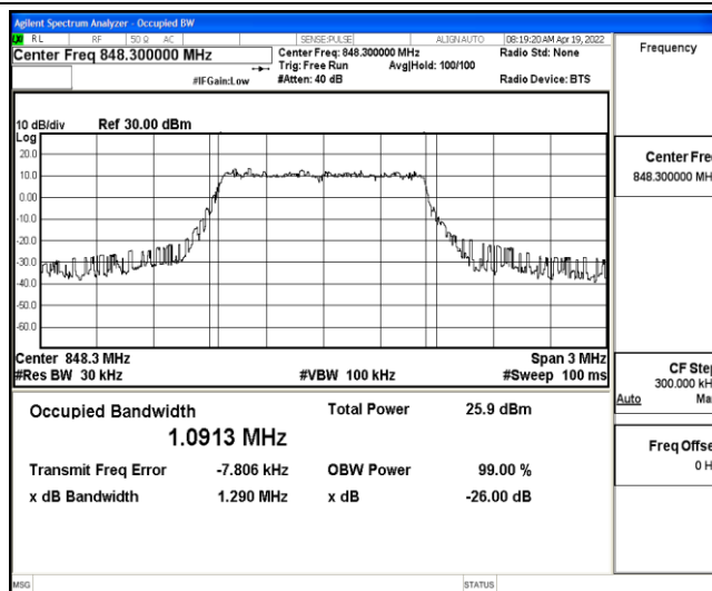
Band5-1.4MHz-16QAM-20643-6-0-High-1.0913-1.290-PASS
