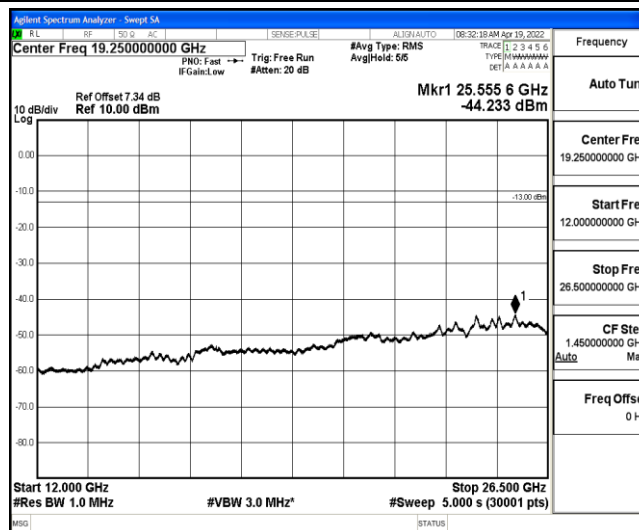
Band5-1.4MHz-16QAM-20643-1-0-High-12000-26500--44.23-PASS
