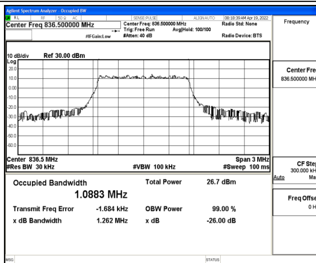
Band5-1.4MHz-16QAM-20525-6-0-Low-1.0883-1.262-PASS
