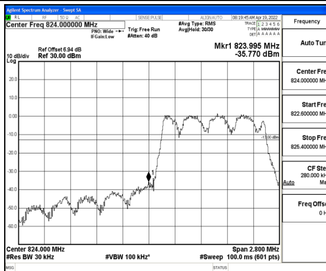
Band5-1.4MHz-16QAM-20407-6-0-Low--35.77-PASS
