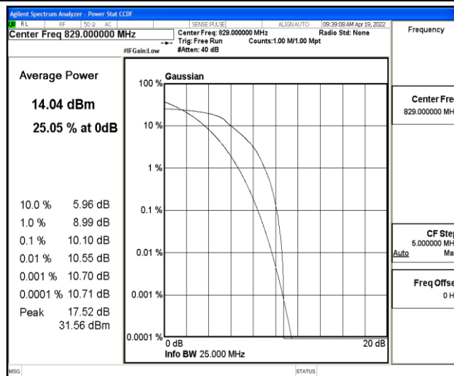
Band5-10MHz-QPSK-20450-6-0-Low-10.10-&lt;=13-PASS
