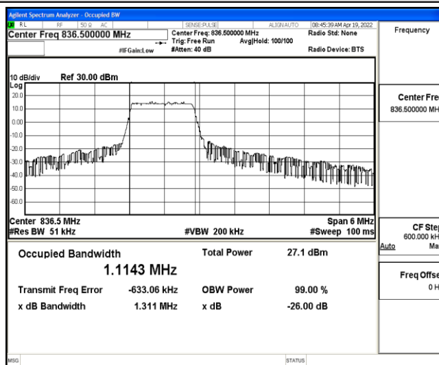
Band5-3MHz-16QAM-20525-6-0-Low-1.1143-1.311-PASS
