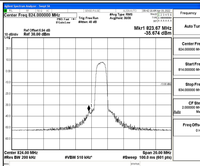
Band5-10MHz-16QAM-20450-6-0-Low--35.67-PASS
