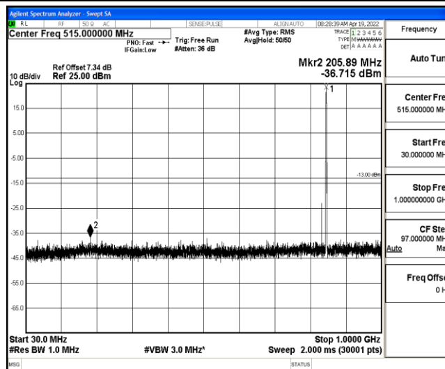
Band5-1.4MHz-QPSK-20643-1-0-High-30-1000--36.72-PASS
