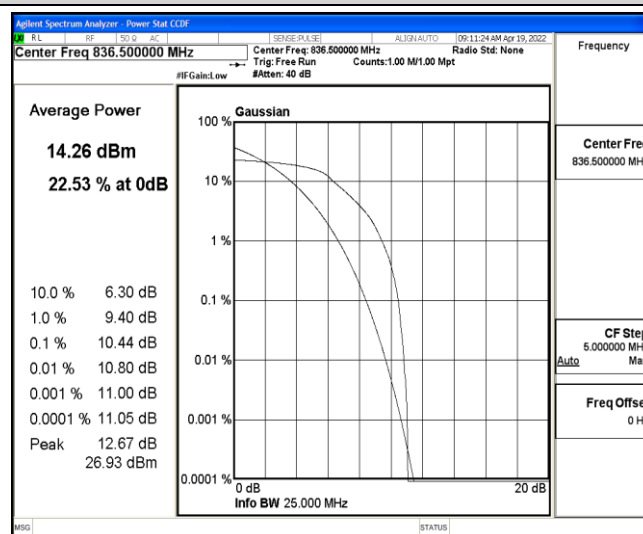
Band5-5MHz-QPSK-20525-6-0-Low-10.44-13-PASS
