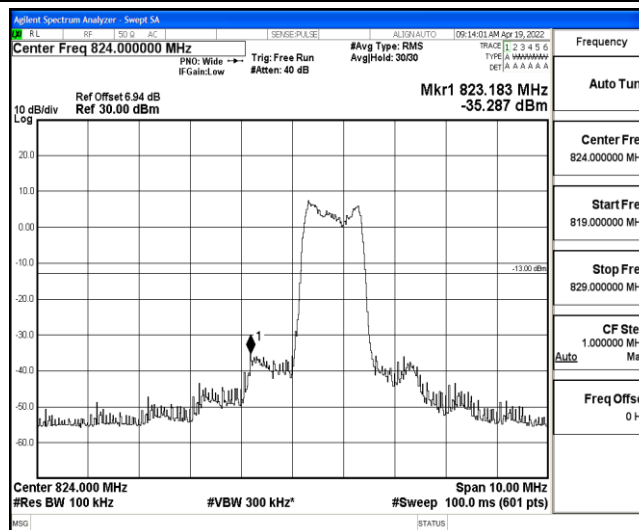
Band5-5MHz-QPSK-20425-6-0-Low--35.29-PASS
