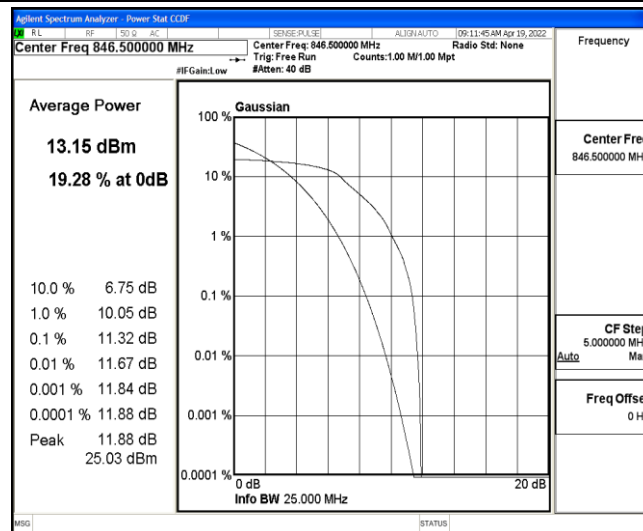
Band5-5MHz-QPSK-20625-6-0-Low-11.32-&lt;=13-PASS
