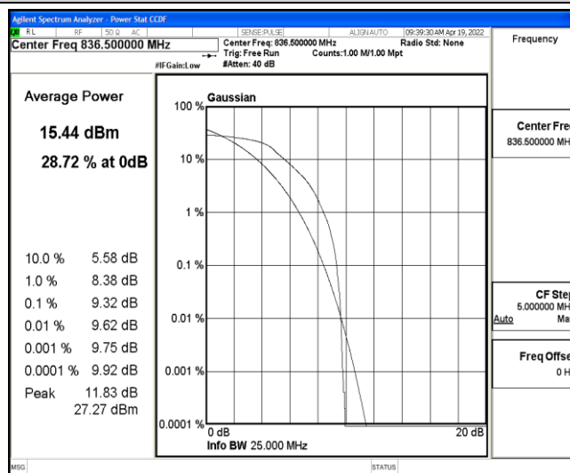
Band5-10MHz-QPSK-20525-6-0-Low-9.32-&lt;=13-PASS
