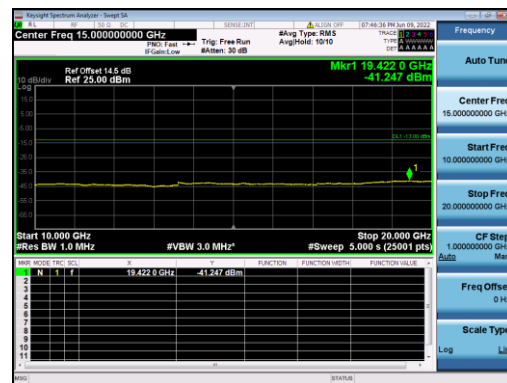
B25-3M-High CH-CSE-1-QPSK-1 RB 0
