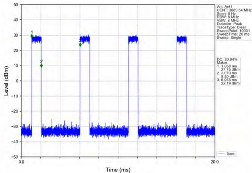
n78d_30kHz_MIMO_NTNV_20MHz_CP-OFDM_16_QAM_3690MHz_Inner_Full
