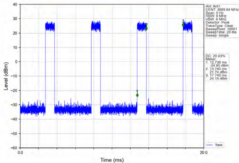
n78d_30kHz_MIMO_NTNV_20MHz_CP-OFDM_256_QAM_3690MHz_Inner_Full
