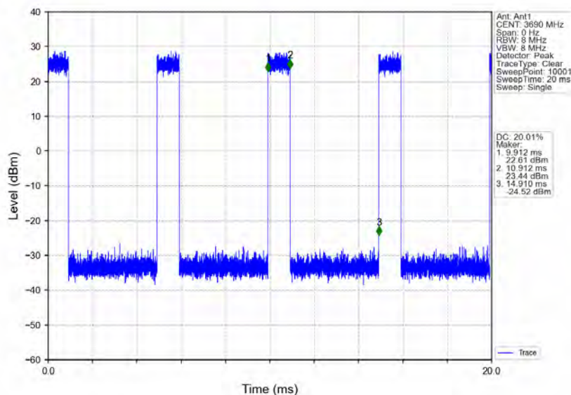
n78d_30kHz_MIMO_NTNV_20MHz_CP-OFDM_64_QAM_3690MHz_Inner_Full
