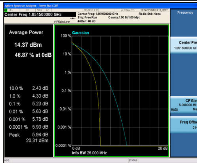
Band2_3MHz_16QAM_18615_15RB#0_6.12_13_PASS
