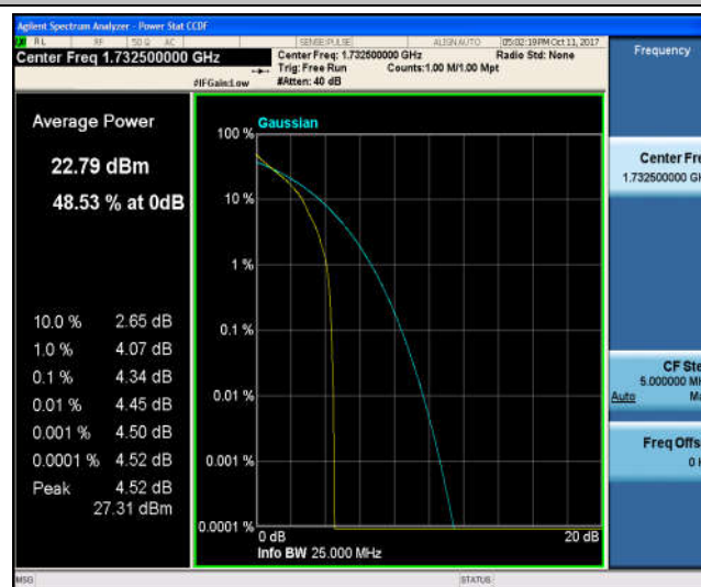
Band4_3MHz_16QAM_20175_1RB#0_5.31_13_PASS
