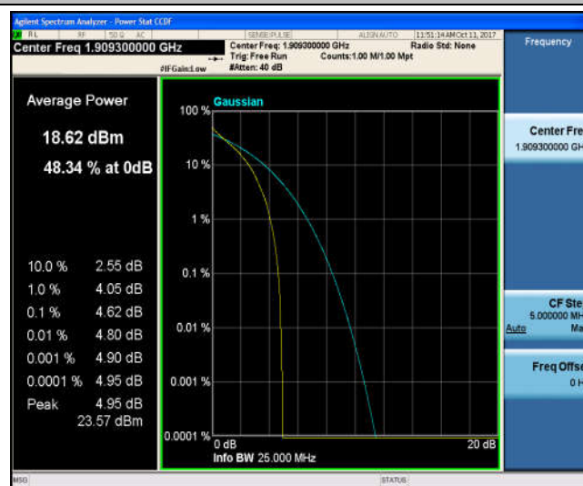
Band2_1.4MHz_16QAM_19193_6RB#0_5.47_13_PASS
