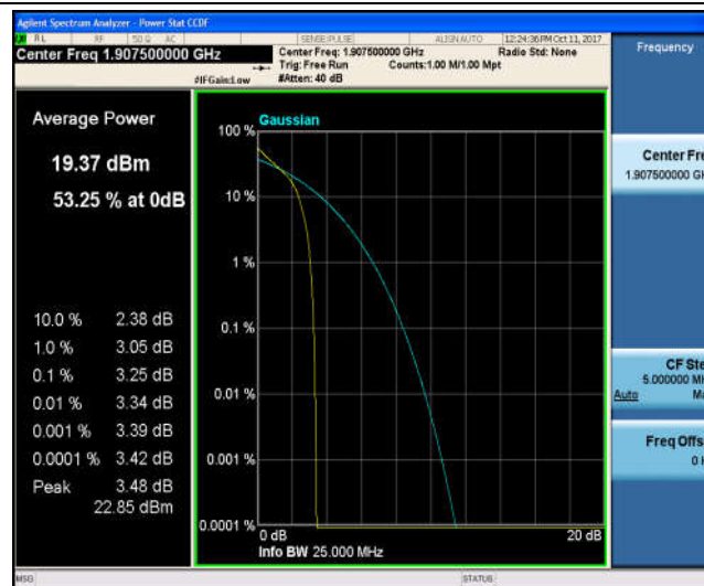
Band2_5MHz_16QAM_19175_1RB#0_4.17_13_PASS
