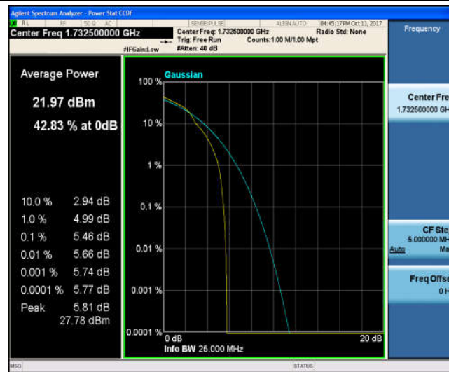
Band4_1.4MHz_QPSK_20175_6RB#0_5.42_13_PASS
