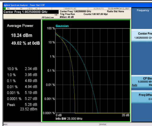
Band2_15MHz_16QAM_19125_75RB#0_5.42_13_PASS
