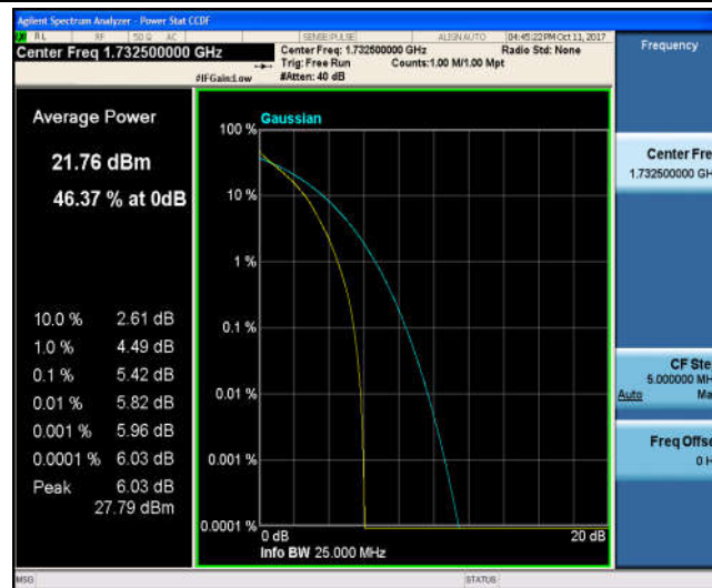
Band4_1.4MHz_16QAM_20175_6RB#0_6.27_13_PASS
