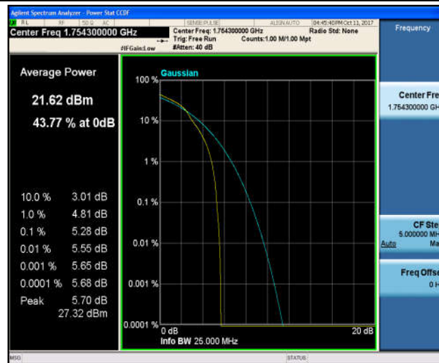
Band4_1.4MHz_QPSK_20393_6RB#0_5.25_13_PASS
