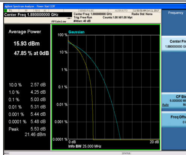
Band2_1.4MHz_16QAM_18900_6RB#0_5.94_13_PASS
