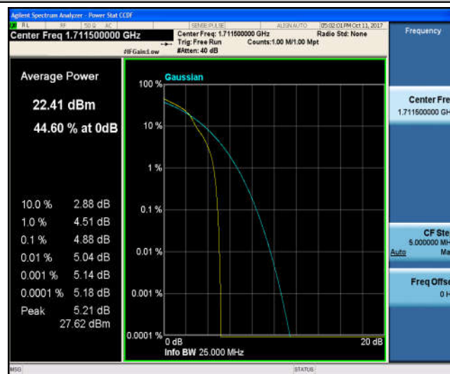
Band4_3MHz_QPSK_19965_15RB#0_5.06_13_PASS
