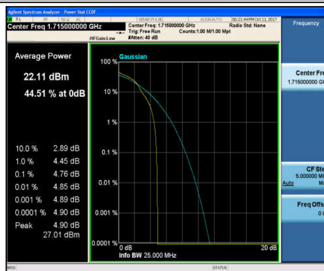
Band4_10MHz_QPSK_20000_50RB#0_5.23_13_PASS
