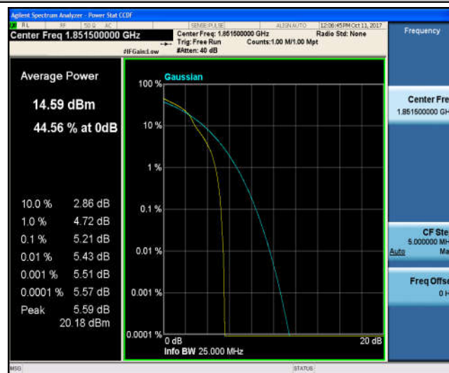
Band2_3MHz_QPSK_18615_15RB#0_5.23_13_PASS
