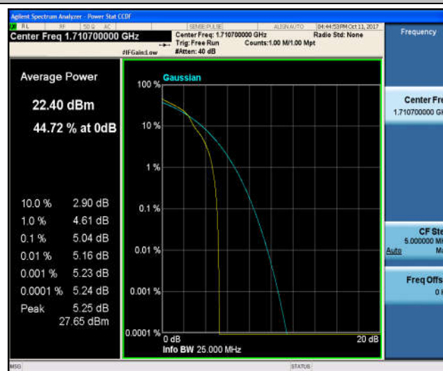
Band4_1.4MHz_QPSK_19957_6RB#0_4.95_13_PASS
