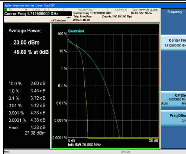
Band4_5MHz_16QAM_19975_1RB#0_4.62_13_PASS
