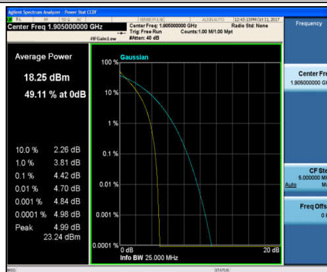
Band2_10MHz_16QAM_19150_50RB#0_5.27_13_PASS
