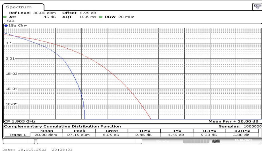
Band2-10MHz-QPSK-19150-50RB#0-PASS
