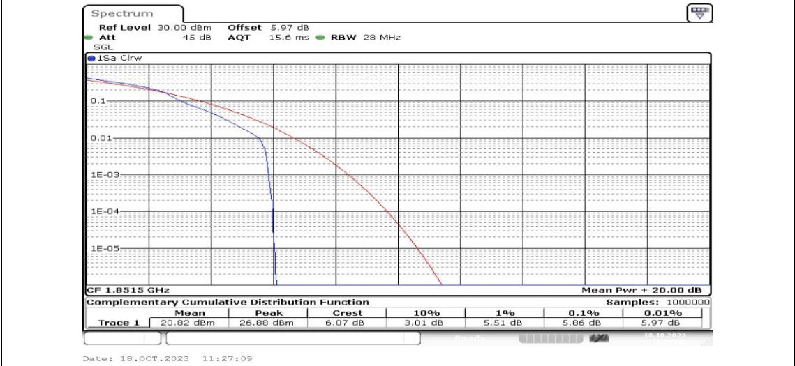
Band2-3MHz-16QAM-18615-1RB#0-PASS
