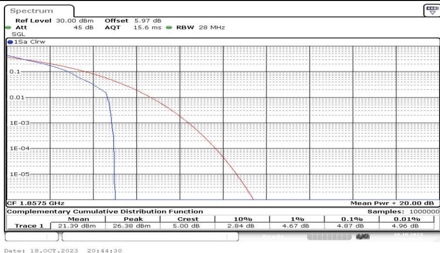
Band2-15MHz-QPSK-18675-1RB#0-PASS
