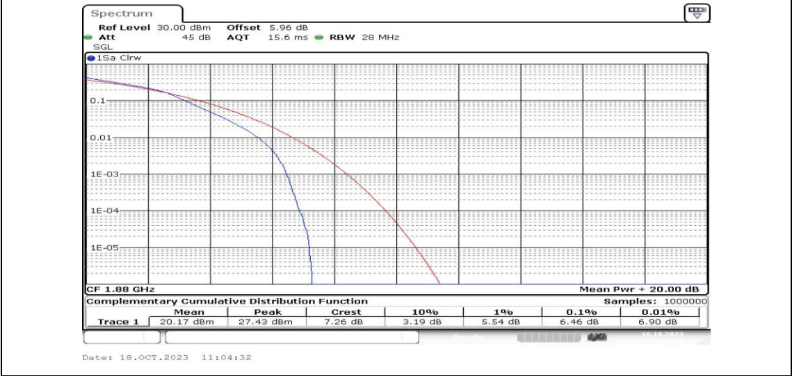
Band2-1.4MHz-16QAM-18900-6RB#0-PASS
