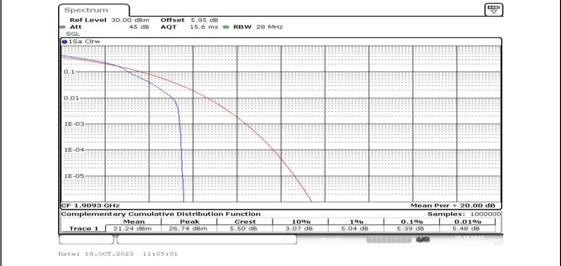
Band2-1.4MHz-16QAM-19193-1RB#0-PASS
