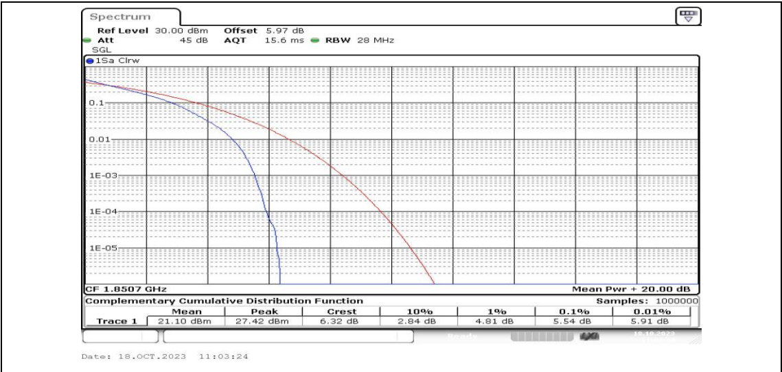
Band2-1.4MHz-QPSK-18607-6RB#0-PASS
