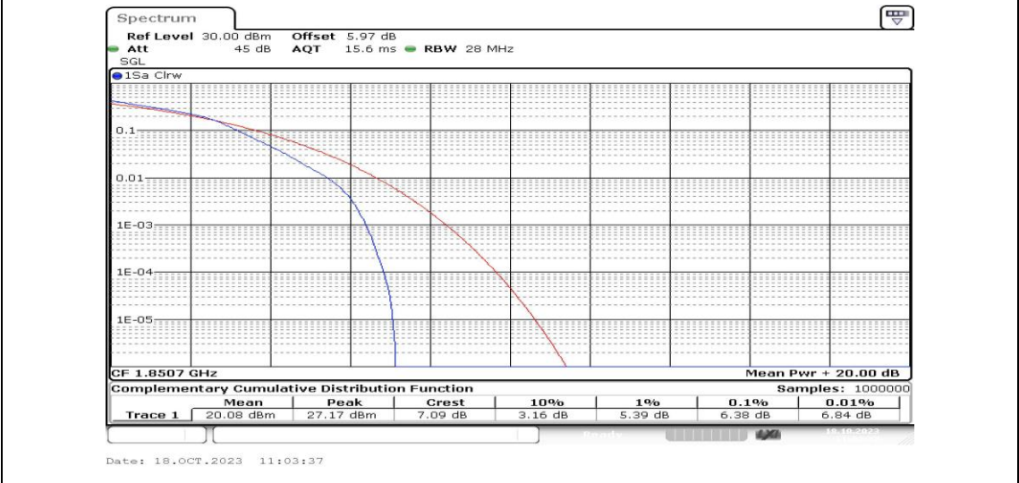
Band2-1.4MHz-16QAM-18607-6RB#0-PASS
