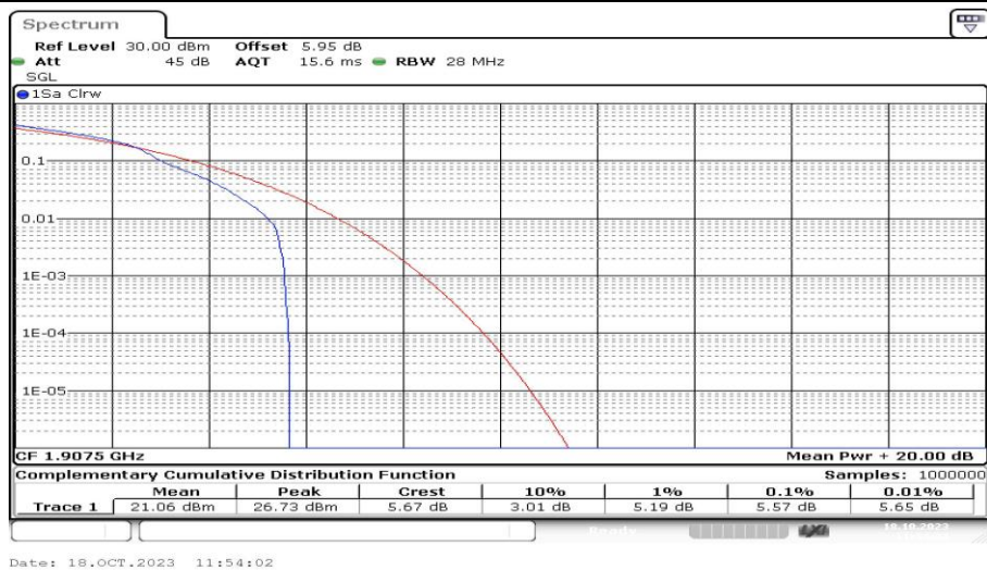
Band2-5MHz-16QAM-19175-1RB#0-PASS
