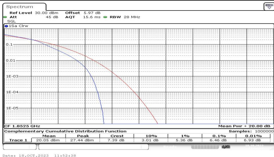
Band2-5MHz-16QAM-18625-25RB#0-PASS
