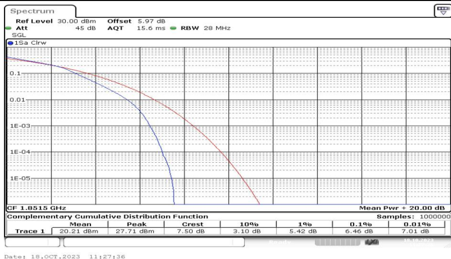
Band2-3MHz-16QAM-18615-15RB#0-PASS
