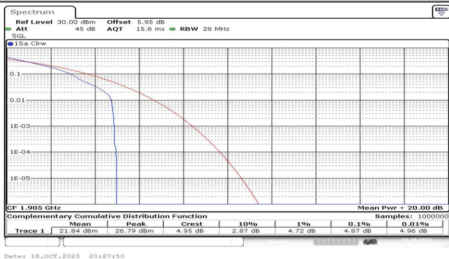
Band2-10MHz-QPSK-19150-1RB#0-PASS
