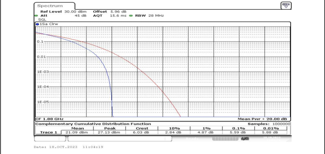
Band2-1.4MHz-QPSK-18900-6RB#0-PASS
