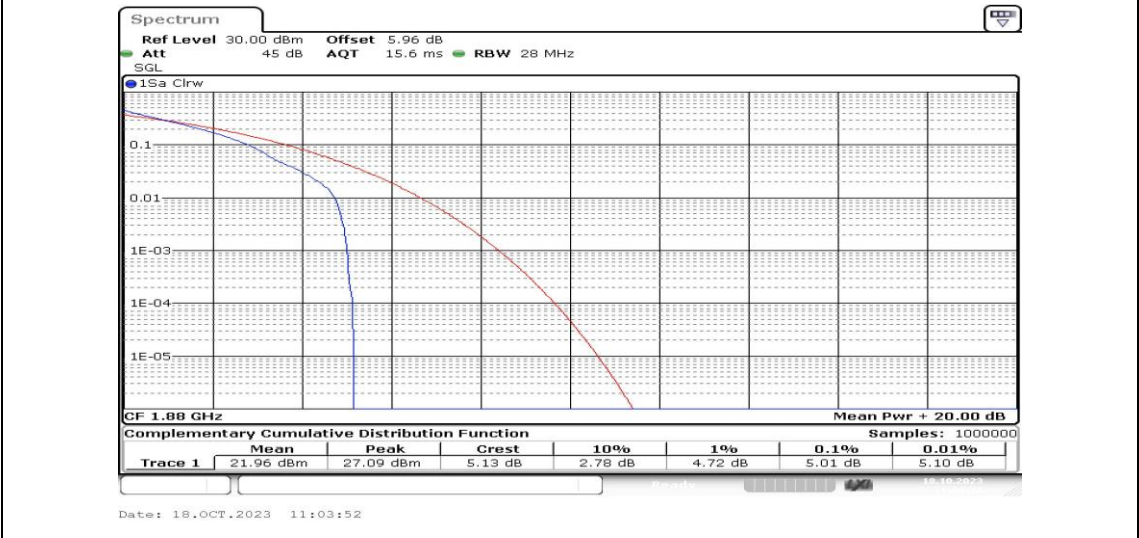
Band2-1.4MHz-QPSK-18900-1RB#0-PASS
