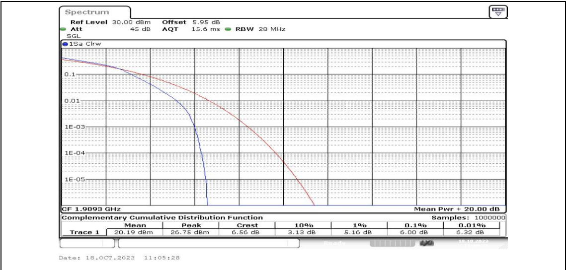
Band2-1.4MHz-16QAM-19193-6RB#0-PASS
