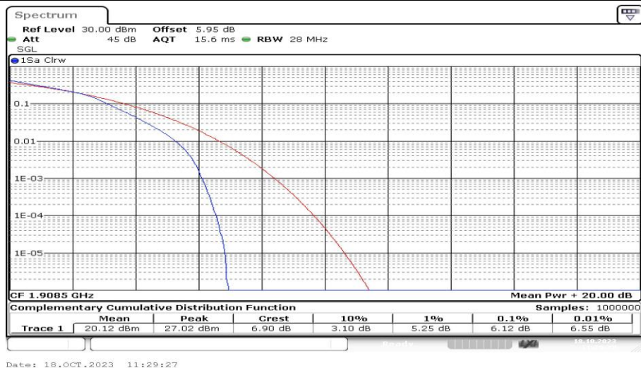
Band2-3MHz-16QAM-19185-15RB#0-PASS
