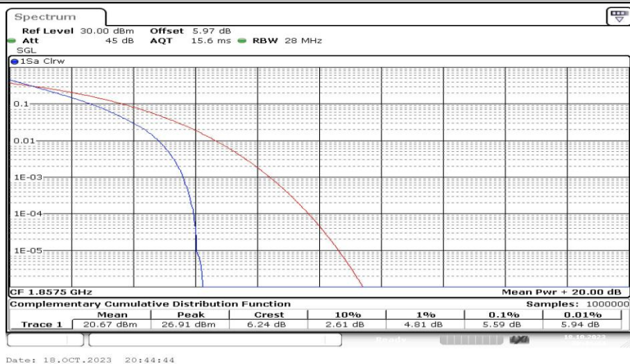
Band2-15MHz-QPSK-18675-75RB#0-PASS
