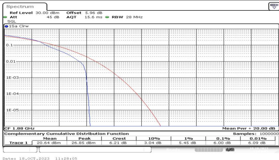
Band2-3MHz-16QAM-18900-1RB#0-PASS
