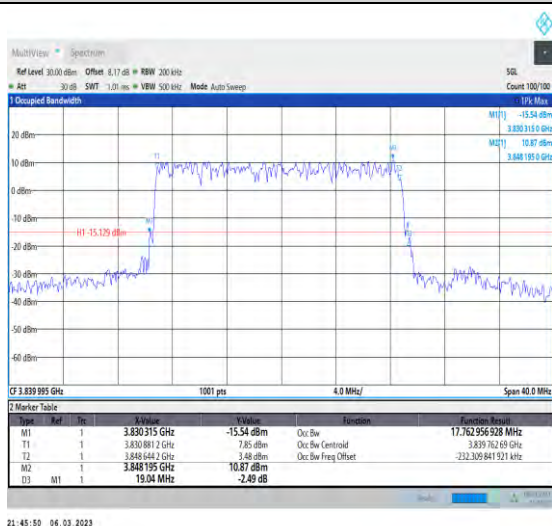
1-N77-3700-3980-PC3-30-20-M-4-DFT-64QAM-Out er_Full-50@0-Ant1-17.763-19.040-≤20-PASS
