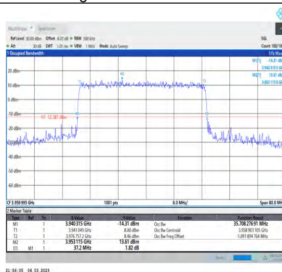
1-N77-3700-3980-PC3-30-40-H-3-DFT-16QAM-Oute r_Full-100@0-Ant1-35.708-37.200-≤40-PASS
