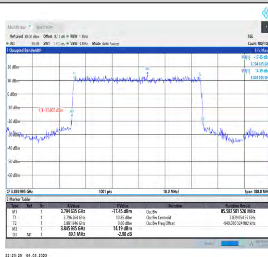
1-N77-3700-3980-PC3-30-90-M-2-DFT-PI2BPSK-Out_r_Full-240@0-Ant1-85.583-89.100-≤90-PASS
