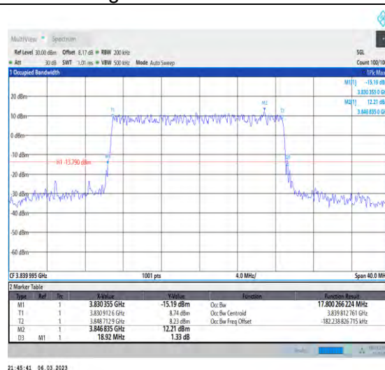
1-N77-3700-3980-PC3-30-20-M-3-DFT-16QAM-Out er_Full-50@0-Ant1-17.8-18.920-≤20-PASS
