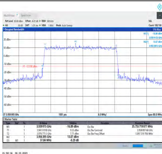
1-N77-3700-3980-PC3-30-40-H-4-DFT-64QAM-Oute r_Full-100@0-Ant1-35.756-37.840-≤40-PASS
