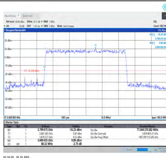
1-N77-3700-3980-PC3-30-80-M-5-DFT-256QAM-Out_Full-216@0-Ant1-77.044-80.320-≤80-PASS
