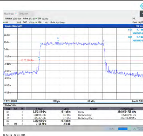
1-N77-3700-3980-PC3-30-40-H-5-DFT-256QAM-Oute r_Full-100@0-Ant1-35.639-37.360-≤40-PASS
