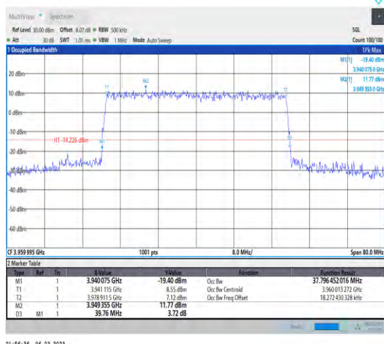
1-N77-3700-3980-PC3-30-40-H-6-CP-QPSK-Outer_Full-106@0-Ant1-37.796-39.760-≤40-PASS
