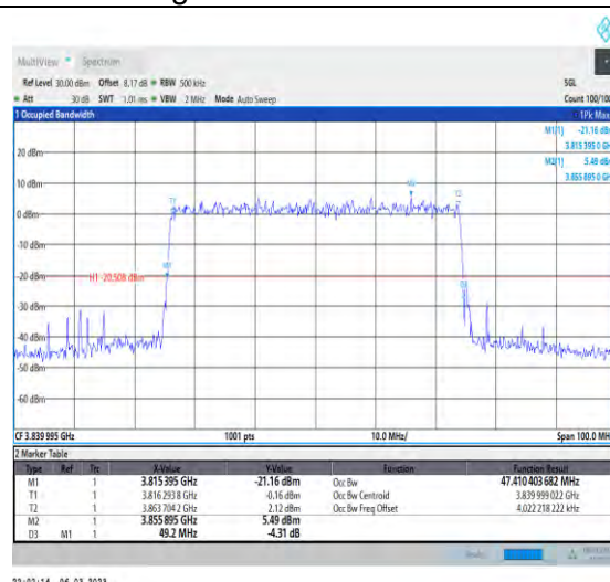
1-N77-3700-3980-PC3-30-50-M-9-CP-256QAM-Outer_Full-133@0-Ant1-47.41-49.200-≤50-PASS
