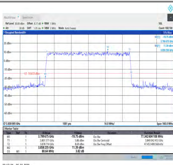
1-N77-3700-3980-PC3-30-80-M-8-CP-64QAM-Outer_Full-217@0-Ant1-77.343-80.640-≤80-PASS
