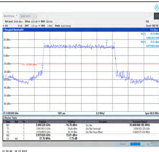
1-N77-3700-3980-PC3-30-40-H-2-DFT-PI2BPSK-Out er_Full-100@0-Ant1-35.848-37.760-≤40-PASS
