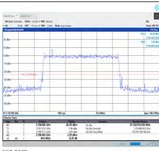
1-N77-3700-3980-PC3-30-50-L-9-CP-256QAM-Outer_Full-133@0-Ant1-47.343-49.600-≤50-PASS
