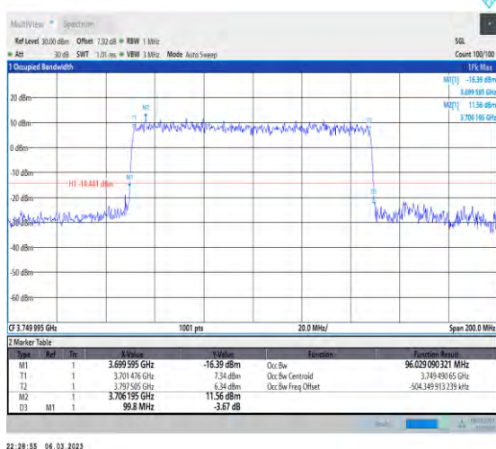
1-N77-3700-3980-PC3-30-100-L-3-DFT-16QAM-Outer_Full-270@0-Ant1-96.029-99.800-≤100-PASS
