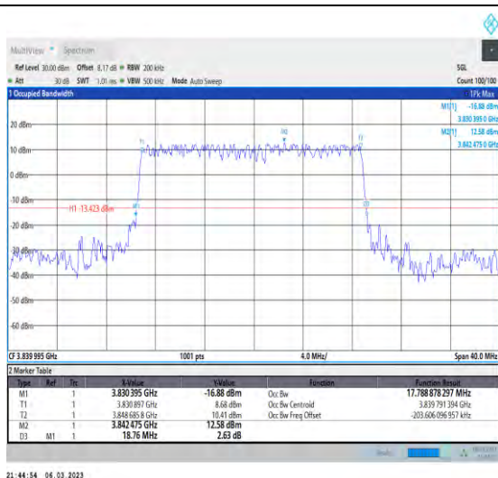
1-N77-3700-3980-PC3-30-20-M-2-DFT-PI2BPSK-Outer_Full-50@0-Ant1-17.789-18.760-≤20-PASS
