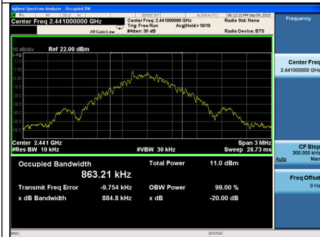
99% and 20dB BW –Bluetooth BDR 2441MHz
