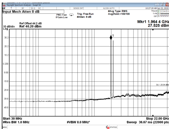
Figure 8.5-71: Conducted spurious emissions for dual band simultaneous transmission with 20 MHz mid channel single-carrier (per band) operation
