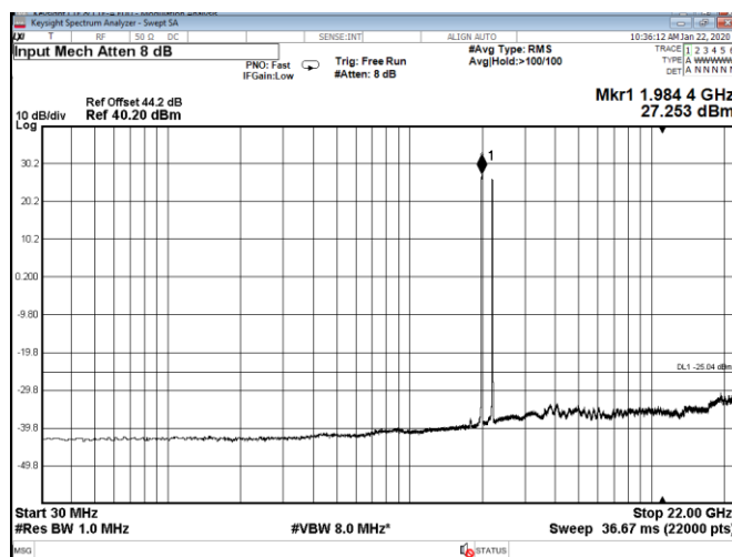
Figure 8.5-75: Conducted spurious emissions for dual band simultaneous transmission with 10 MHz top channels dual-carrier (per band) operation
