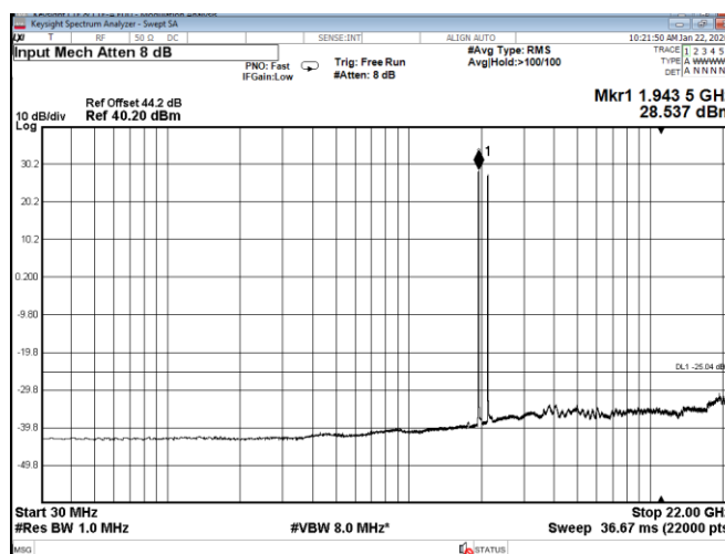
Figure 8.5-67: Conducted spurious emissions for dual band simultaneous transmission with 15 MHz low channel single-carrier (per band) operation
