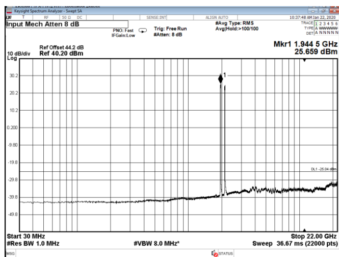
Figure 8.5-76: Conducted spurious emissions for dual band simultaneous transmission with 15 MHz bottom channels dual-carrier (per band) operation
