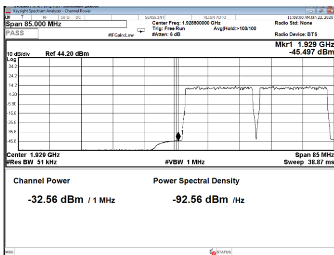
Figure 8.5-57: Conducted band edge emission at 1929 MHz, 20 MHz two-carrier operation (RBW = 1 MHz)
