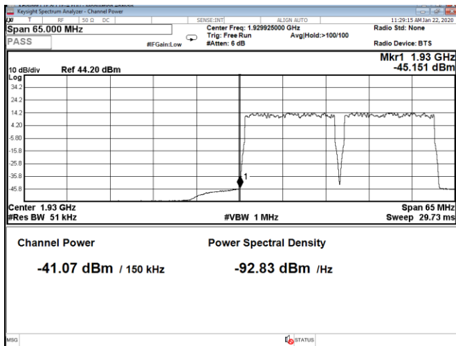
Figure 8.5-54: Conducted band edge emission at 1930 MHz, 15 MHz two-carrier operation (RBW = 1% of EBW)
