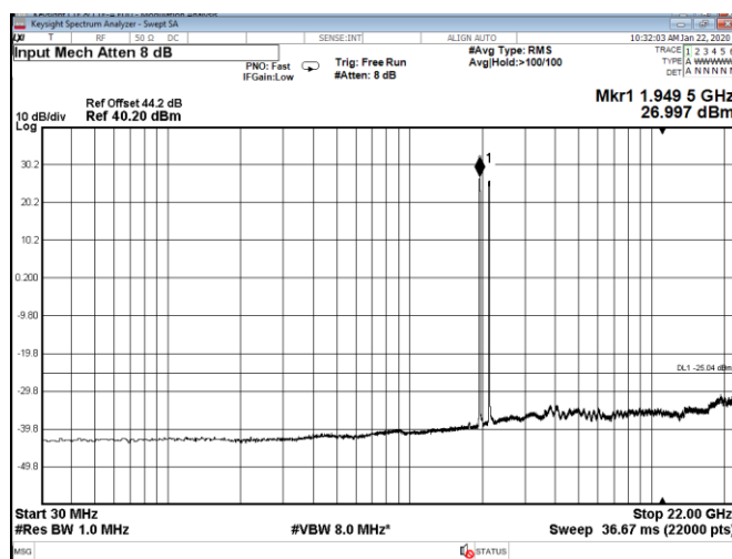
Figure 8.5-73: Conducted spurious emissions for dual band simultaneous transmission with 10 MHz bottom channels dual-carrier (per band) operation
