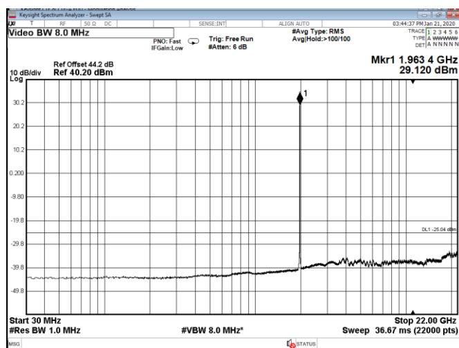
Figure 8.5-5: Conducted spurious emissions of 15 MHz mid channel, single-carrier operation
