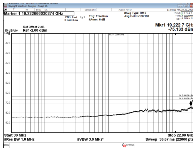
Figure 8.10-1: Receiver spurious emissions at Port 021
