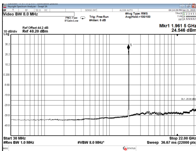
Figure 8.5-26: Conducted spurious emissions of 10 MHz middle channels, two-carrier operation with IoT
