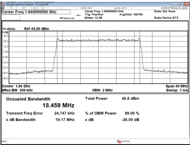
Figure 8.7-6: Occupied bandwidth for 20 MHz channel LTE + IoT, sample plot
