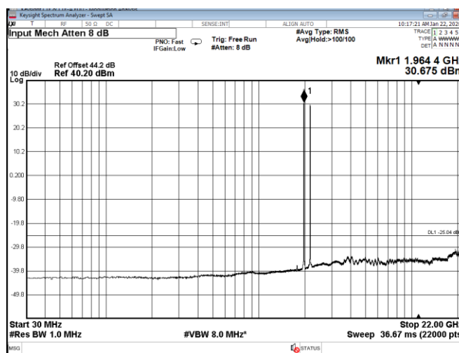
Figure 8.5-65: Conducted spurious emissions for dual band simultaneous transmission with 10 MHz mid channel single-carrier (per band) operation
