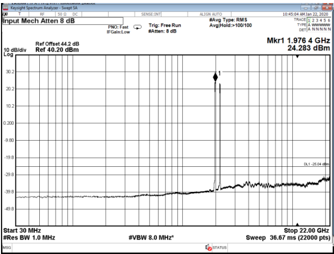
Figure 8.5-81: Conducted spurious emissions for dual band simultaneous transmission with 20 MHz top channels dual-carrier (per band) operation
