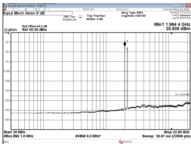
Figure 8.5-78: Conducted spurious emissions for dual band simultaneous transmission with 15 MHz top channels dual-carrier (per band) operation
