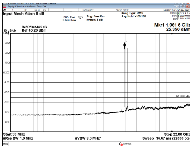
Figure 8.5-77: Conducted spurious emissions for dual band simultaneous transmission with 15 MHz middle channels dual-carrier (per band) operation
