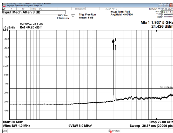
Figure 8.5-79: Conducted spurious emissions for dual band simultaneous transmission with 20 MHz bottom channels dual-carrier (per band) operation
