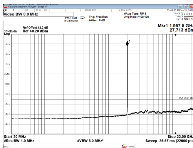
Figure 8.5-8: Conducted spurious emissions of 20 MHz mid channel, single-carrier operation
