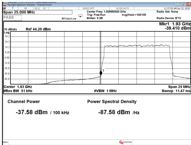
Figure 8.5-28: Conducted band edge emission at 1930 MHz, 10 MHz single carrier operation (RBW = 1% of EBW)
