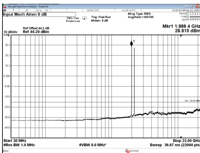
Figure 8.5-69: Conducted spurious emissions for dual band simultaneous transmission with 15 MHz high channel single-carrier (per band) operation
