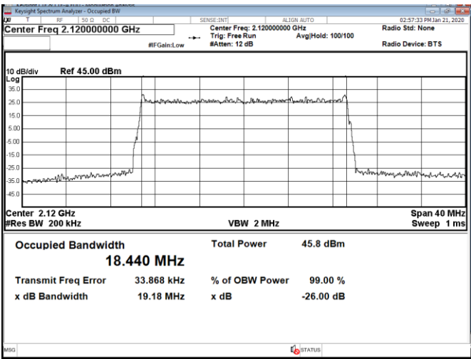
Figure 8.6-6: Occupied bandwidth for 20 MHz channel LTE + IoT, sample plot
