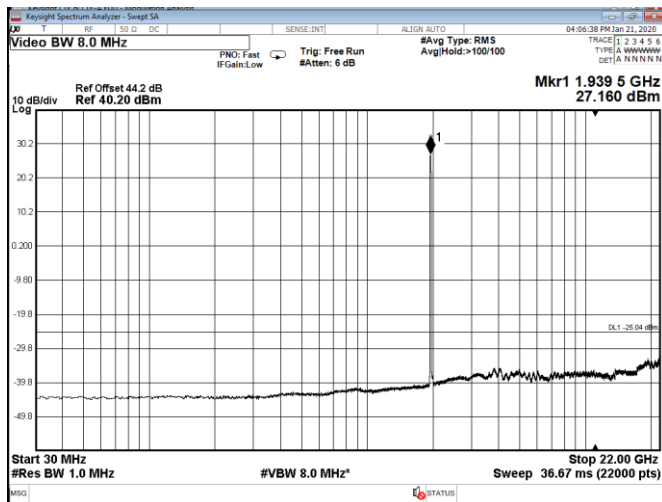
Figure 8.5-19: Conducted spurious emissions of 10 MHz bottom channels, two-carrier operation with IoT
