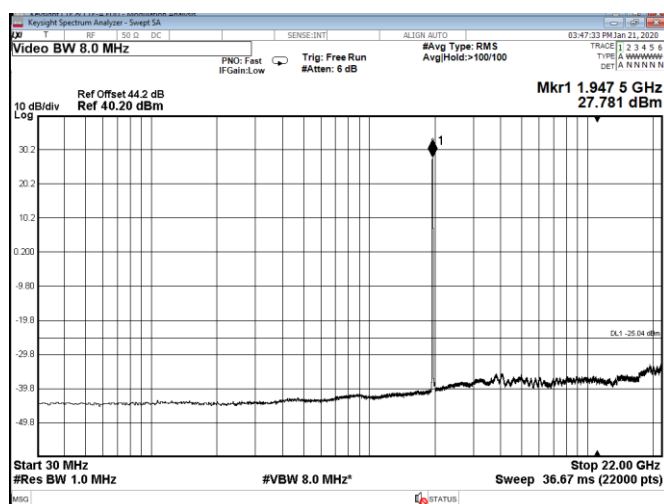
Figure 8.5-7: Conducted spurious emissions of 20 MHz low channel, single-carrier operation
