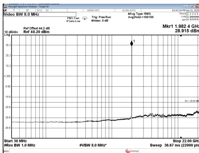
Figure 8.5-6: Conducted spurious emissions of 15 MHz high channel, single-carrier operation
