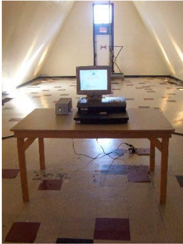
Radiated Emissions Test Setup Front
