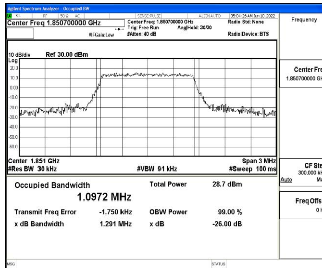
Band25-1.4MHz-16QAM-26365-6RB#0
