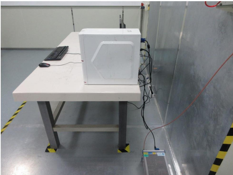
Description: Back View of Conducted Emission Test Setup – Wi-Fi
