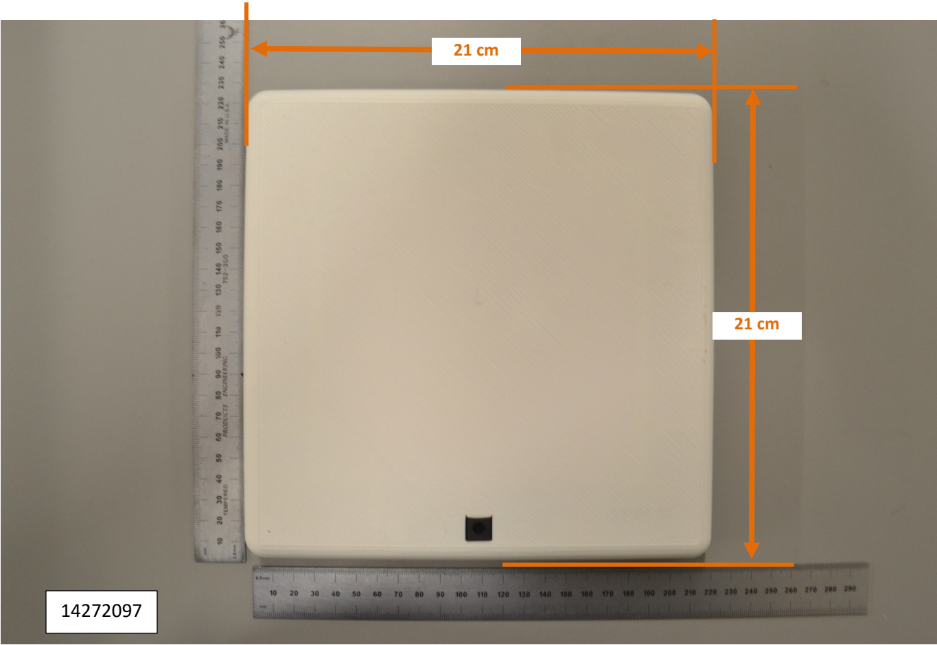
Photograph 1: Overall Dimensions
