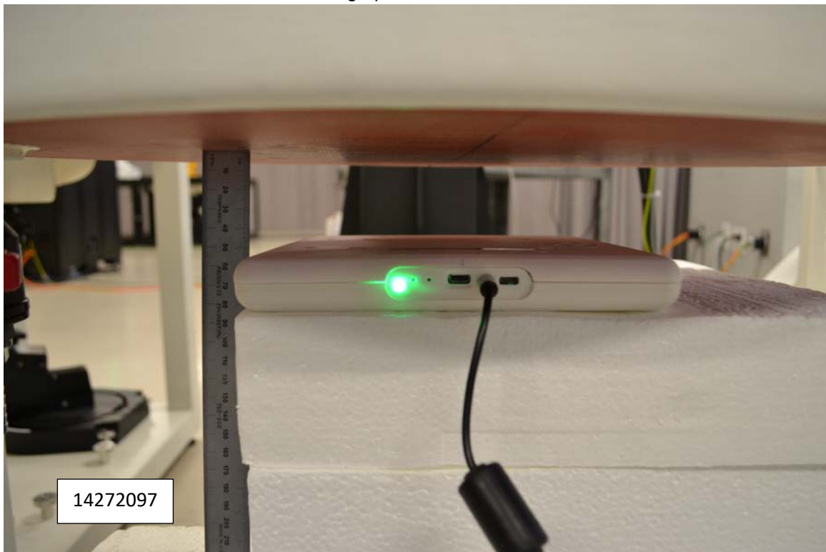
Photograph 8: Edge 1 @ 10 cm
