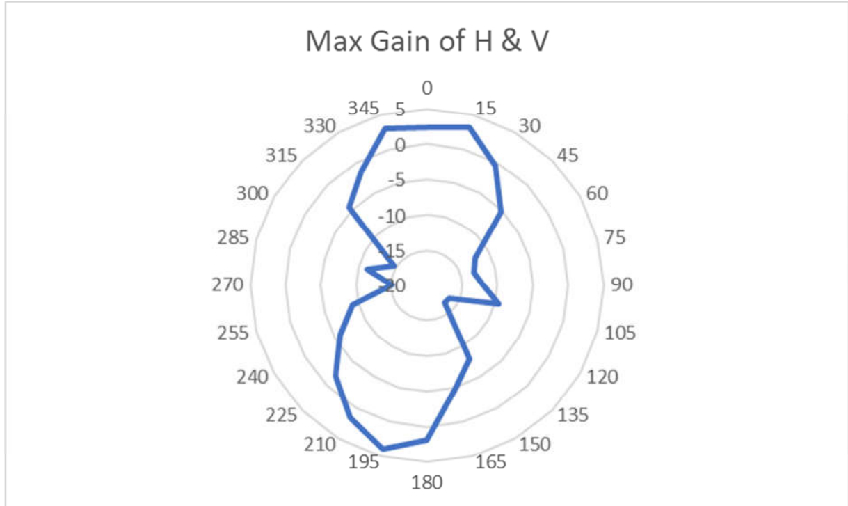
Wifi UNII-5
