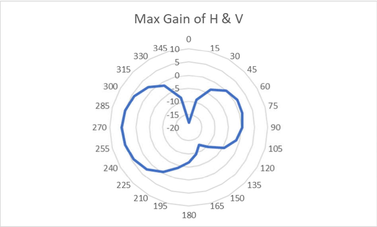
Wifi UNII-3
