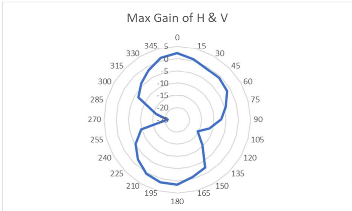
Wifi UNII-1
