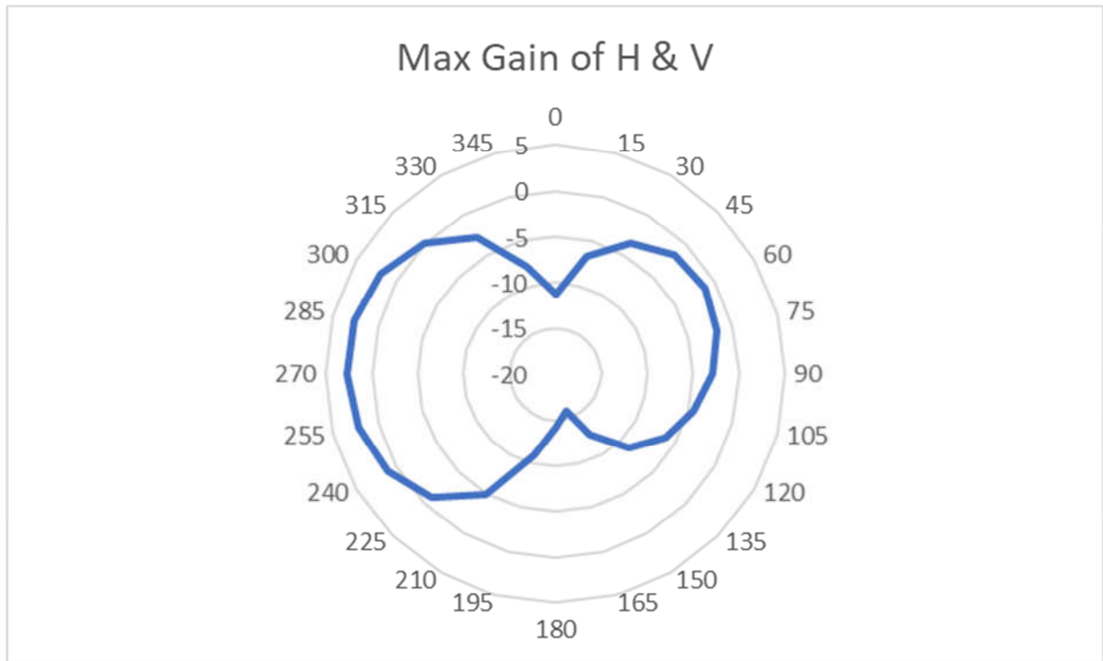
Wifi UNII-1
