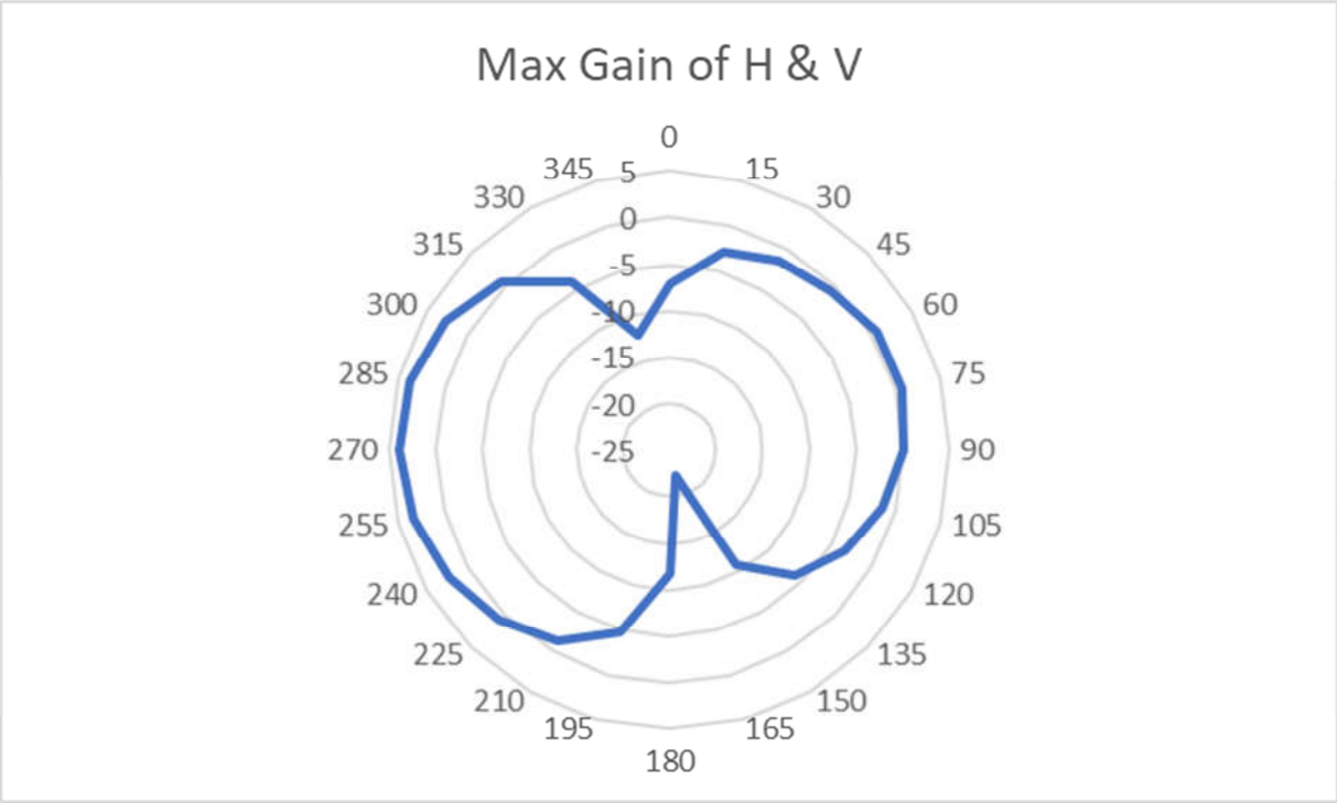
Wifi UNII-6
