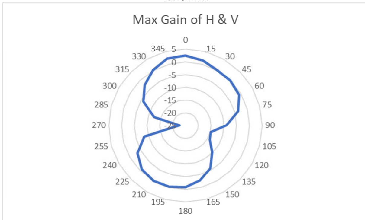
Wifi UNII-2A
