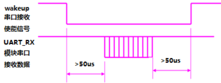
Figure 10. Module UART Receive Enable Signal Map
