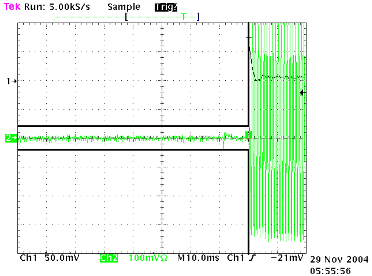
Switch Off Condition – 25 kHz Channel Spacing
