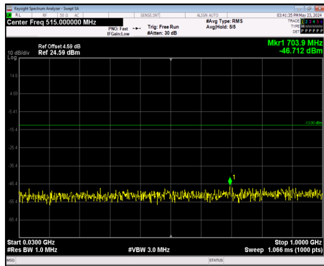
Band2-20MHz-64QAM-18900-1RB#0-Range1:30~100 0MHz
