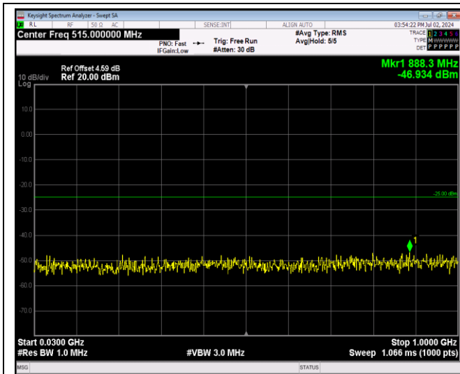
Band7-5MHz-64QAM-21100-1RB#0-Range1:30~1000 MHz
