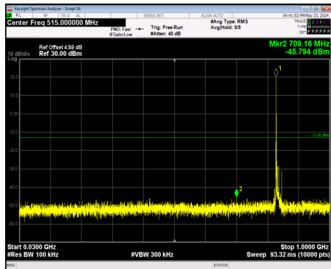
Band5-10MHz-16QAM-20600-1RB#0-Range1:30~100 0MHz
