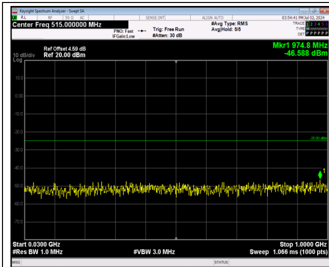
Band7-5MHz-QPSK-21425-1RB#0-Range1:30~1000 MHz
