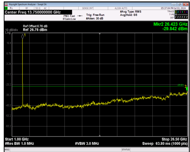
Band7-20MHz-64QAM-20850-1RB#0-Range2:1000~265
