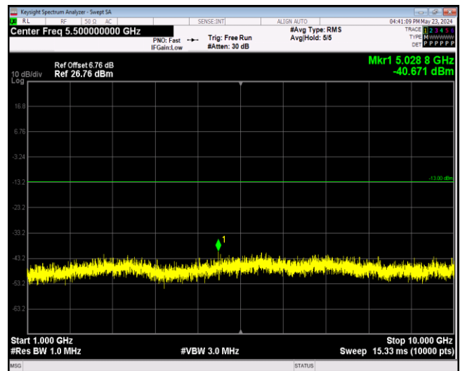
Band5-10MHz-16QAM-20600-1RB#0-Range2:1000~100 00MHz
