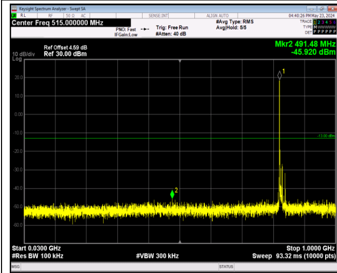
Band5-10MHz-64QAM-20525-1RB#0-Range1:30~100 0MHz
