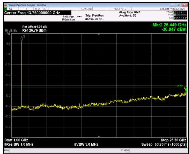
Band7-5MHz-64QAM-21425-1RB#0-Range2:1000~2650 OMHz
