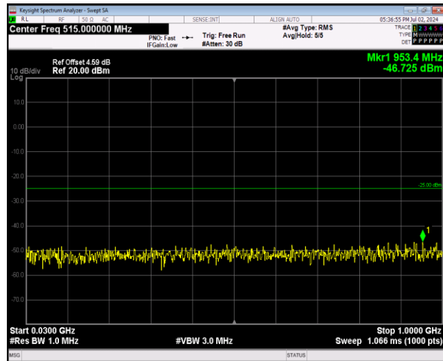
Band7-20MHz-64QAM-20850-1RB#0-Range1:30~100
