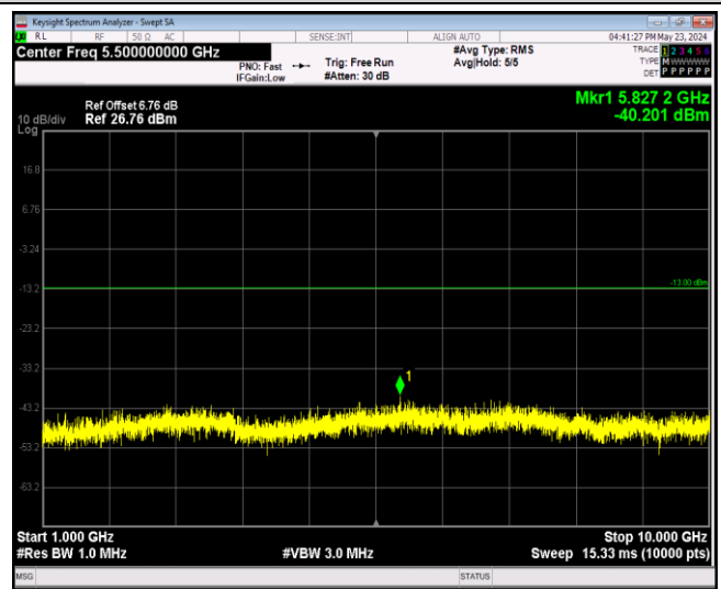
Band5-10MHz-64QAM-20525-1RB#0-Range2:1000~100 00MHz
