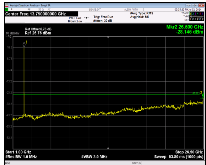
Band7-20MHz-64QAM-21100-1RB#0-Range2:1000~265
