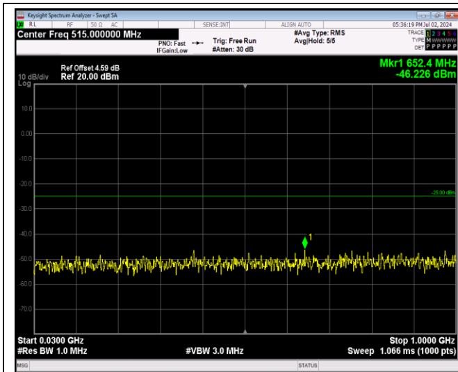
Band7-20MHz-64QAM-21350-1RB#0-Range1:30~100 0MHz
