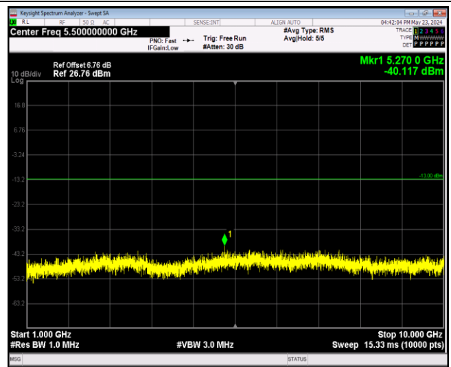
Band5-10MHz-64QAM-20450-1RB#0-Range2:1000~100 00MHz
