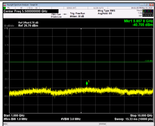
Band5-1.4MHz-QPSK-20525-1RB#0-Range2:1000~1000 OMHz
