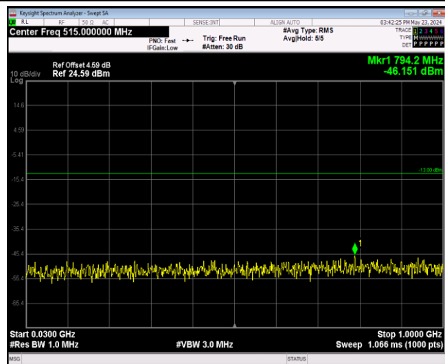
Band2-20MHz-64QAM-19100-1RB#0-Range1:30~100 0MHz
