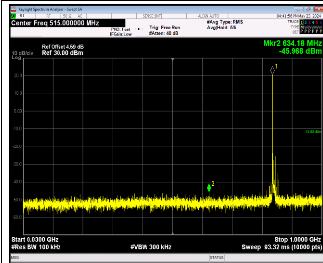
Band5-10MHz-64QAM-20450-1RB#0-Range1:30~100 0MHz
