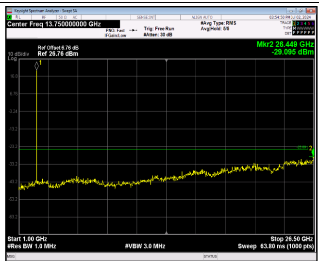
Band7-5MHz-QPSK-21425-1RB#0-Range2:1000~26500 MHz
