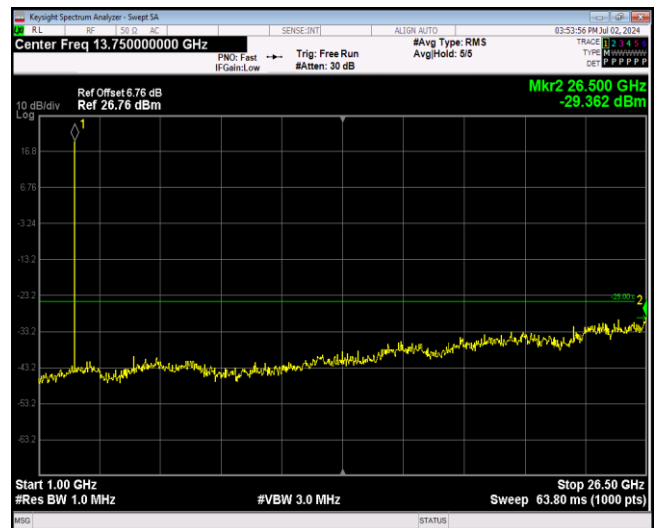
Band7-5MHz-QPSK-21100-1RB#0-Range2:1000~26500 MHz
