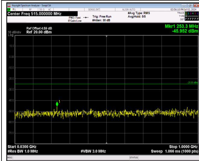
Band7-5MHz-64QAM-21425-1RB#0-Range1:30~1000 MHz
