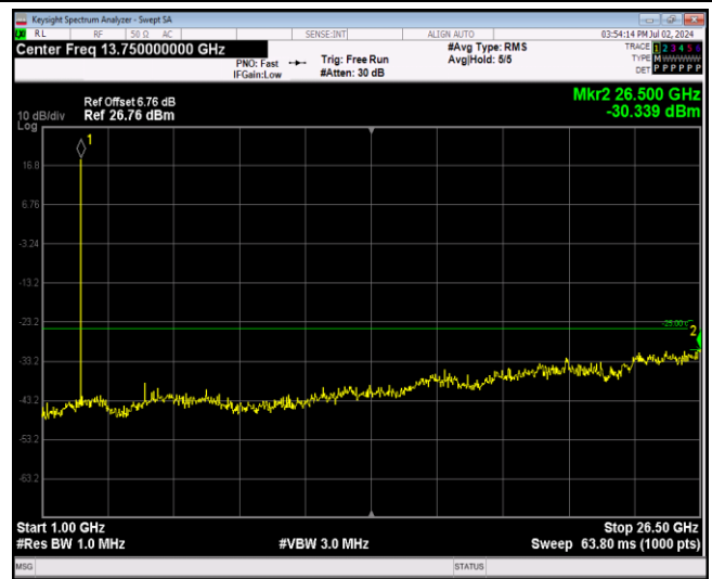
Band7-5MHz-16QAM-20775-1RB#0-Range2:1000~2650 0MHz
