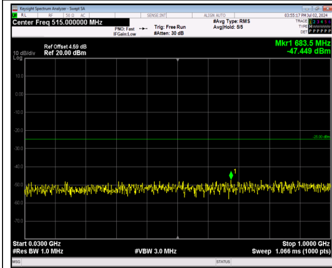
Band7-5MHz-64QAM-21425-1RB#0-Range1:30~1000 MHz
