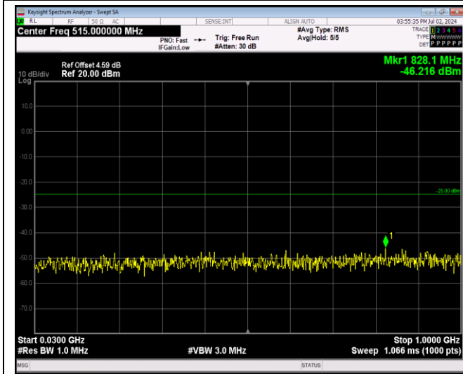
Band7-5MHz-16QAM-20775-1RB#0-Range1:30~1000 MHz
