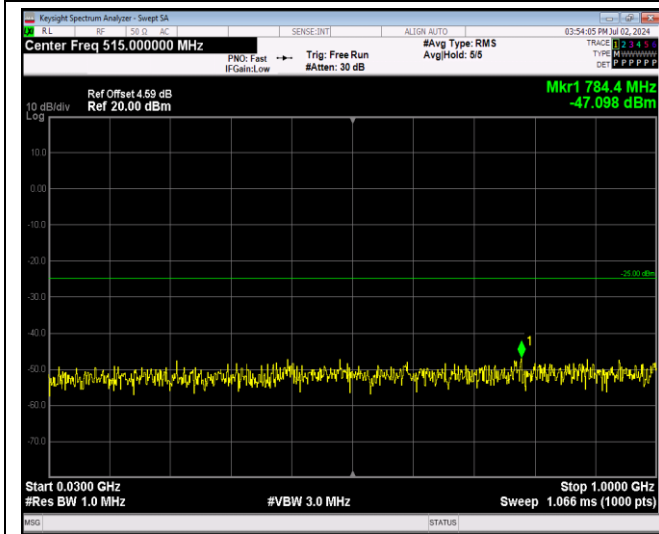
Band7-5MHz-16QAM-20775-1RB#0-Range1:30~1000 MHz
