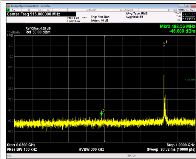
Band5-10MHz-64QAM-20525-1RB#0-Range1:30~100 0MHz
