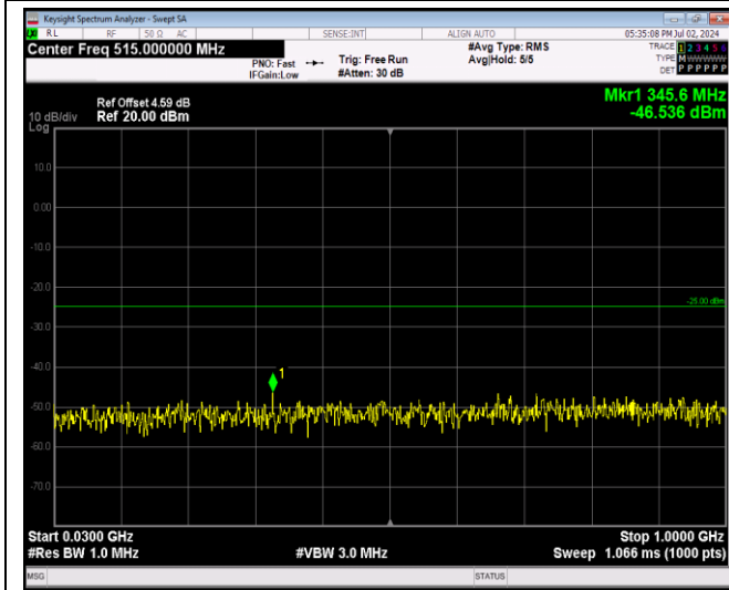
Band7-20MHz-16QAM-21100-1RB#0-Range1:30~100 0MHz
