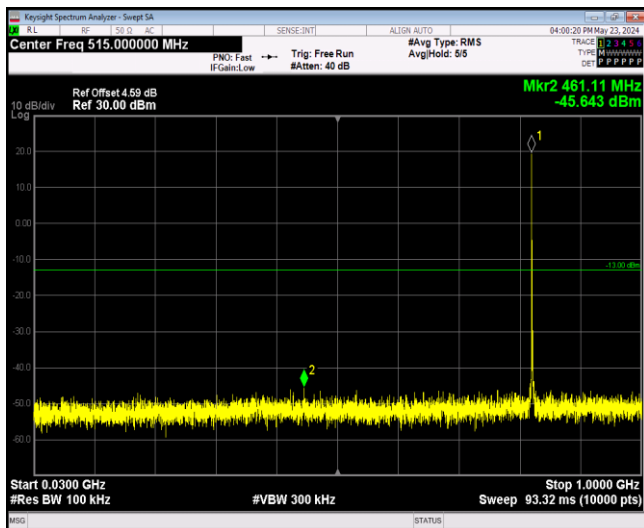
Band5-1.4MHz-16QAM-20525-1RB#0-Range1:30~10
