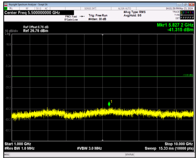
Band5-1.4MHz-16QAM-20407-1RB#0-Range2:1000~100
