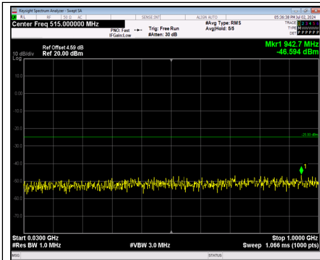
Band7-20MHz-16QAM-20850-1RB#0-Range1:30~100 0MHz
