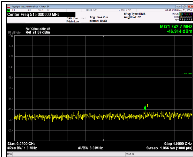
Band5-1.4MHz-QPSK-20407-1RB#0-Range1:30~100 OMHz
