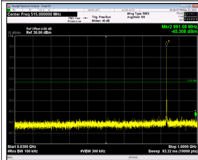
Band5-1.4MHz-QPSK-20525-1RB#0-Range1:30~100 OMHz
