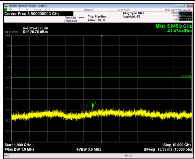
Band5-1.4MHz-16QAM-20643-1RB#0-Range2:1000~10000MHz
