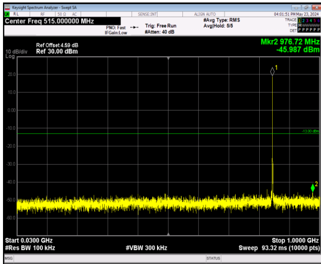
Band5-1.4MHz-16QAM-20407-1RB#0-Range1:30~10
