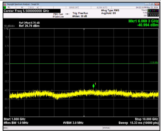
Band5-1.4MHz-64QAM-20407-1RB#0-Range2:1000~10000MHz
