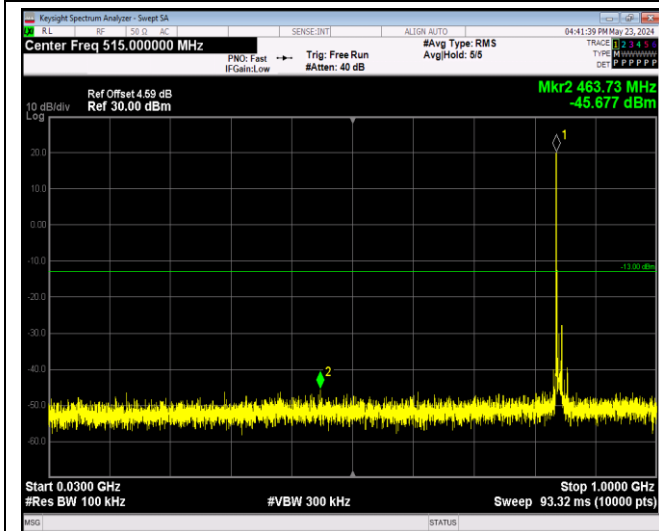
Band5-10MHz-QPSK-20600-1RB#0-Range1:30~1000 MHz
