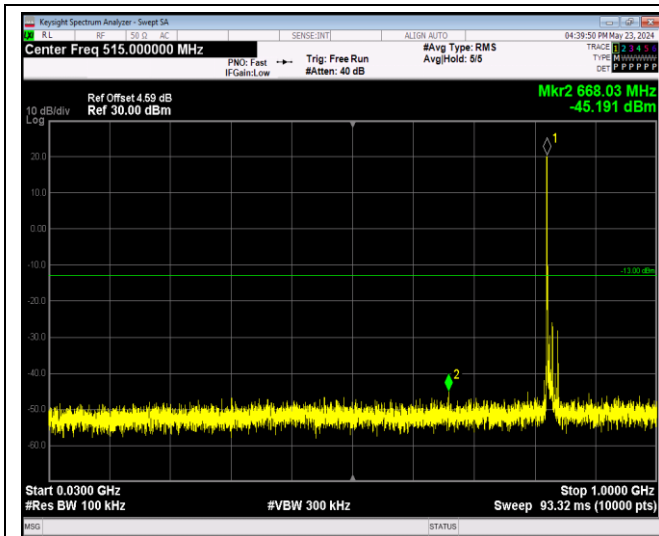
Band5-10MHz-QPSK-20525-1RB#0-Range1:30~1000 MHz
