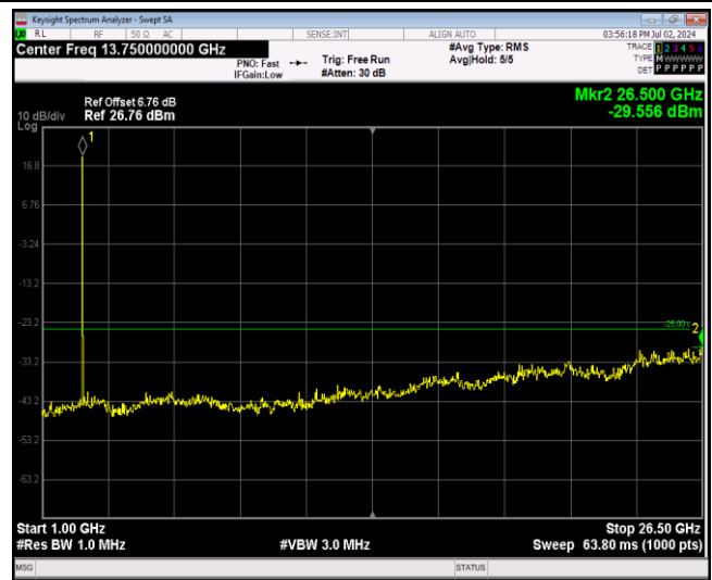
Band7-5MHz-64QAM-21425-1RB#0-Range2:1000~2650 OMHz
