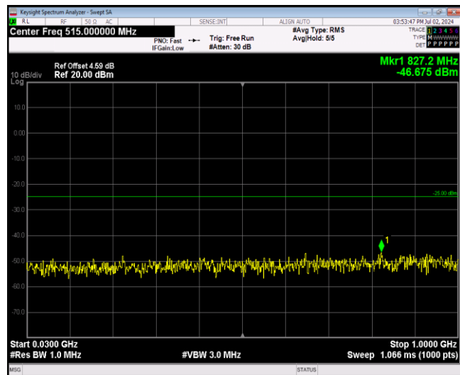
Band7-5MHz-QPSK-21100-1RB#0-Range1:30~1000M Hz
