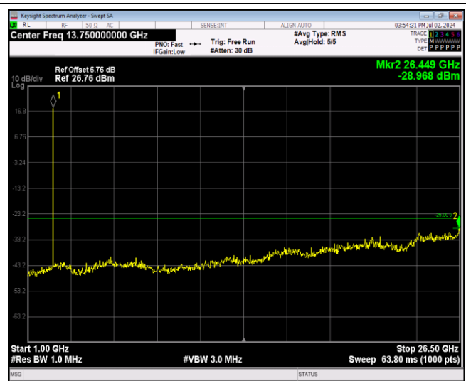
Band7-5MHz-64QAM-21100-1RB#0-Range2:1000~2650 OMHz
