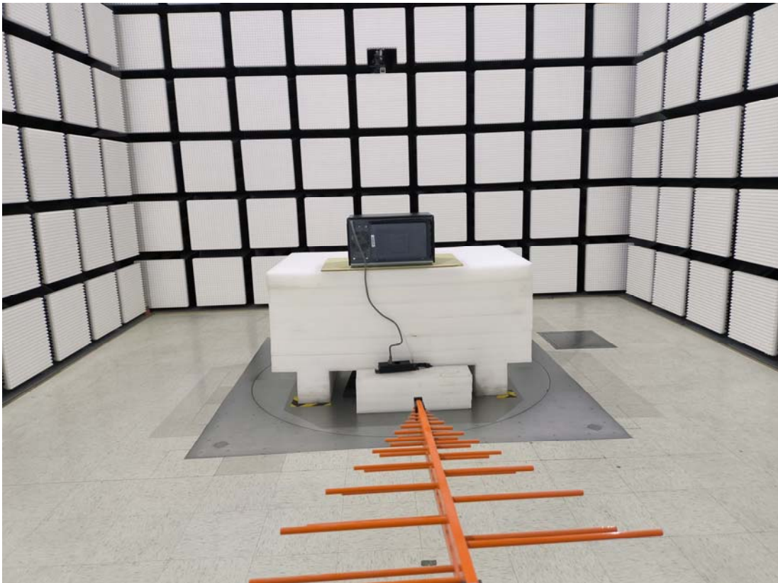
Radiated Emission Below 1GHz Rear View
