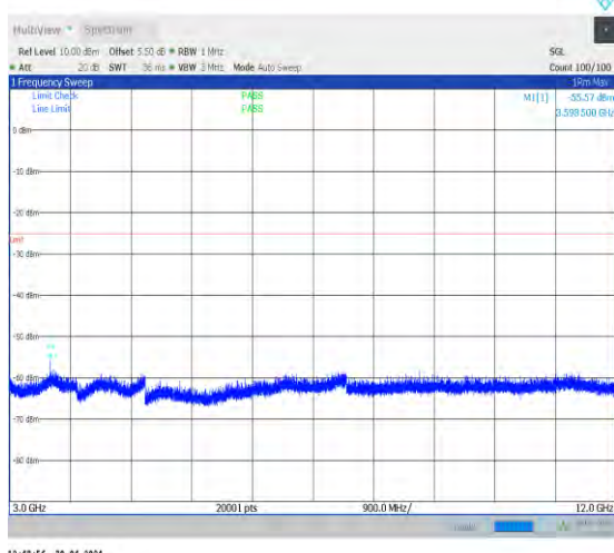
1-N7-PC3-15-40-M-1-DFT-PI2BPSK-Inner_1RB_Lef t-1@1-3000-12000-Ant0-11132.40--55.57--25-PASS
