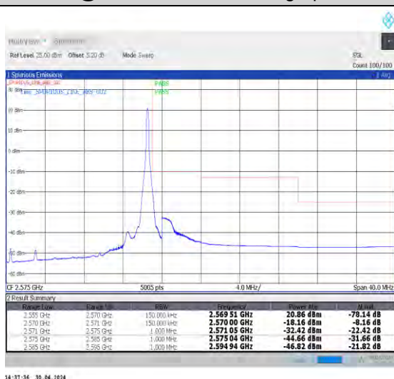
1-N7-PC3-15-15-H-5-CP-QPSK-Edge_1RB_Right-1@78-Ant0-1--PASS-see graph
