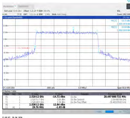
1-N7-PC3-15-30-M-7-CP-16QAM-Outer_Full-160@0 -Ant0-28.5-29.760-≤30-PASS
