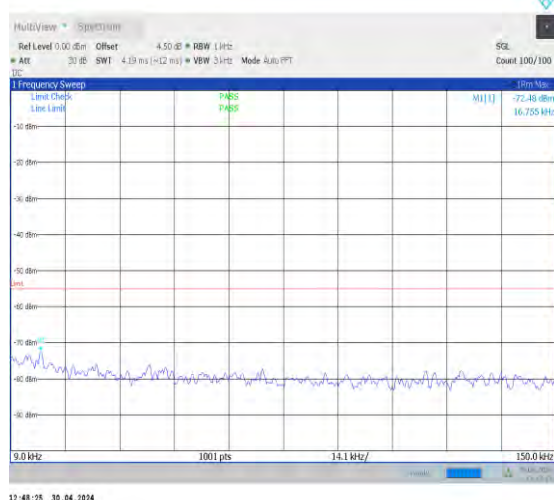
1-N7-PC3-15-40-M-1-DFT-PI2BPSK-Inner_1RB_Left -1@1-0.009-0.15-Ant0-0.14--72.48--55-PASS
