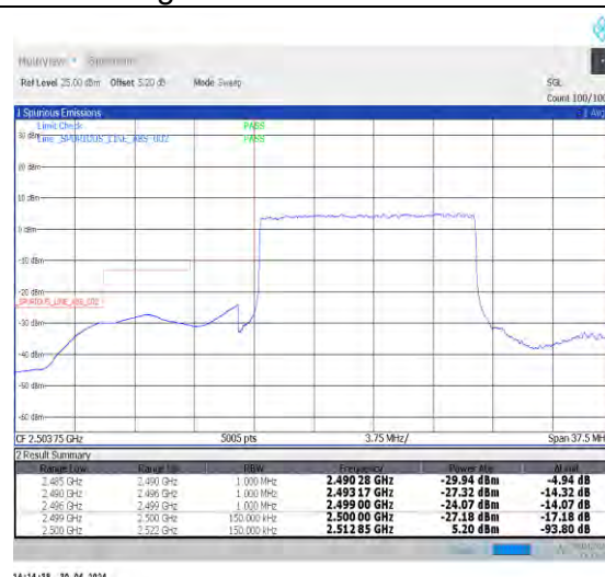
1-N7-PC3-15-15-L-3-DFT-PI2BPSK-Outer_Full-75 @0-Ant0-1--PASS-see graph
