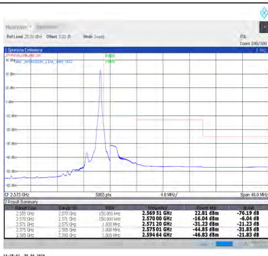
1-N7-PC3-15-15-H-2-DFT-PI2BPSK-Edge_1RB_Right-1@78-Ant0-1--PASS-see graph
