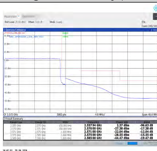
1-N7-PC3-15-15-H-6-CP-QPSK-Outer_Full-79@0-Ant0-1--PASS-see graph
