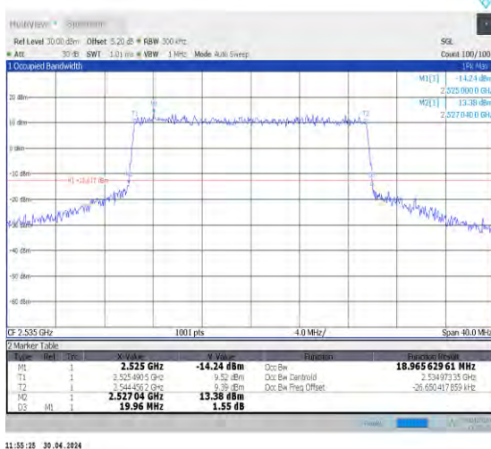
1-N7-PC3-15-20-M-8-CP-64QAM-Outer_Full-106@0-Ant0-18.966-19.960-≤20-PASS
