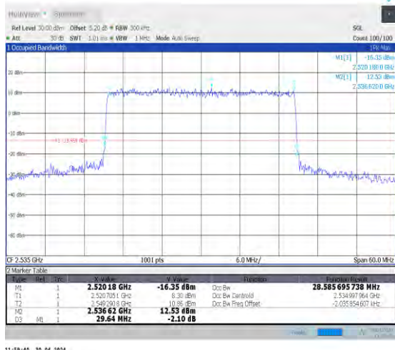
1-N7-PC3-15-30-M-4-DFT-64QAM-Outer_Full-160@ 0-Ant0-28.588-29.640-≤30-PASS
