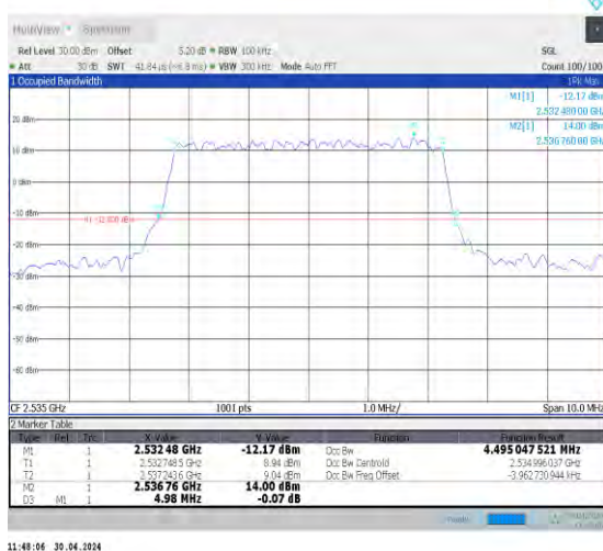
1-N7-PC3-15-5-M-7-CP-16QAM-Outer_Full-25@0-Ant0-4.495-4.980-≤5-PASS
