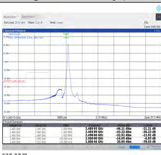
1-N7-PC3-15-15-L-4-CP-QPSK-Edge_1RB_Left-1@0-Ant0-1--PASS-see graph
