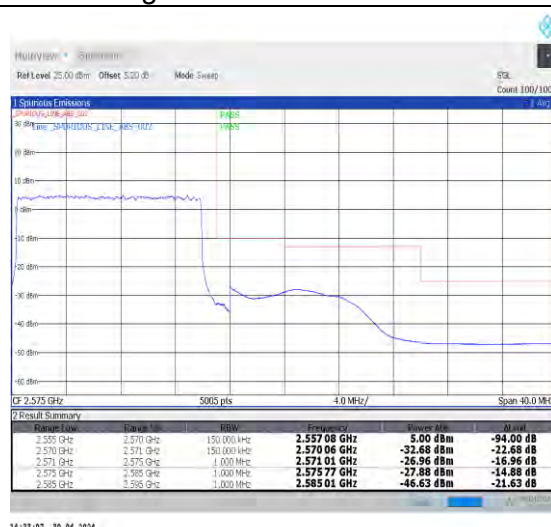
1-N7-PC3-15-15-H-3-DFT-PI2BPSK-Outer_Full-75@0-Ant0-1--PASS-see graph
