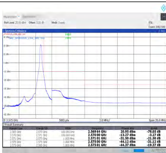
1-N7-PC3-15-5-H-2-DFT-PI2BPSK-Edge_1RB_Right-1 @24-Ant0-1--PASS-see graph
