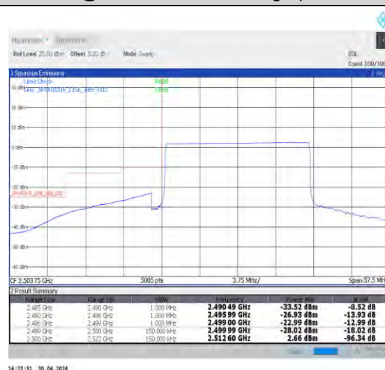
1-N7-PC3-15-15-L-6-CP-QPSK-Outer_Full-79@0-Ant0-1--PASS-see graph
