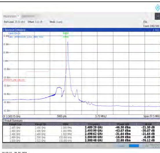
1-N7-PC3-15-15-L-1-DFT-PI2BPSK-Edge_1RB_Left-1 @0-Ant0-1--PASS-see graph
