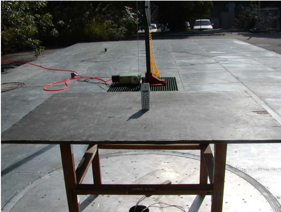
Handset Radiated Emission - Front View (Model: GH3150 & GH3110)
