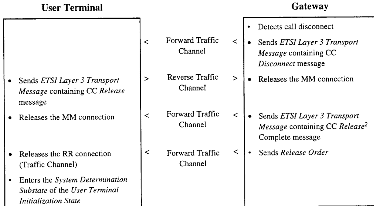
3 Figure 6-11 Simple Call Flow, Gateway Initiated Call Disconnect Example (ETSI Call 4 Control Procedure) 5 (Part 2 of 2) 6
