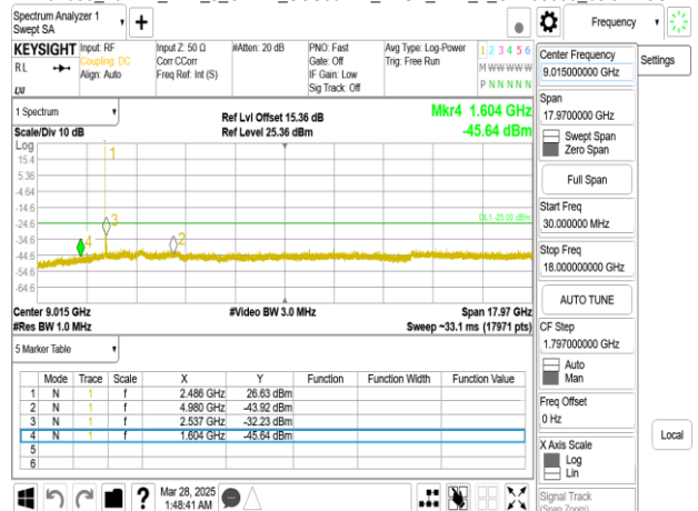
Band53_10MHz_DFT_s_OFDM_SCS30kHz_BPSK_RB1_1_CH498000upper 18G
