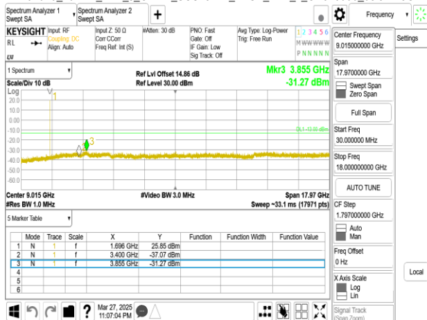
Band70_10MHz_DFT_s_OFDM_SCS15kHz_BPSK_RB1_1_CH340000_below 18G
