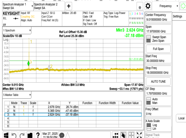
Band41_15MHz_DFT_s_OFDM_SCS30kHz_BPSK_RB1_1_CH536496upper 18G
