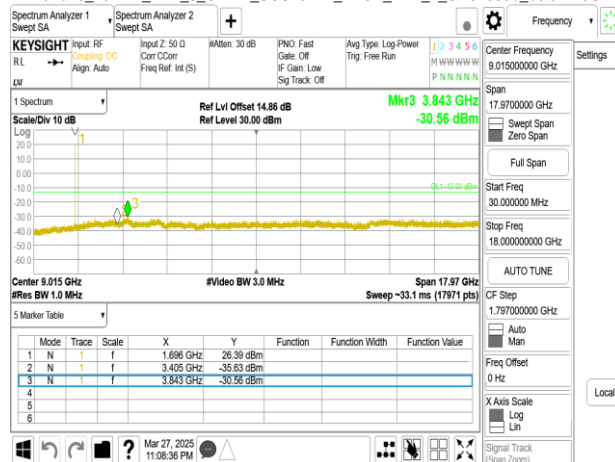
Band70_15MHz_DFT_s_OFDM_SCS15kHz_BPSK_RB1_1_CH340500_below 18G
