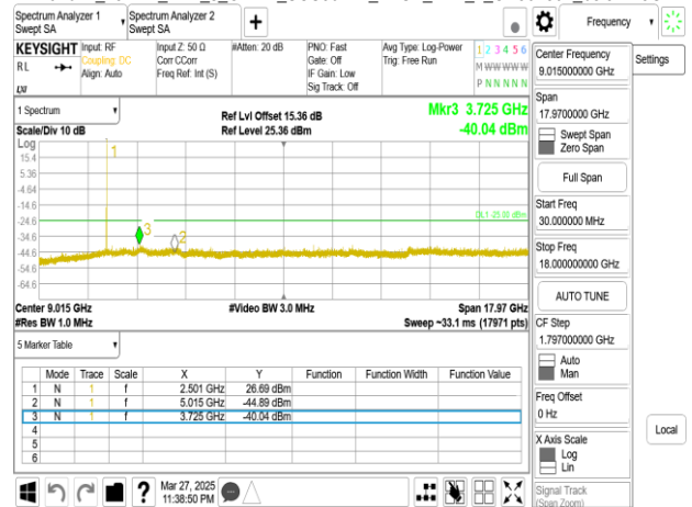
Band41_15MHz_DFT_s_OFDM_SCS30kHz_BPSK_RB1_1_CH501504upper 18G
