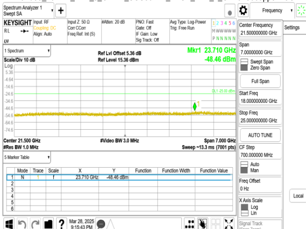
Band53_10MHz_DFT_s_OFDM_SCS30kHz_BPSK_RB1_1_CH497800upper 18G
