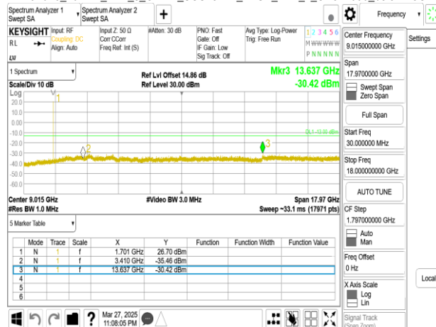
Band70_15MHz_DFT_s_OFDM_SCS15kHz_BPSK_RB1_1_CH340500_below 18G
