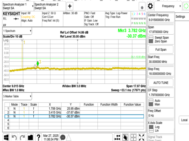
Band70_10MHz_DFT_s_OFDM_SCS15kHz_BPSK_RB1_1_CH340000_below 18G
