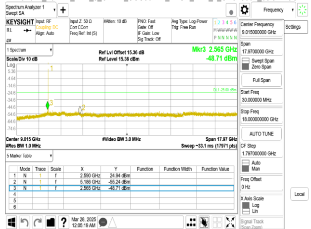
Band41_10MHz_DFT_s_OFDM_SCS30kHz_BPSK_RB1_1_CH518604upper 18G
