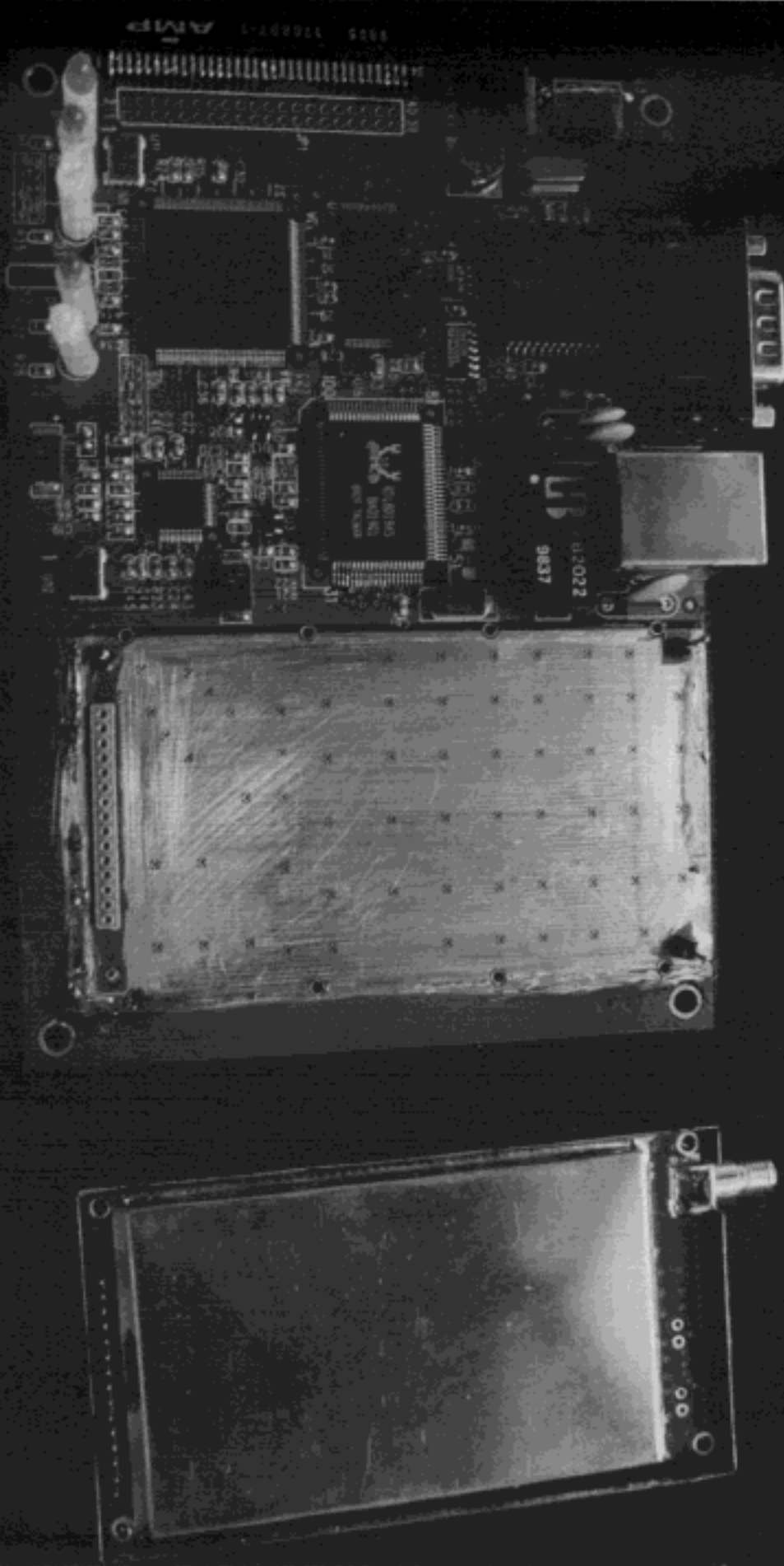
Component View of Main Board
