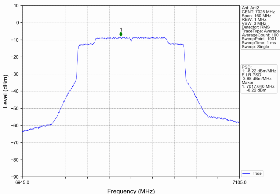
802.11ax(HEW80)_HCH_7025MHz_RU996_Left_MIMO_NTNV
