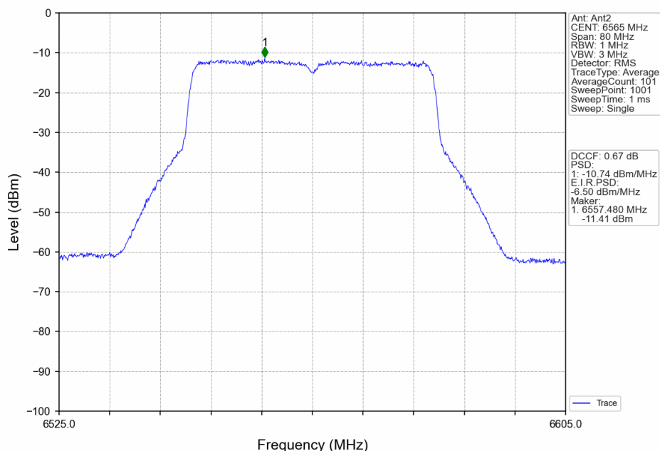
802.11ax(HEW40)_LCH_6565MHz_RU484_Left_MIMO_NTNV
