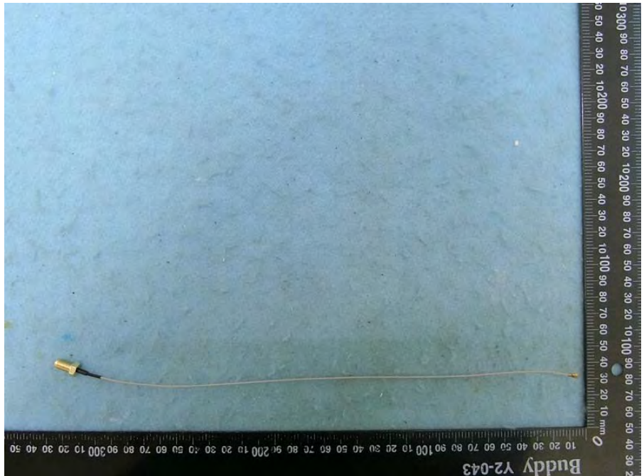
300mm antenna cable (Only for set 9 antenna use) P/N: 510411-5210-24C
