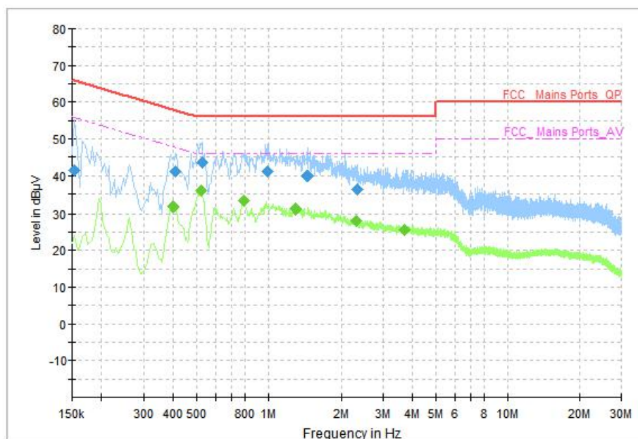
Fig.70 AC Power line Conducted Emission (Idle, AE2, 120V)
