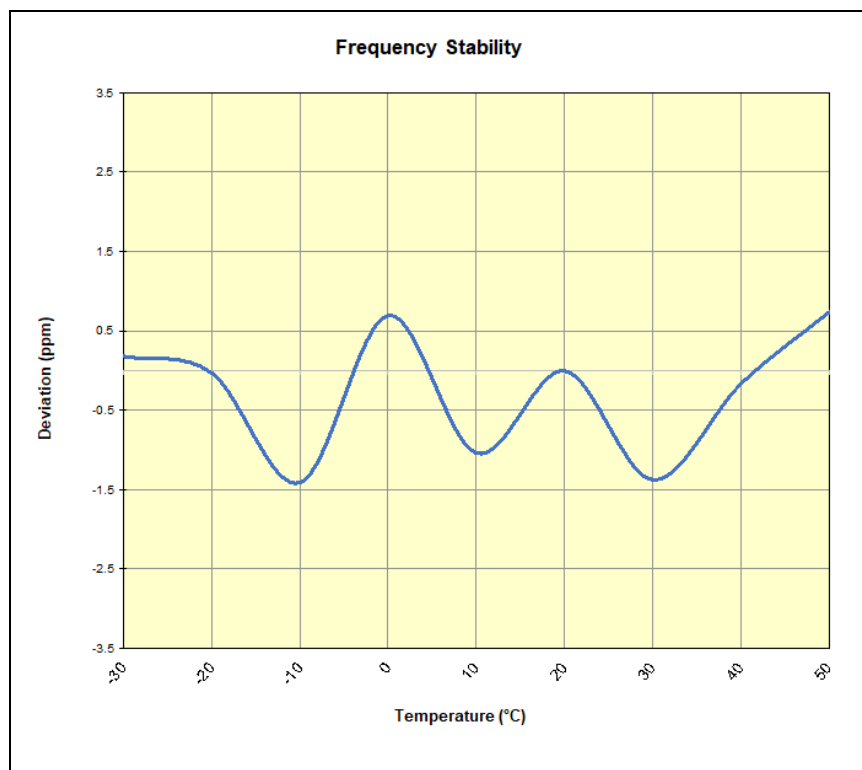
Plot 7-21. LTE Band 14 Frequency Stability Chart
