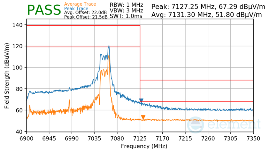
Plot 7-1808. SDM Radiated Upper Band Edge (Peak & Average – UNII Band 8 – RU26)
