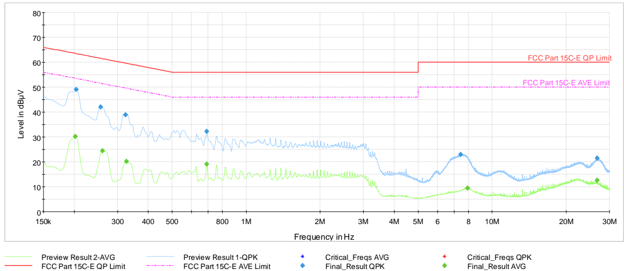
Plot 7-1817. AC Line Conducted Plot with SDM Primary 11ax UNII Band 5 – RU26 – Ch.1 (L1) with Laptop
