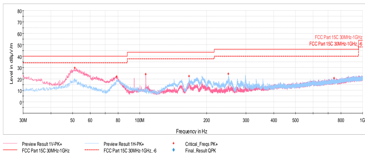
Plot 7-1814. Radiated Spurious Emissions below 1GHz SDM Primary (802.11ax – Ch.1 – RU242) with AC/DC Adapter
