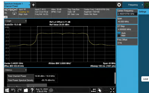
11AX20SISO-Ant1-2462-PASS
